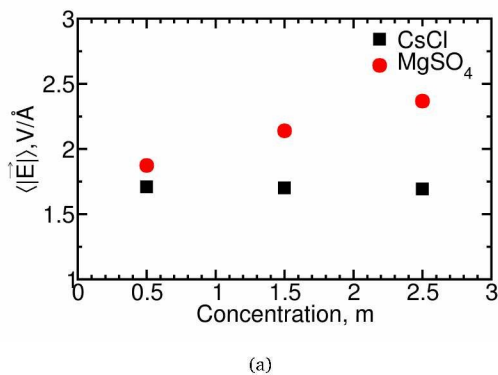
Fig. 10 Average electric field magnitude, \langle |\vec{E}| \rangle , for \text{CsCl} and \text{MgSO}_4 solutions.
