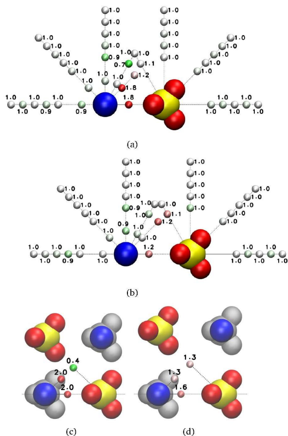
Fig. 8 Cooperativity factor for \text{MgSO}_4 (a,b) ion pairs and (c,d) ion clusters. The anion-cation distance is (a,c) 5 Å, corresponding to the \text{SIP}_i configuration, and (b,d) 5.6 Å, corresponding to the \text{SIP}_o configuration.
