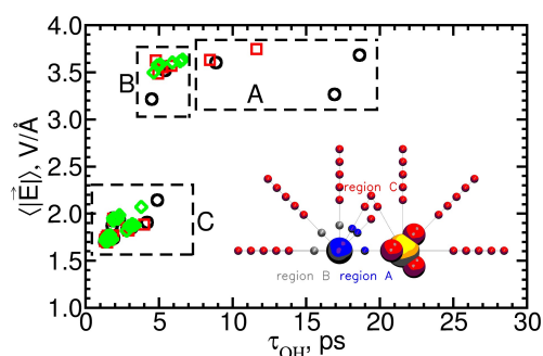
Fig. 11 Electric field magnitude, \langle |\vec{E}| \rangle , as a function of the reorientation time of water OH groups belonging to different water subpopulations around \text{MgSO}_4 SIP i , SIP o , and 2SIP with freely rotating ions. The different data points are for water subpopulations in regions A, B and C around the ion pairs, as shown in the inset.
