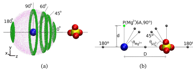
Fig. 5 (a) Example water subpopulations (small green dots) near an anion-cation pair. The image shows only water subpopulations centered on magnesium, but similar subpopulations centered on sulfate are also investigated. The same water subpopulations are investigated near ion clusters. (b) Water subpopulations near ions are represented by the grey spheres and referred to in the text by the reference ion, distance d and angle \theta associated with them, as exemplified for point P (green).
