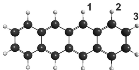
Fig. 1: Illustration of tetracene or benz[ b ]anthracene. Labels 1, 2, and 3 denote the three available deprotonation sites to produce the C_{18}H_{11}^- species. Position 1 is the predominant deprotonation site in the present experiments. Key: charcoal – carbon; white – hydrogen.
