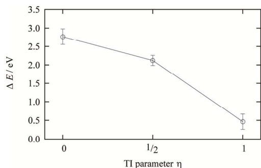
Figure 5 The ensemble average of the ionization energy of the \Delta E_0 for each \eta state of I^{0-} .
