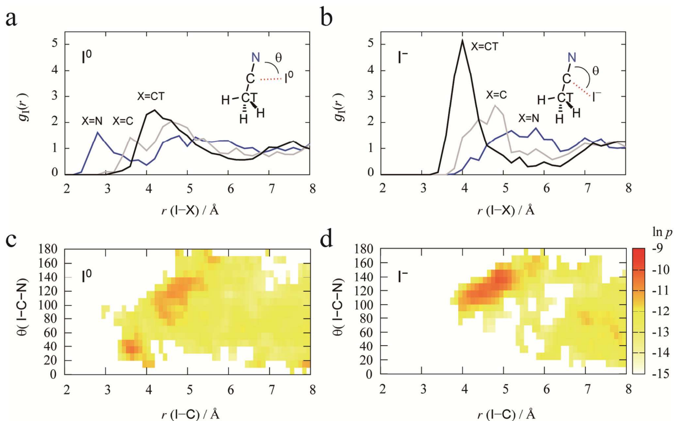
Figure 4 (a), (b): Radial distribution functions g_I(r) calculated from DFT–MD simulations for I^0 (a) and I^- (b) in 44 AN molecules. Blue, gray, and black lines denote the RDFs for nitrogen (N), carbon (C), and terminal methyl carbon (CT) of AN, respectively. (c), (d): The two-dimensional distributions along r(I-C) and \theta(I-C-N) for I^0 (c) and I^- (d) in the 44 AN molecule system. The carbon is the one colored gray in the RDFs.
