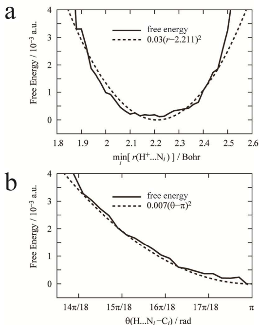
Figure 2 Calculated free energy profiles along r(\text{H}^+-\text{N}_i) (a) and \theta(\text{H}^+-\text{N}_i-\text{C}_i) (b), where \text{N}_i is the nitrogen of the AN molecule
