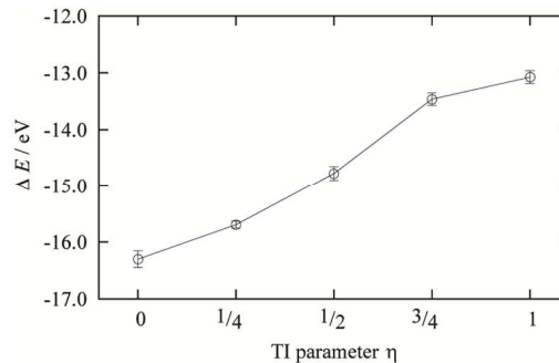
Figure 3 The ensemble average of the ionization energy of \Delta E_0 for each \eta state.
