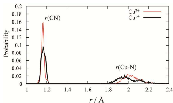
Figure 7 The distribution of the distance between carbon and nitrogen and that between the copper ion and nitrogen of directly connected AN molecules with a copper ion.
