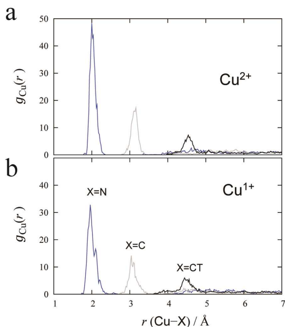
Figure 6 RDFs calculated from (a) \text{Cu}^{2+} and (b) \text{Cu}^{1+} in 44 AN molecules. Blue, gray, and black lines denote the RDF for nitrogen, carbon, and carbon in the methyl group of AN, respectively.
