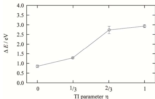
Figure 8 The ensemble average of the ionization energy of the \Delta E_0 for each \eta state of \text{Cu}^{2+} .
