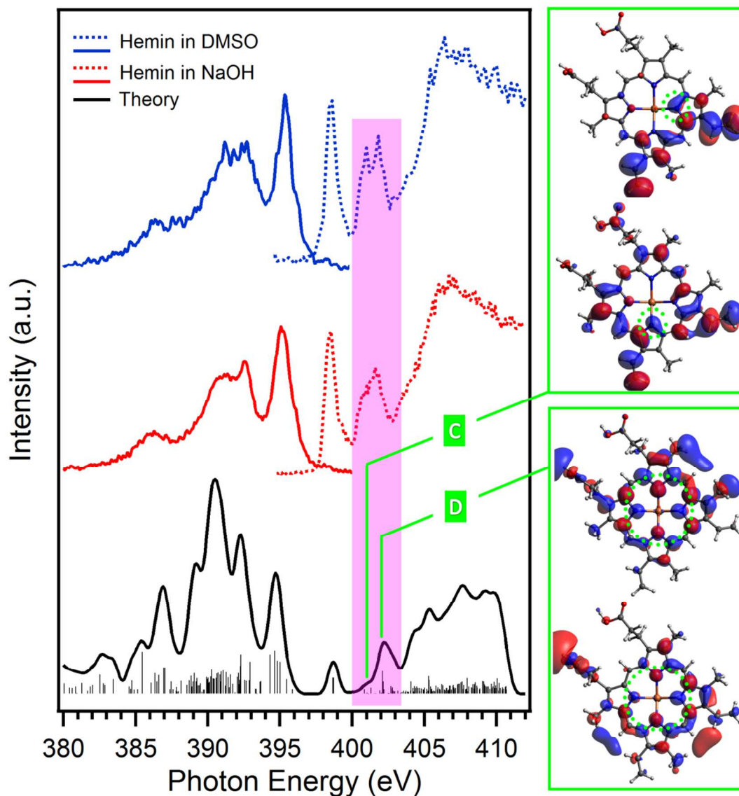
Figure 4. Off-resonant XE spectra (solid blue and red traces) at the excitation energies of 420 eV for the hemin dissolved in DMSO and NaOH aqueous solution, respectively, combined with their respective PFY-XA spectra (dashed blue and red traces). The experimental spectra are identical to the corresponding spectra in Figure 2. The theoretical DFT calculations and individual MOs weighted by N contributions are shown at the bottom as black trace and vertical bars, respectively. The characteristic features C and D identified in Figure 3 are assigned to certain calculated MOs with visualized orbitals presented on the right side of the figure. The orbitals localized at the N sites are highlighted with dotted green circles.
