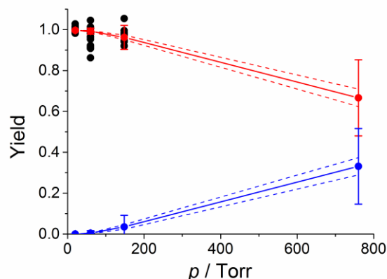
Fig. 4 Experimental \text{HO}_2 yield (black circles) and calculated \text{HO}_2 and \text{HOCH}_2\text{CH}(\text{O}_2)\text{NH}_2 yields (red circles and line and blue circles and line, respectively) using MESMER for \text{HOCH}_2\text{CHNH}_2 + \text{O}_2 reaction at 298 K and various pressures of nitrogen bath gas. The error bars were calculated by varying the energy barrier for the formation of \text{HO}_2 by \pm 4 \text{ kJ mol}^{-1} . The dash lines show the propagation of the statistical errors obtained by fitting the experimental points.
