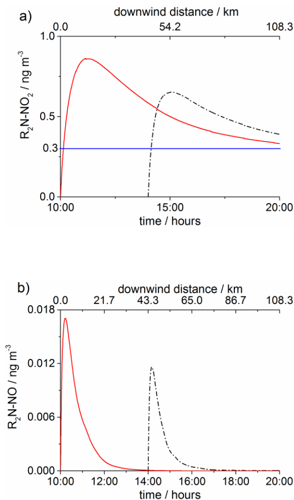
Fig. 7 Gas-phase concentrations of (a) \text{R}_2\text{N-NO}_2 and (b) \text{R}_2\text{N-NO} in the PCCC plume as a function of time (bottom axis) in the clear day scenario. Emission time: 10:00 (red solid line) and 14:00 (black dash dot line). The top axis shows the downwind distance from the source for the emission at 10:00. The horizontal blue line in (a) shows the safety limit of 0.3 \text{ ng m}^{-3} for [\text{R}_2\text{N-NO}_2] + [\text{R}_2\text{N-NO}] established by the NIPH. 21
