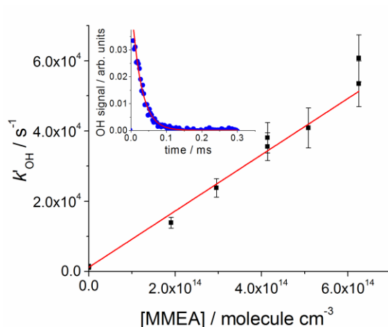
Fig. 1 Bimolecular plot for MMEA, (8.01 \pm 0.92) \times 10^{-11} \text{ cm}^3 \text{ molecule}^{-1} \text{ s}^{-1} , at 298 K and a total pressure of 17 Torr of \text{N}_2 . The error bars are at \sigma level. A typical OH fluorescence decay trace and fit to eqn E1 is shown in the inset.
