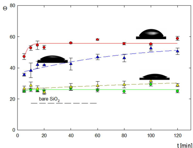
Figure 4. Contact angle changes in time measured for various HEWL concentrations at pH4 and pH7. Green circles: HEWL concentration 5ppm and pH 4; red circles: HEWL concentration 5ppm, pH 7; yellow triangles: HEWL concentration 0.5ppm and pH 4; navy triangles HEWL concentration 0.5ppm and pH7. Insets show the
