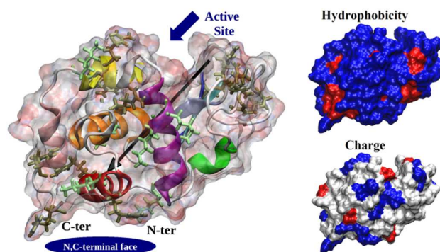
Figure 1. HEWL structure. Protein surface is shown as a ghost surface colored by partial charge with protein secondary structure elements indicated as a cartoon and colored as follows: red, \alpha -helix A; orange, \alpha -helix B; purple, \alpha -helix C; yellow, \alpha -helix D; pink, C-terminal \alpha -helix 3_{10} from domain \alpha ; green middle \alpha -helix 3_{10} from domain \beta ; blue, sheet \beta_1 ; cyan, sheet \beta_2 ; gray, sheet \beta_3 ; white, other structures including loops, turns and \beta -bridges. Arg and Lys residues are shown as licorice and colored in tan and light green, respectively. The black needle indicates the protein dipole moment. Protein termini, N,C-terminal face and active site location are shown by navy objects and annotated. Figures on the right show
