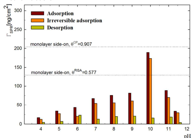
Figure 3. Surface mass density of HEWL (in ng/cm 2 ) adsorbed at the silica surface obtained from MP-SPR in the pH range 4 to 12. The mass density of close-packed (CP) and Random Sequential Adsorption (RSA) monolayers of protein adsorbed in the side-on orientation are shown by dotted lines.
