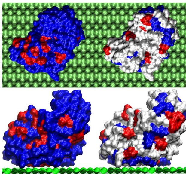
Figure 2. A typical final HEWL adsorption stage. Both SiO 2 and HEWL are shown using a surface representation. SiO 2 is shown in green while the protein is colored by hydrophobicity index (left) and by total residue charge (right) using the colour scheme of Fig. 1. The top and bottom figures show the plan and the side view, respectively. For clarity water molecules are not shown.
