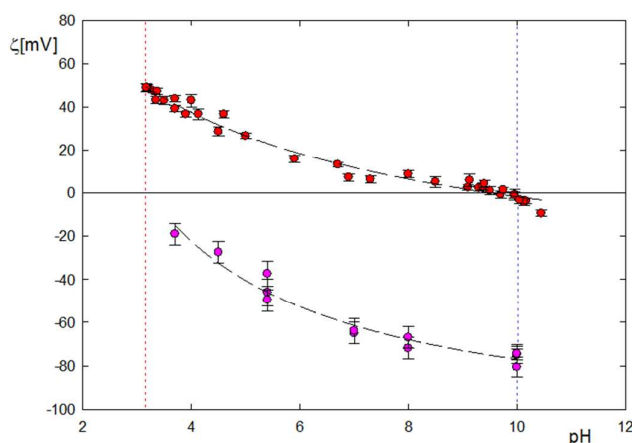
Figure 5. Zeta potential (in mV) measured for HEWL (red) and bare SiO 2 surface (purple) at pH range 2 to 12 in ionic strength 0.01M of NaCl. The red and blue vertical dotted lines point the isoelectric point of SiO 2 (at pH 3.0) and HEWL (at pH 10.0), respectively.
