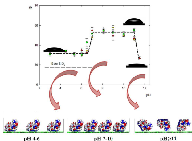
Figure 6. Contact angle measured for bare and HEWL-modified SiO 2 surface at pH range 3 to 11. The insets into the plot shows the water drop shape created on the HEWL-modified SiO 2 surface. Green, yellow and red points in the plot indicate the contact angle obtained for protein concentration 1000ppm, 10ppm and 5ppm, respectively. The figures at the bottom of the picture shows the schematic HEWL orientation on the SiO 2 surface at low (left), intermediate (middle) and high (right) pH.
