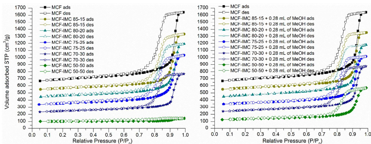
Fig. 3. Nitrogen adsorption-desorption isotherms of MCF host loaded with different ratios of IMC using the melting method (left) and MCF host loaded with different ratios of IMC using the melting method and subsequently treated with MeOH (right). The isotherms are offset by 100 \text{ cm}^3/\text{g} .
