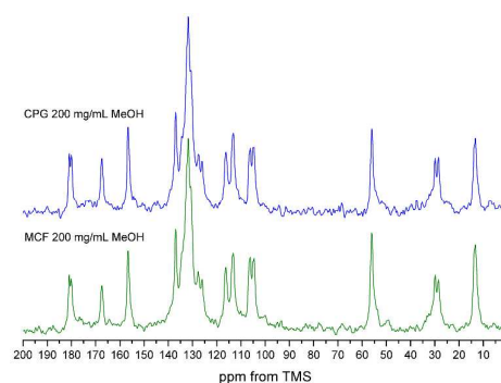
Fig. 12 ^1\text{H} - ^{13}\text{C} CP/MAS solid-state NMR spectra of CPG and MCF hosts loaded using IW method at indomethacin concentration in methanol of 200 mg/mL.
