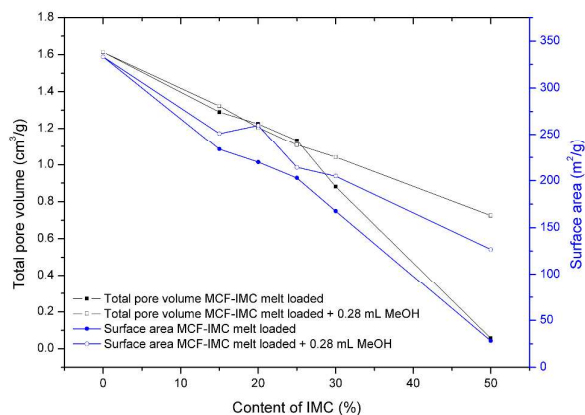
Fig. 4 Total pore volume and BET surface area of MCF-IMC melt loaded samples before and after addition of the solvent. The total amount of IMC within the materials was determined using TG analysis.
