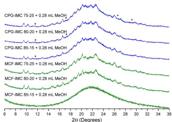
Fig. 8 PXRD patterns of MCF and CPG hosts loaded with molten indomethacin after treatment with methanol (peaks showing the presence of \gamma -IMC are labelled with asterisks).
