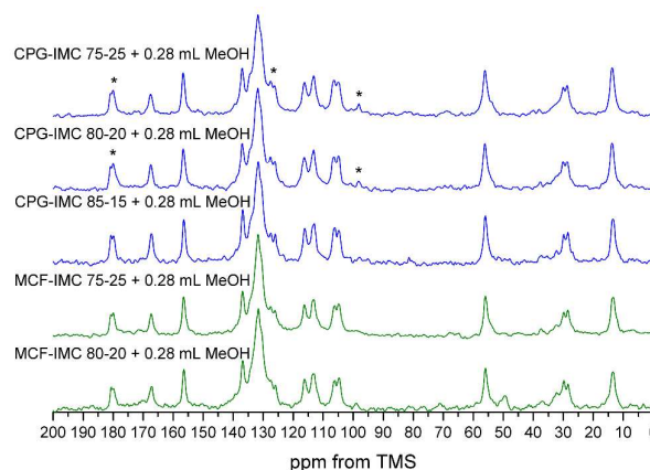
Fig. 9 1 H- 13 C CP/MAS solid-state NMR spectra of MCF and CPG hosts loaded with molten IMC at different concentration subsequently treated with methanol (peaks assigned to \gamma -IMC are labelled with asterisks).
