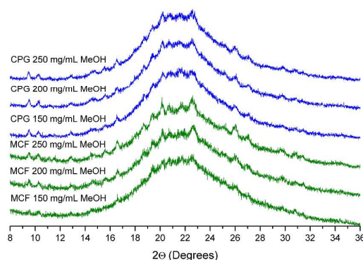
Fig. 10 PXRD patterns of CPG host and MCF materials loaded with IMC using IW method with 0.6 mL/g of the solvent for CPG and 0.8 mL/g of the solvent for MCF.
