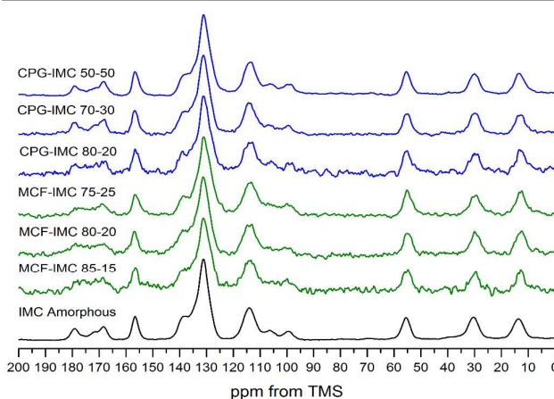
Fig. 5 1 H- 13 C CP MAS NMR spectra of MCF and CPG hosts loaded with molten IMC at different concentrations.
