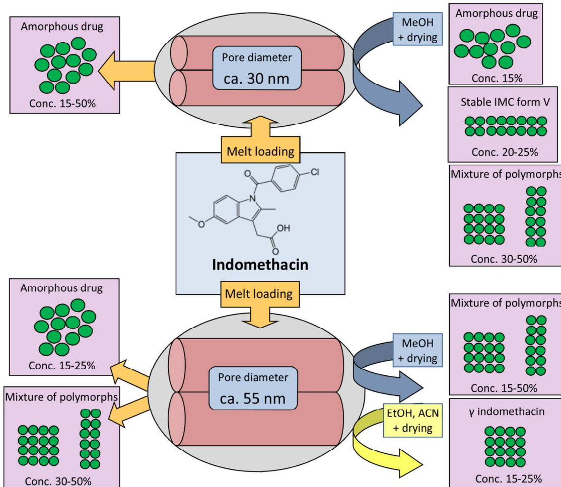
Scheme 1 Summary of possible amorphous to crystalline transformations of melt loaded indomethacin under confinement of MCF and CPG hosts.
