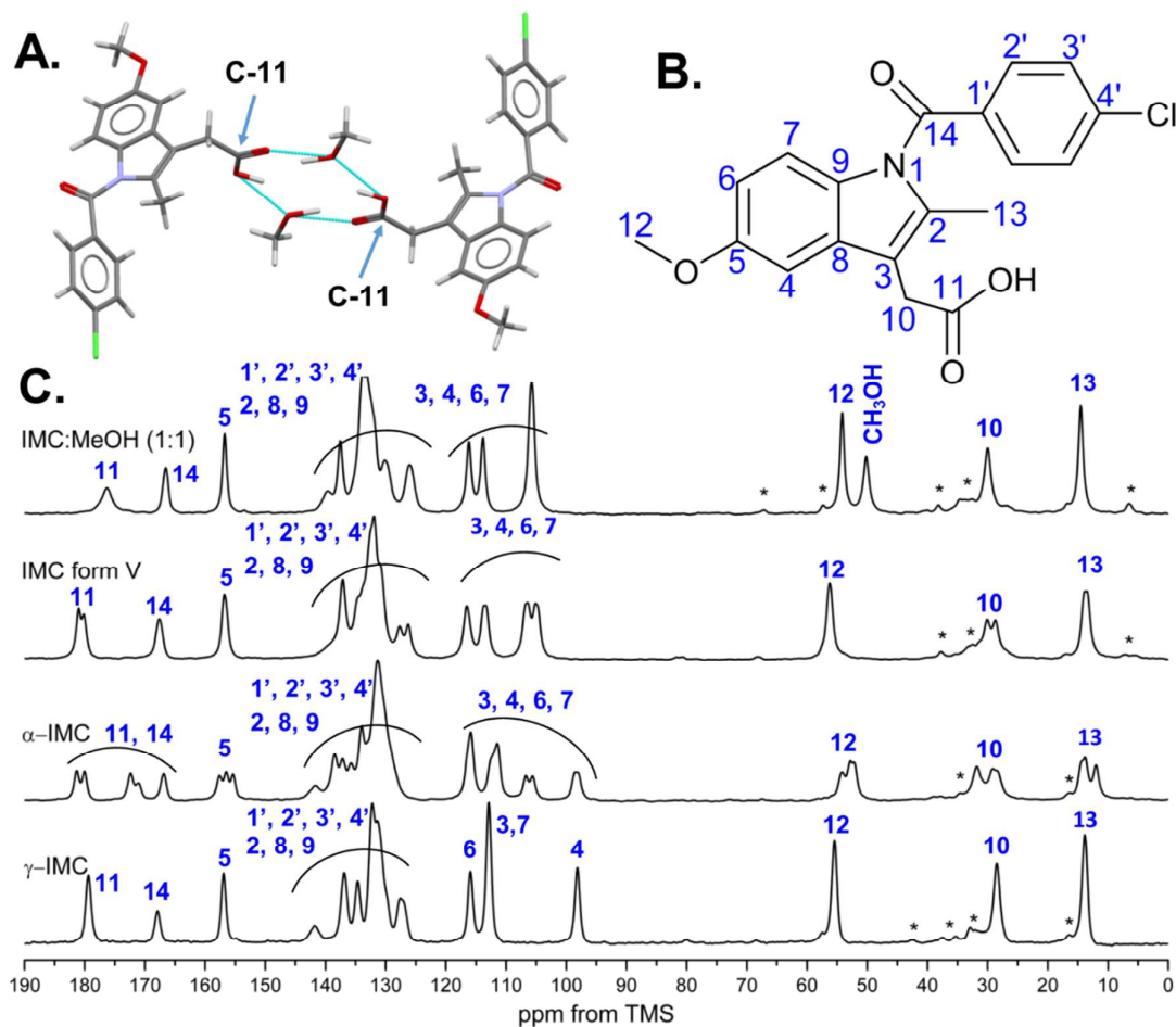
Fig. 2. A. Hydrogen bonded R_4(12) ring motif formed between IMC and methanol extracted from the IMC methanol solvate crystal structure (BANMUZ); B. Molecular diagram of IMC with labelled carbons; C. ^1\text{H} - ^{13}\text{C} CP/MAS NMR spectra of IMC polymorphs and methanol solvate (spinning sidebands are labelled with asterisks).
