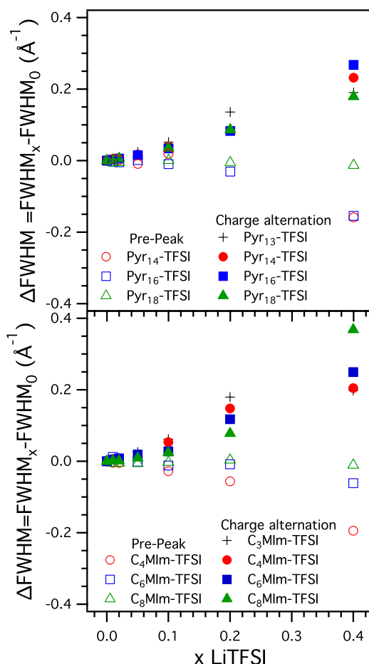
Figure 5. FWHM differences, see text, as a function of Li-salt doping x and alkyl chain length n for \text{Pyr}_{1n} -TFSI (top) and \text{C}_n\text{MIm} -TFSI (bottom).
