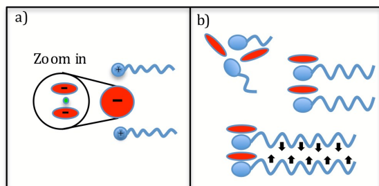
Figure 3. a) Schematic of \text{Li}[\text{TFSI}]_2 complexes where the cluster can effectively act as a single negative charge (lithium ion in green). b) Schematic of the effect of the alkyl chain length on the distance between the polar groups.
