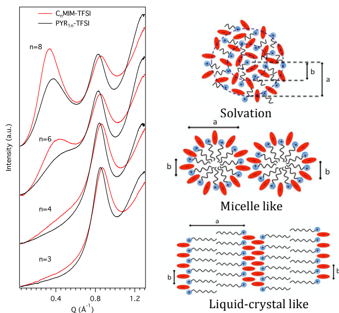
Figure 1. Left: SAXS patterns of the two ILs families \text{Pyr}_{1n}\text{-TFSI} and \text{C}_n\text{MIm-TFSI} . Right: Schematic representation of different models to interpret the origin of the peaks in the SAXS diffraction patterns of ionic liquids, where (a) is the pre-peak and (b) the charge alternation peak.
