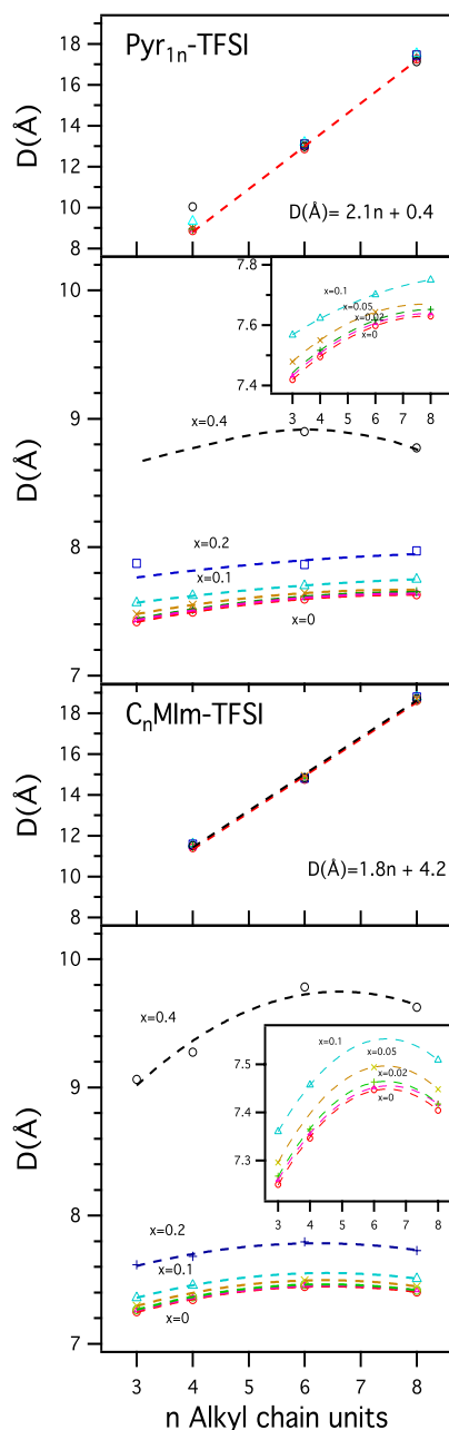
Figure 4. Characteristic distances of structural heterogeneities related to the pre-peak (top panels) and the charge alternation peak (bottom panels) in the static structure factor as a function of alkyl chain length n and Li-salt concentration for Pyr 1n -TFSI (top) and C n MIm-TFSI (bottom). Insets show a close up of the distances related to the charge alternation peak in the low salt concentration region.
