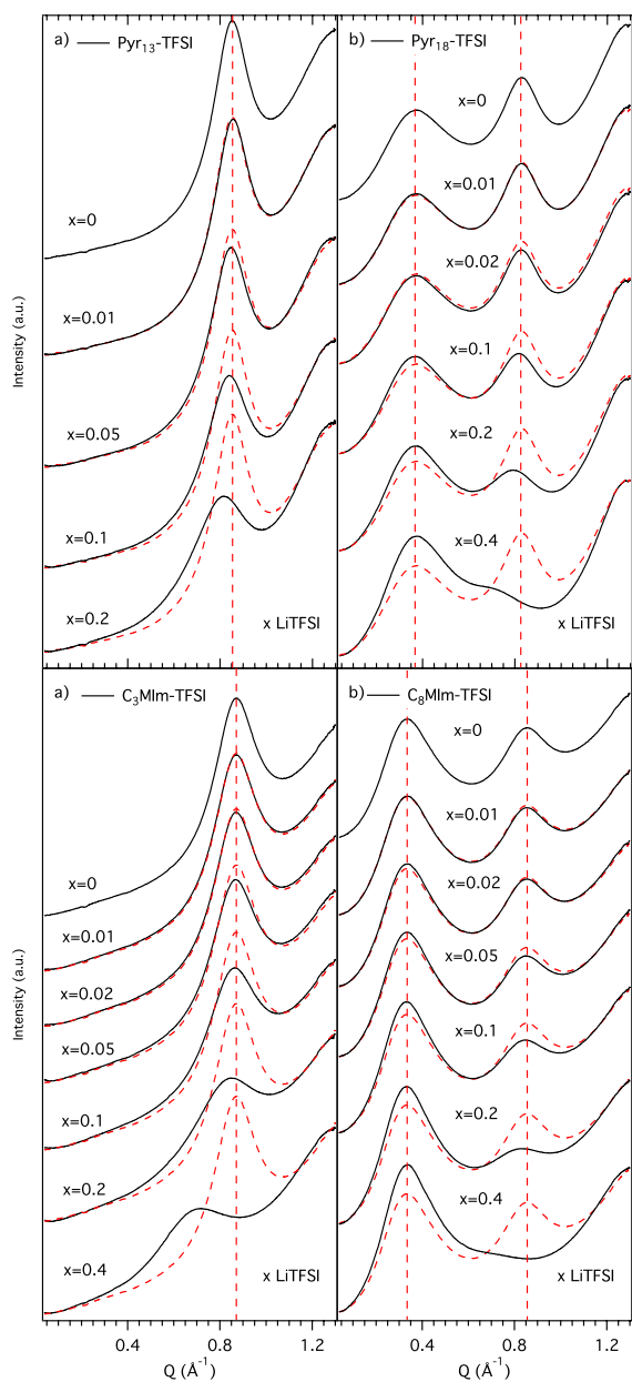
Figure 2. SAXS patterns of the two ILs families \text{Pyr}_{1n}\text{-TFSI} (top) and \text{C}_n\text{MIm-TFSI} (bottom), a) as a function of Li-salt doping for n=3 , and b) as a function of Li-salt doping for n=8 . Dashed curves represent the undoped ILs ( x=0 ), while the dashed vertical lines show the peak positions of the undoped ILs.
