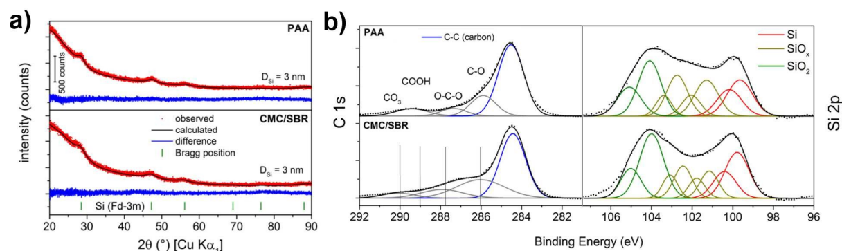
Figure 1. a) XRD pattern and b) XP spectra of the pristine silicon electrodes prepared with PAA and CMC/SBR as binder.
