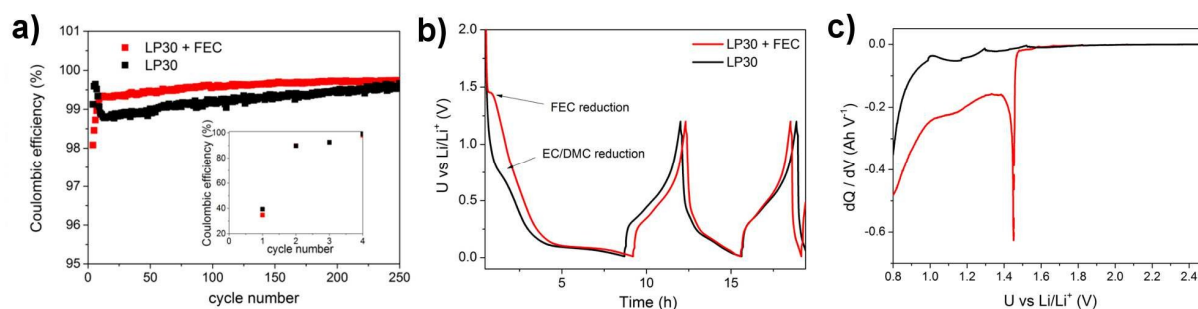
Figure 3. Electrochemical characterization of the silicon electrode with CMC/SBR as binder in dependency of FEC addition. a) Coulombic efficiency of the galvanostatic cycling between 0.01–1.2V vs. Li/Li + at 2.5 A/g (the first two cycles at 0.5 A/g), b) the first two discharge/charge curves and c) the differential capacity of the first discharge.
