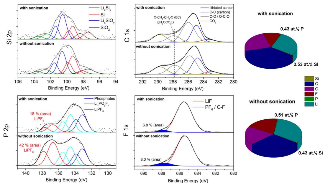
Figure 4. XP spectra (left) and concentration (right) of the silicon electrode with PAA as binder after 400 times cycling in LP30 with FEC addition in dependency of the washing procedure (washed 3 times in DMC with a final sonication process or 3 times in DMC without sonication).
