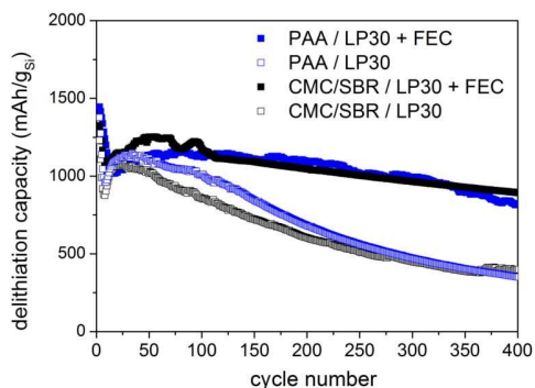
Figure 2. Galvanostatic cycling between 0.01–1.2V vs. Li/Li + at 2.5 A/g (two pre-cycles at 0.5 A/g) of the silicon electrode in dependency of binder and FEC addition.
