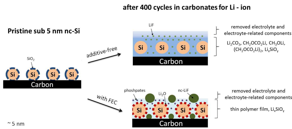
Figure 9. Simplified schematic illustration of the silicon-carbon nanostructure after long-term cycling in dependency of FEC addition.
