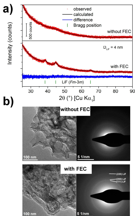
Figure 5. a) XRD pattern and b) TEM bright-field images (left) with selected area electron diffraction (SAED) (right) of the cycled silicon electrodes with CMC/SBR in dependency of FEC addition.
