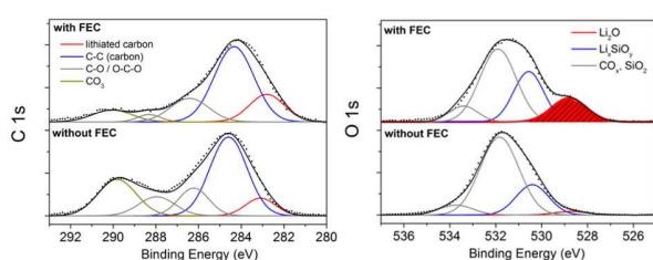
Figure 7. XP spectra of the silicon electrodes with CMC/SBR as binder cycled 400 times in dependency of FEC addition after \text{Ar}^+ ion sputtering ( \sim 15 nm surface removal).
