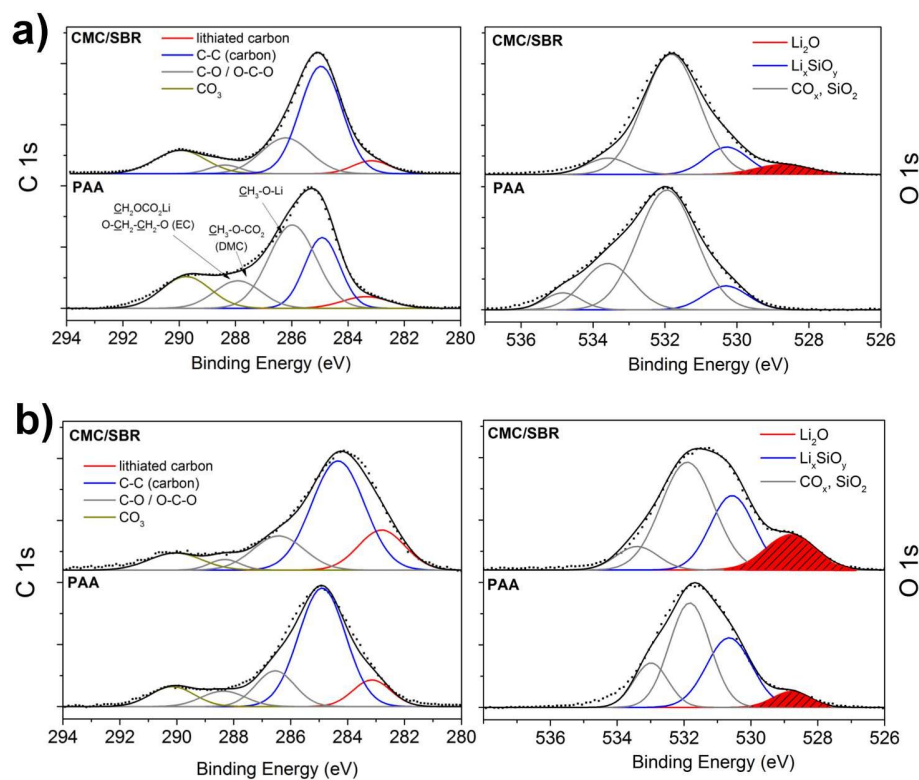
Figure 8. XPS spectra of the silicon electrodes cycled 400 times in LP30 with FEC in dependency of the binder a) no sputtering and b) after sputtering with an Ar + beam (~ 15 nm surface removal).
