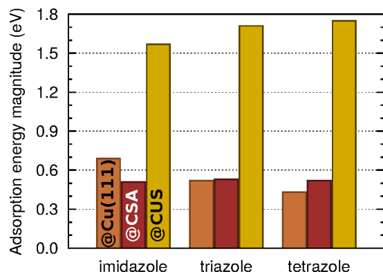
Fig. 3 Adsorption energies of imidazole, triazole, and tetrazole on \text{Cu}(111) and at the CSA and CUS sites of \text{Cu}_2\text{O} . The values for \text{Cu}(111) are taken from ref. 6.
