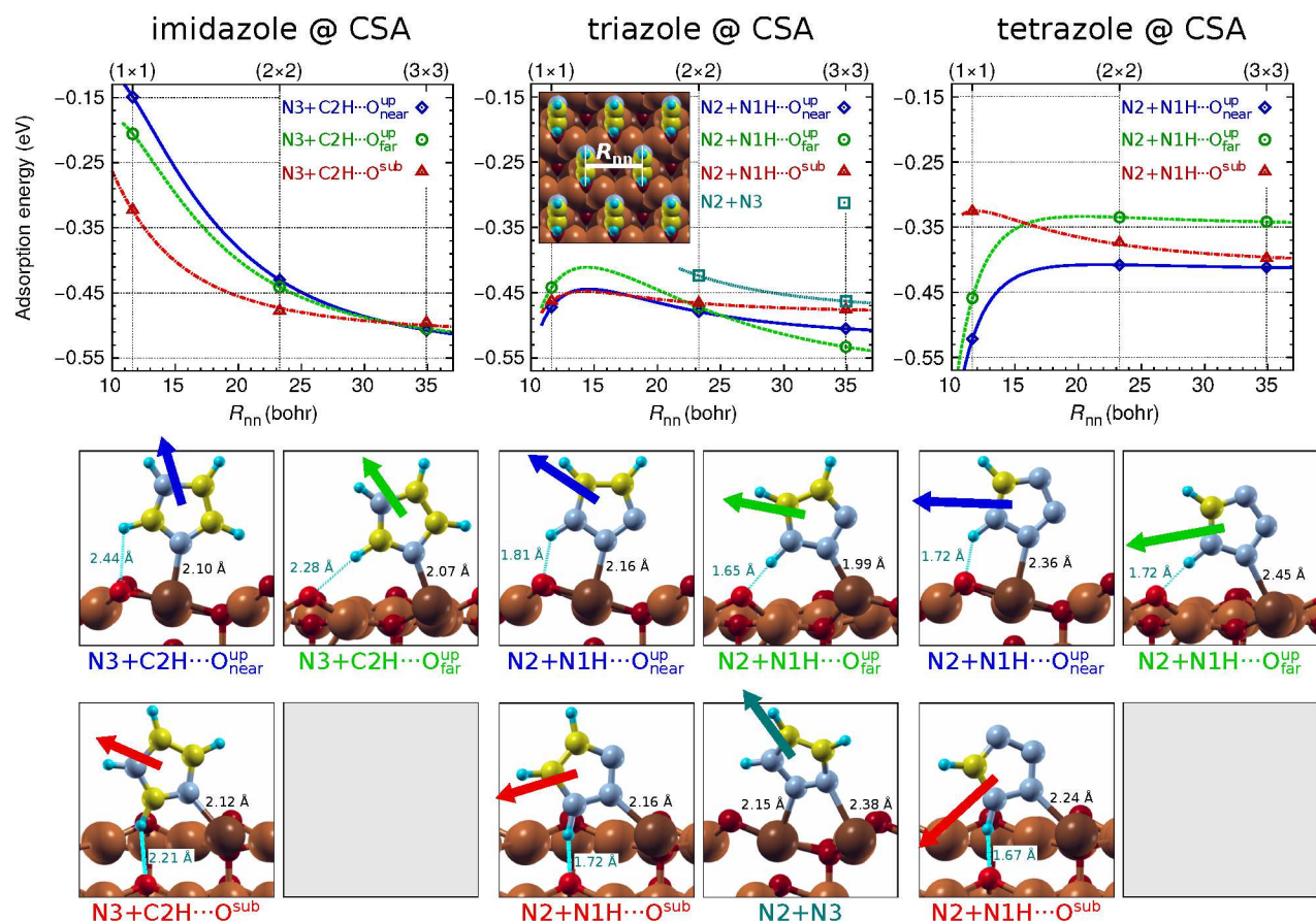
Fig. 1 Top: adsorption energy as a function of nearest-neighbor intermolecular distance ( R_{nn} , defined graphically in the inset at the center) for imidazole, triazole, and tetrazole bonded at a CSA site of \text{Cu}_2\text{O}(111)\text{-w/o-Cu}^{\text{CUS}} . Curves are mainly drawn to guide the eye as to make the plots more readable; they were calculated using the polarizable point-dipole model of ref. 47. Calculations were performed using the (1 × 1), (2 × 2), and (3 × 3) supercells. Bottom: snapshots of pertinent adsorption modes, as obtained with the (3 × 3) supercell, superimposed with dipole vectors of isolated molecules. The corresponding N–Cu bond lengths and H...O distances are also stated.
