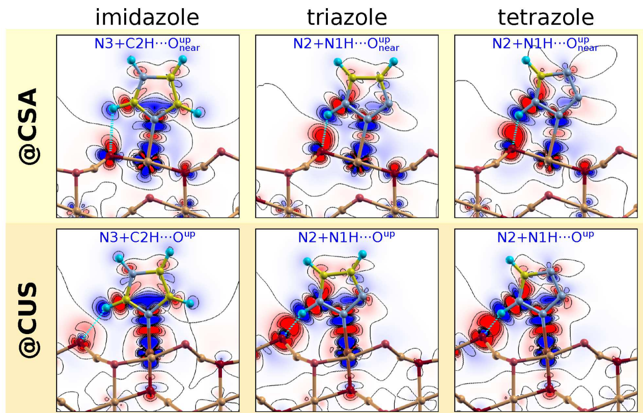
Fig. 6 Electron charge density difference, \Delta\rho(\mathbf{r}) , for imidazole, triazole, and tetrazole bonded at CSA (top) and CUS (bottom) sites. Plots are drawn with seven contours in linear scale from -0.006 to +0.006 e/a_0^3 . The blue (red) color represents the electron deficit (excess) regions; i.e. , electron charge flows from blue to red regions.
