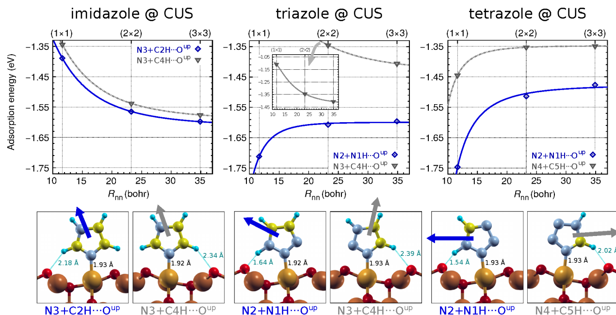
Fig. 2 As in Fig. 1 but for the molecular bonding at a CUS site. Adsorption energies are calculated with respect to high-symmetry position of \text{Cu}^{\text{CUS}} ions in the bare substrate as to better represent the molecule–surface bond strengths. Note that the \text{Cu}^{\text{CUS}} ions of the bare substrate relax laterally to a more stable asymmetric position if the symmetry is broken (see Fig. 1 in ref. 9) with the energy stabilization of 0.13 eV at full ( \Theta = 1 ) and 0.04 eV at lower surface concentration ( \Theta \leq 1/4 ) of extraneous \text{Cu}^{\text{CUS}} ions at \text{Cu}_2\text{O}(111)\text{-w/o-Cu}^{\text{CUS}} .
