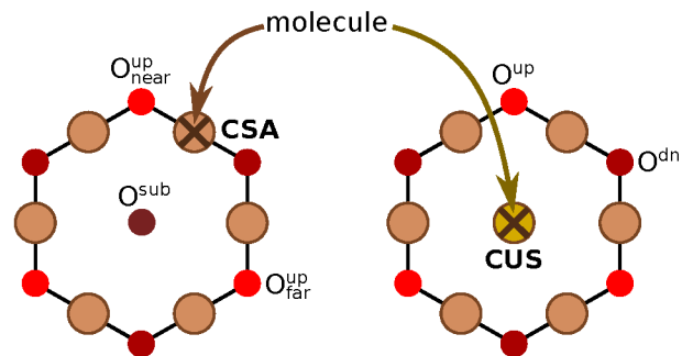
Scheme 3 Definition of various O sites near an adsorbed molecule at the CSA site on \text{Cu}_2\text{O}(111)\text{-w/o-Cu}^{\text{CUS}} (left) and CUS site (right). Molecule adsorbed at the CSA site can form a hydrogen bond with either \text{O}_{\text{near}}^{\text{up}} , \text{O}_{\text{far}}^{\text{up}} , or \text{O}^{\text{sub}} . In contrast, molecule adsorbed at the CUS site can only form a hydrogen bond with one among the three equivalent nearby \text{O}^{\text{up}} ions.
