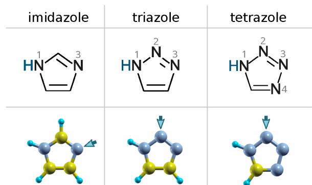
Scheme 1 Skeletal formulae of imidazole, triazole, and tetrazole with the numbering of N atoms (top) and ball-and-stick models of optimized molecular structures (bottom). Arrows indicate the N atoms that preferentially bond with \text{Cu}_2\text{O} surfaces (see Section 3).
