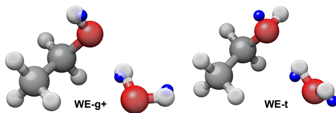
Fig. 4 Kraitchman substitution positions of three hydrogens in the ethanol water dimer are shown as blue spheres, superimposed on the ab initio structures of WE-g+ (left) and WE-t (right). Based on the substitution positions, it is clear that WE-g+ is the measured conformer.
