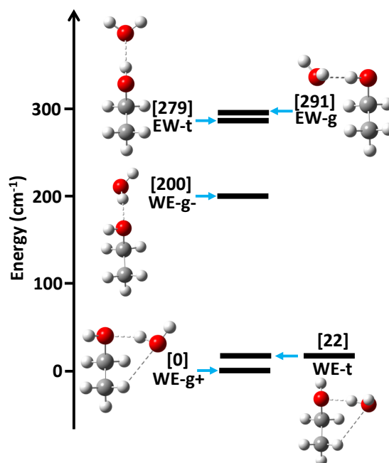
Fig. 1 The ab initio relative energy landscape, including ZPVE, of the ethanol-water dimer. Geometry optimizations and harmonic force field calculations were performed at the MP2/aug-cc-pVTZ level of theory, followed by single point energy calculations using CCSD(T)/aug-cc-pVTZ.
