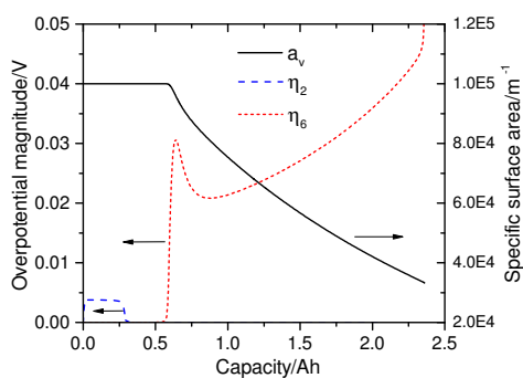
Fig. 3 Simulated activation overpotentials \eta_2 (for reaction Eq. 2) and \eta_6 (for Eq. 6) during 0.15C discharge, and the specific electrochemical surface area ( a_v ) during discharge.
