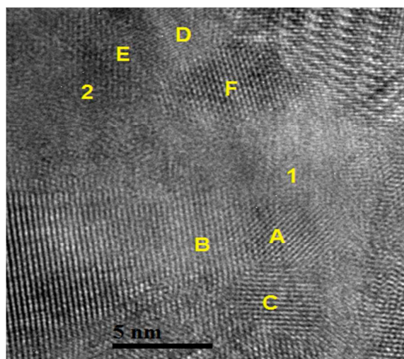
Figure 12. TEM micrograph indicating localised amorphous regions (1) and (2). Attributed phases for the lattice spacing present include: (A) (011) Mg; (B) and (C) (011) \text{CaB}_6 ; (D) 1.98 Å (011) hkl reflection \text{CaB}_6 (E) and (F) 2.49 Å, Mg.
