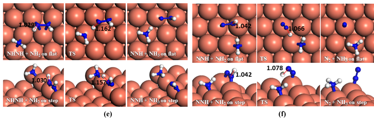
Fig. 12. Schematic representation of the initial, transition and final states for dehydrogenation pathways on the flat (top-view) and stepped (side-view) Cu(111) via \text{NH}_2 attacking to (a) \text{N}_2\text{H}_4 , (b) and (c) \text{N}_2\text{H}_3 , (d) \text{NNH}_2 , (e) \text{NHNH} and (f) \text{NNH} . Bond lengths are given in Å.
