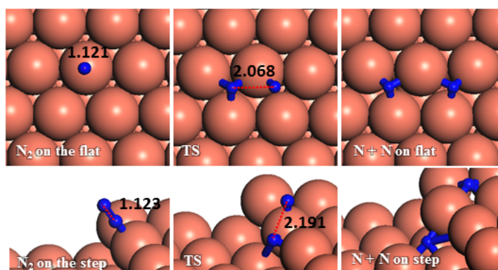
Fig. 9. Schematic representation of the initial, transition and final states for N 2 dissociation pathways on the flat (top-view) and stepped (side-view) Cu(111) surfaces. Bond lengths are given in Å.
