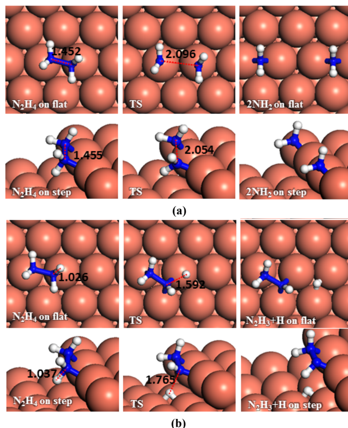
Fig. 4. Schematic representation of the initial, transition and final states for N_2H_4 dissociation pathways on the flat (top-view) and stepped (side-view) Cu(111) surfaces via (a) N–N, (b) N–H breaking. Bond lengths are given in Å.
