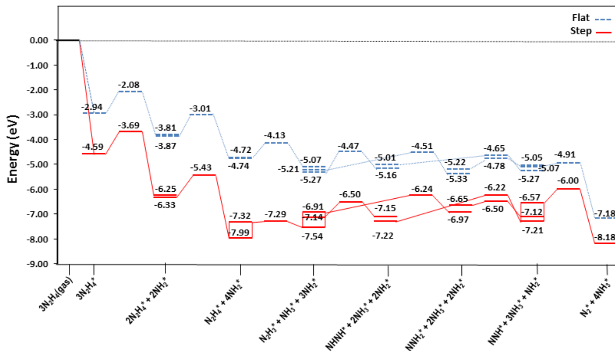
Fig. 16. Reaction profiles for dissociation of N_2H_4 via intermolecular dehydrogenation via NH_2 on the flat (---) and stepped (—) Cu(111) surfaces. Energies are relative to the energy of the gas-phase hydrazine (in eV). Note that we have considered the diffusion of intermediates to their most stable adsorption sites on the surface as a barrier-less pathway.
