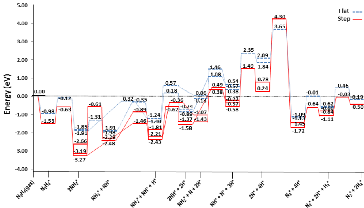
Fig. 15. Reaction profiles for dissociation of N_2H_4 via N-N bond breaking and subsequent dehydrogenation pathways on the flat (---) and stepped (—) Cu(111) surfaces. Energies are relative to the energy of the gas-phase hydrazine (in eV). Note that we have considered the diffusion of intermediates to their most stable adsorption sites on the surface as a barrier-less pathway.
