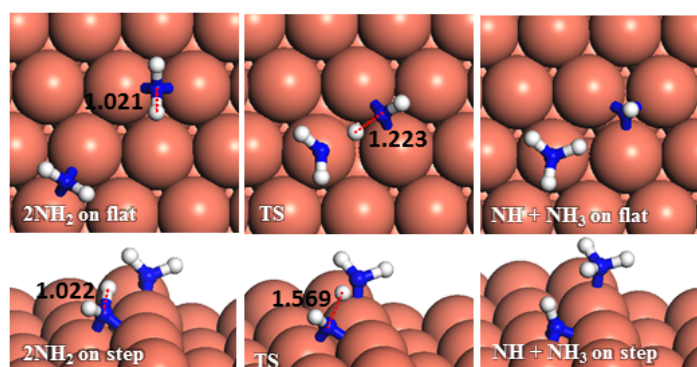
Fig. 13. Schematic representation of the initial, transition and final states for dehydrogenation pathway via \text{NH}_2 attacking \text{NH}_2 on the flat (top-view) and stepped (side-view) Cu(111) surfaces. Bond lengths are given in Å.
