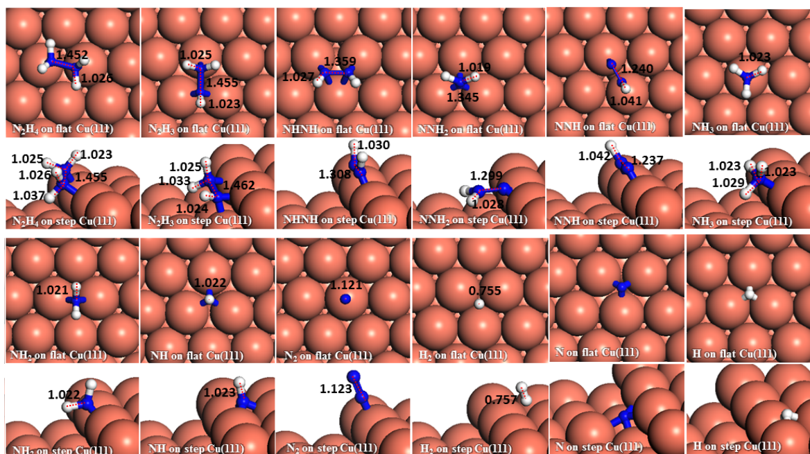
Fig. 3. Surface geometries of the most preferred adsorption configurations of the various intermediates on the flat (top-view) and stepped (side-view) Cu(111) surfaces with their N–N and N–H bond distances in Å.
