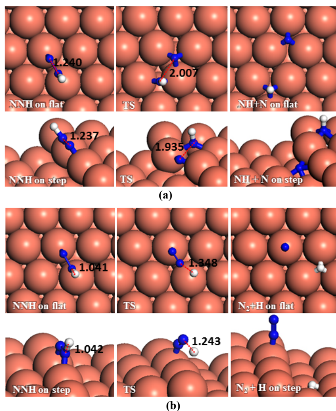
Fig. 8. Schematic representation of the initial, transition and final states for NNH dissociation pathways on the flat (top-view) and stepped (side-view) Cu(111) surfaces via (a) N–N, (b) N–H breaking. Bond lengths are given in Å.
