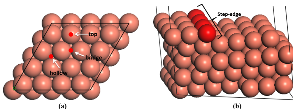
Fig. 1. The simulation cells and surface geometry of different sites used in the calculations of (a) perfect (top view) and (b) stepped (side view) surfaces. Note that low-coordinated atoms in the stepped surface are shaded darker.
