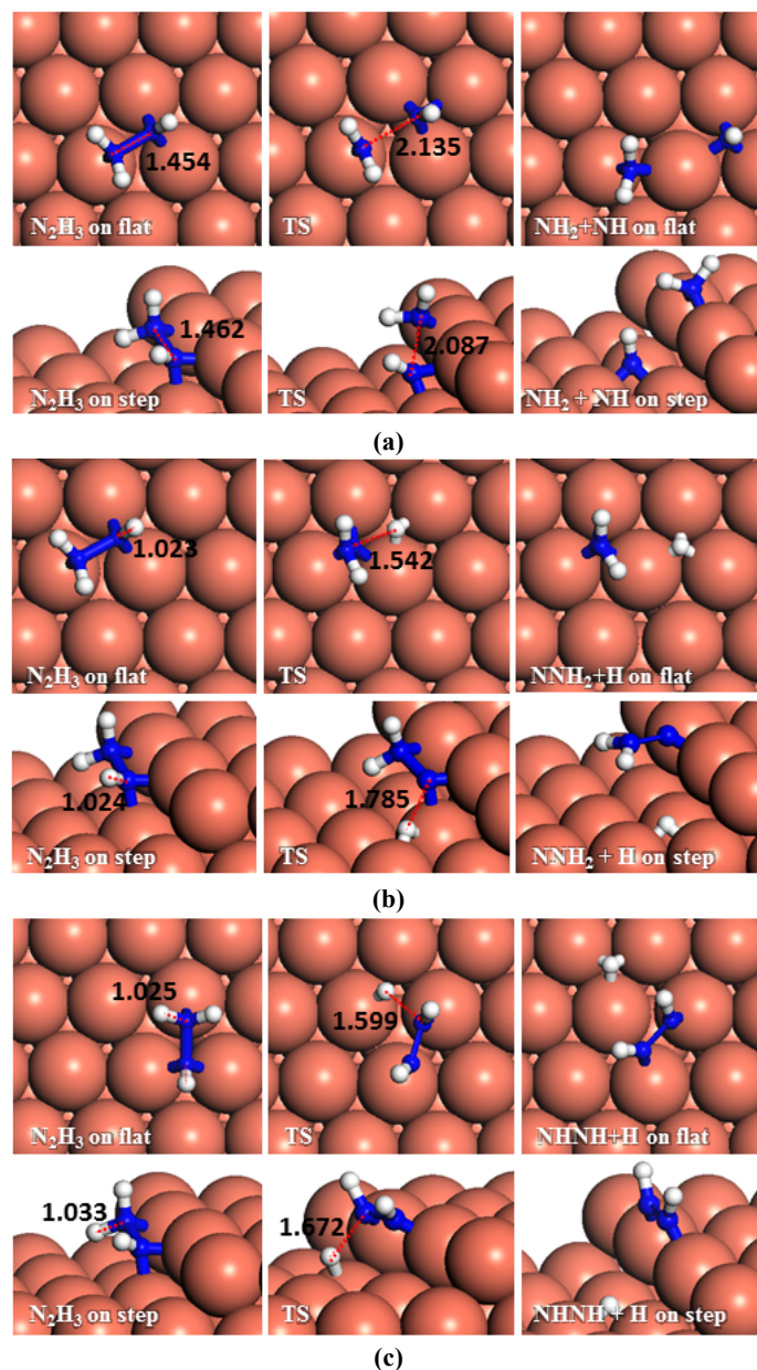
Fig. 5. Schematic representation of the initial, transition and final states for N_2H_3 dissociation pathways on the flat (top-view) and stepped (side-view) Cu(111) surfaces via (a) N–N, (b) and (c) N–H breaking. Bond lengths are given in Å.
