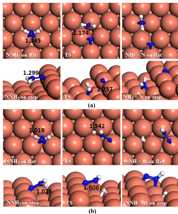
Fig. 6. Schematic representation of the initial, transition and final states for \text{NNH}_2 dissociation pathways on the flat (top-view) and stepped (side-view) \text{Cu}(111) surfaces via (a) N–N, and (b) N–H breaking. Bond lengths are given in Å.
