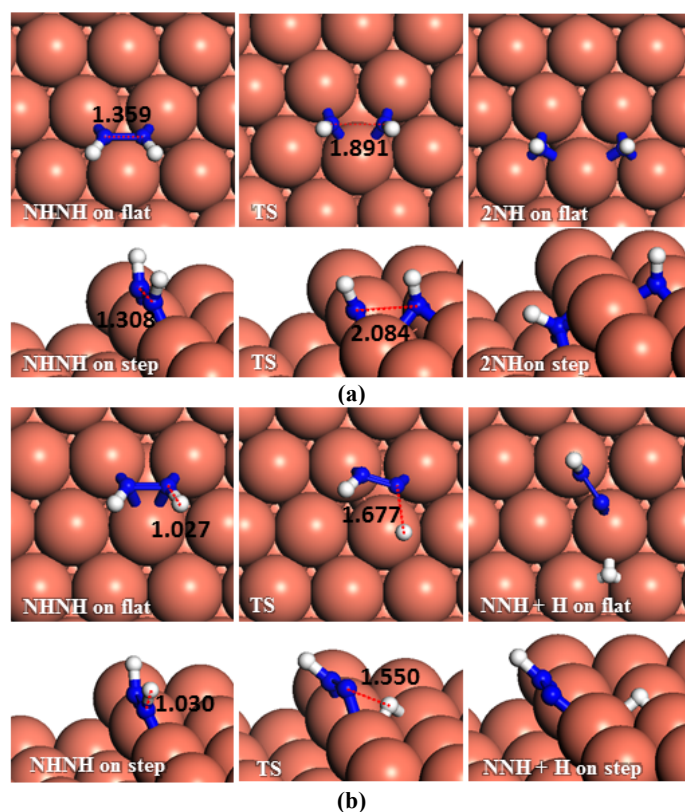
Fig. 7. Schematic representation of the initial, transition and final states for NHNH dissociation pathways on the flat (top-view) and stepped (side-view) Cu(111) surfaces via (a) N–N, and (b) N–H breaking. Bond lengths are given in Å.
