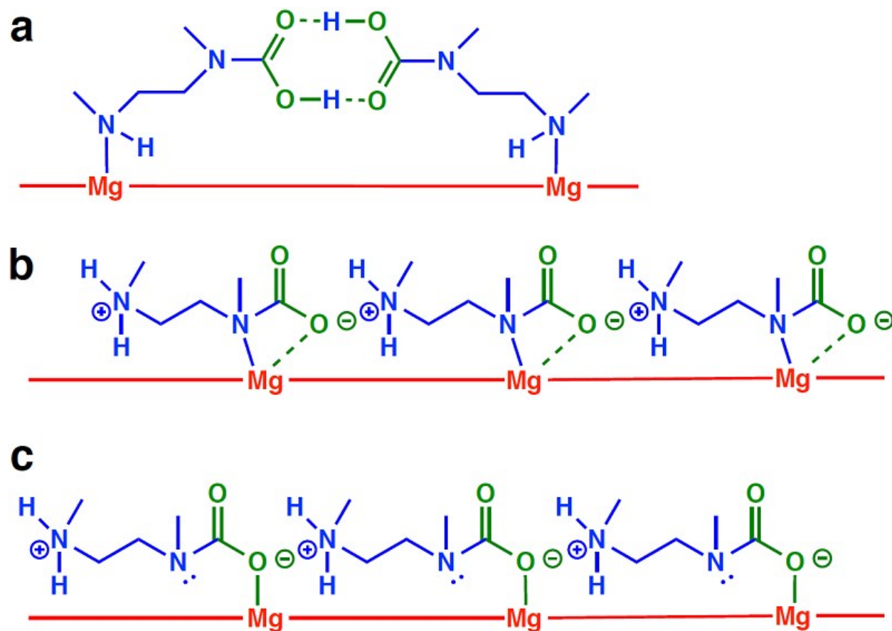
Figure 2: a) The “pairs structure”. A CO 2 molecule binds to the free end of each amine, creating a carbamic acid which then forms a hydrogen bonded pair with its neighbor. b) The “chain structure”. CO 2 adsorbs to the metal-bound end of each amine, and the free end of each amine removes a hydrogen from its neighbor, creating ammonium carbamate (or neutral amine / carbamic acid) chains along the channels of the MOF. c) The “insertion structure”. Similar to the chain structure, except that the adsorbed CO 2 inserts into the metal-nitrogen bond, forming ammonium carbamate chains that are bound to the metals through the carbamate oxygen atoms.
