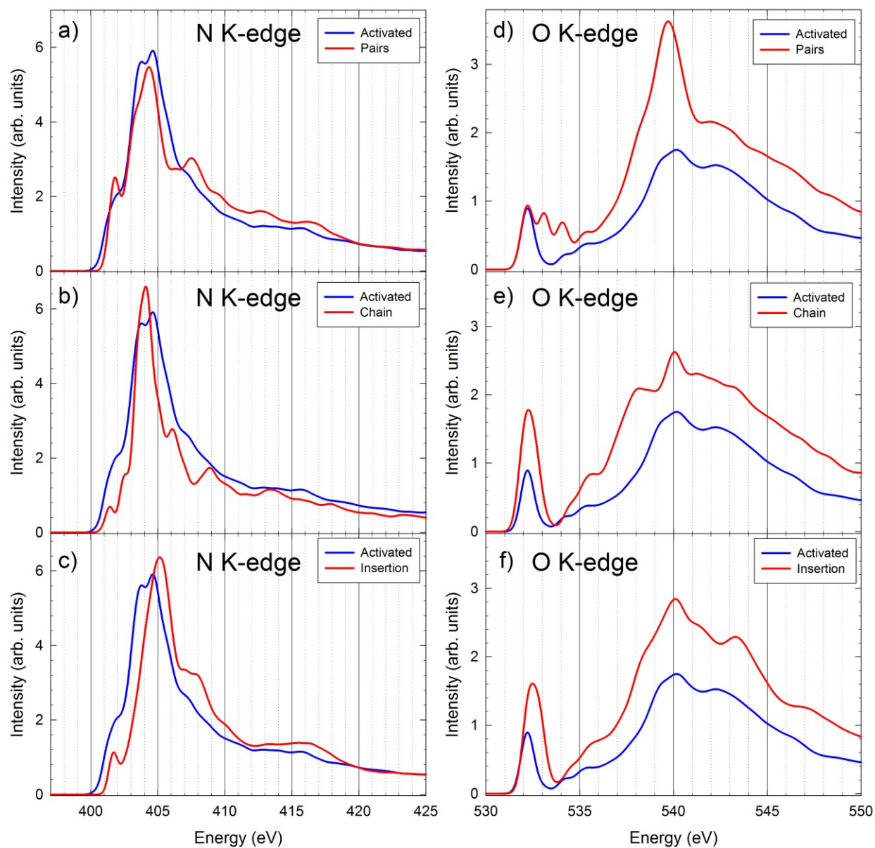
Figure 3: Top row: computed N K-edge (left) and O k-edge (right) spectra for the activated MOF and the pairs structure at zero K. The N K-edge spectra reproduce the new peak near 402 eV but not the blueshift or increase in intensity of the main edge at 404.5 eV. The O K-edge spectra show two new \pi^* peaks at 533 and 534 eV. Middle row: computed N K-edge (left) and O K-edge (right) spectra for the activated MOF and the chain structure at zero K. The N K-edge spectra do not show any of the experimentally observed changes. The O K-edge spectra show a slight broadening of the \pi^* peak near
