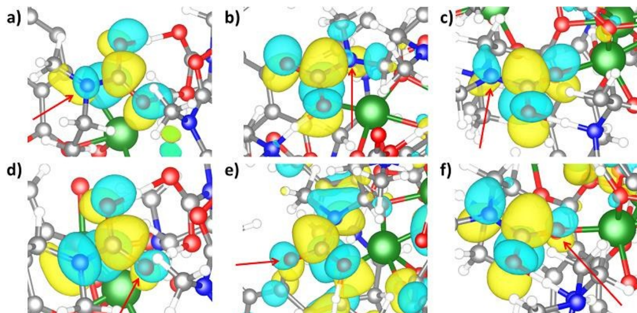
Figure 5: Top row: final state wavefunctions corresponding to the peak near 402 eV in the N K-edge spectra for the pairs structure (left), chain structure (center) and insertion structure (right). Red arrows indicate the excited atom in each case. Bottom row: final state wavefunctions corresponding to the \pi^* peak in the O K-edge spectra for the pairs structure (left), chain structure (center) and insertion structure (right). Red arrows indicate the excited atom in each case. These states closely resemble those in the top row, indicating a similar electronic structure accessed from both nitrogen and oxygen excitations.
