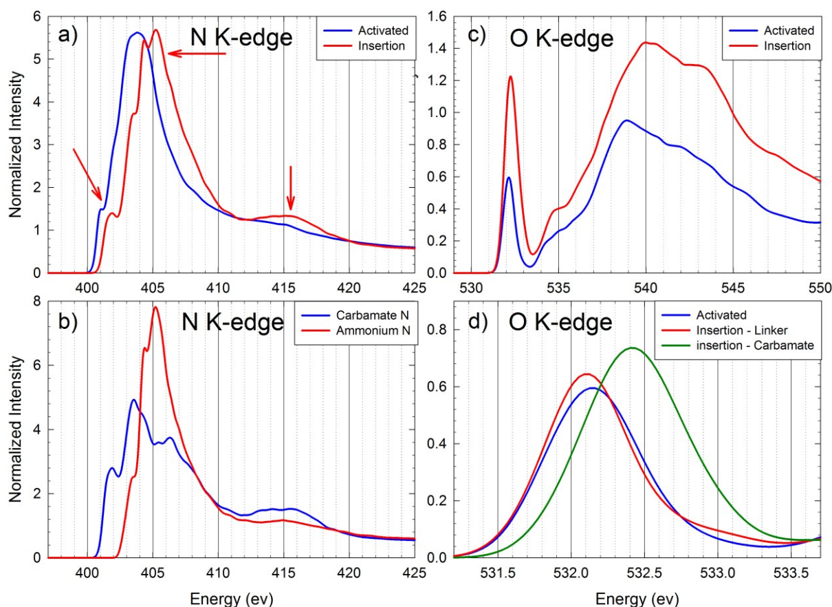
Figure 4: a) Computed N K-edge spectra for the activated MOF and insertion structure at 298 K. All three major spectral changes seen in experiment are reproduced, marked with red arrows: a new peak at 402 eV, a blueshift and increase in intensity of the main edge peak at 403.8 eV, and a new broad feature between 412 and 419 eV. b) Computed N K-edge spectra for the insertion structure at 298 K, with contributions divided between carbamate N atoms and ammonium N atoms. The new peaks at 402 eV and 407.2 eV, as well as the broad feature between 412 and 419 eV, arise solely from the carbamate N atoms. The increase in intensity and blueshift of the main edge peak near 404 eV arises primarily from the ammonium N atoms. c) Computed O k-edge spectra for the activated MOF and insertion structure at 298 K. New \pi^* resonances from the adsorbed \text{CO}_2 appear at slightly higher energy, but not as high as in experiment. d) A zoomed-in plot of the \pi^* feature at the O K-edge, including contributions to the
