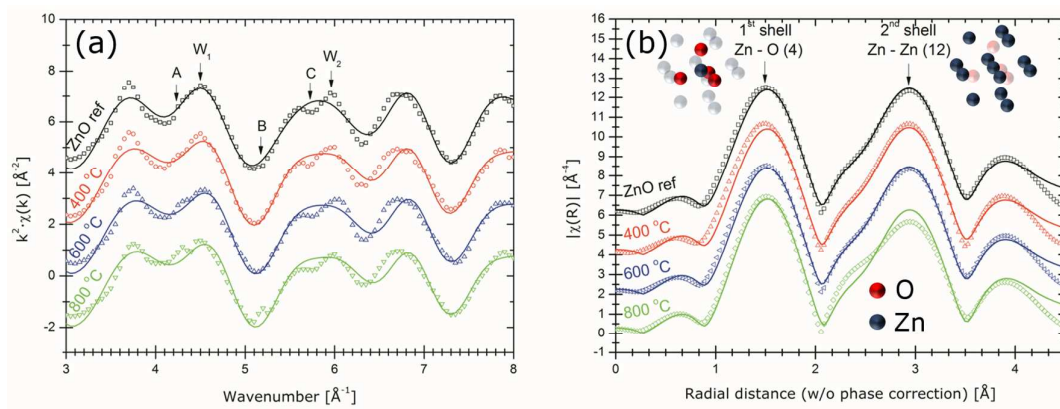
Figure 5: k^2 \cdot \chi(k) (a) and its Fourier transform (b) for the ZnO reference and the samples annealed between 400 and 800 °C. Experimental data are represented with hollow symbols while fit to data is shown with continuous lines. FT is not phase-corrected. An inset to figure (b) shows the atoms in the structure contributing to the shell.
