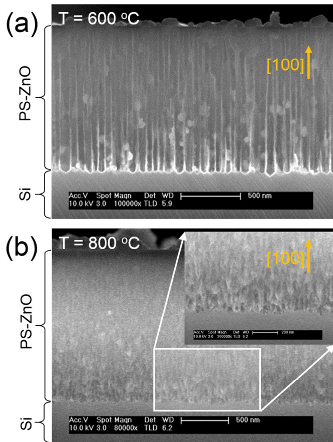
Figure 1: Cross-sectional FESEM images of the samples annealed at 600 °C (a) and 800 °C (b).
