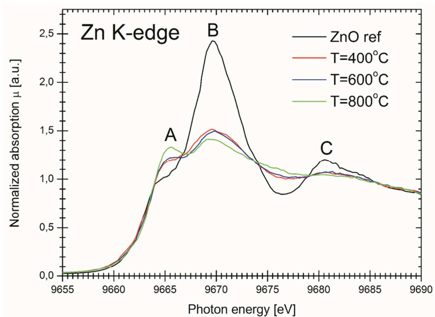
Figure 4: XANES spectra of the PS-ZnO nanocomposites and a bulk ZnO reference. PS-ZnO samples have been annealed at 400, 600 and 800 °C in atmospheric conditions.
