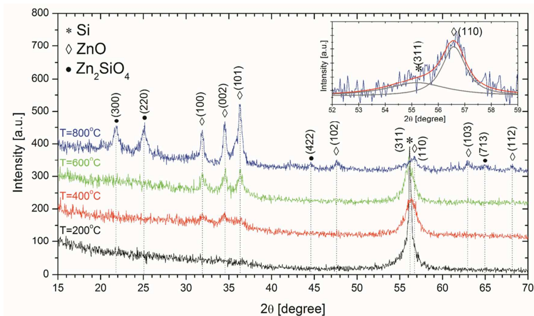
Figure 2: GIXD patterns from PS-ZnO samples annealed between 200 and 800°C. The inset shows the deconvolution of the peak centered on 2\theta = 56^\circ .
