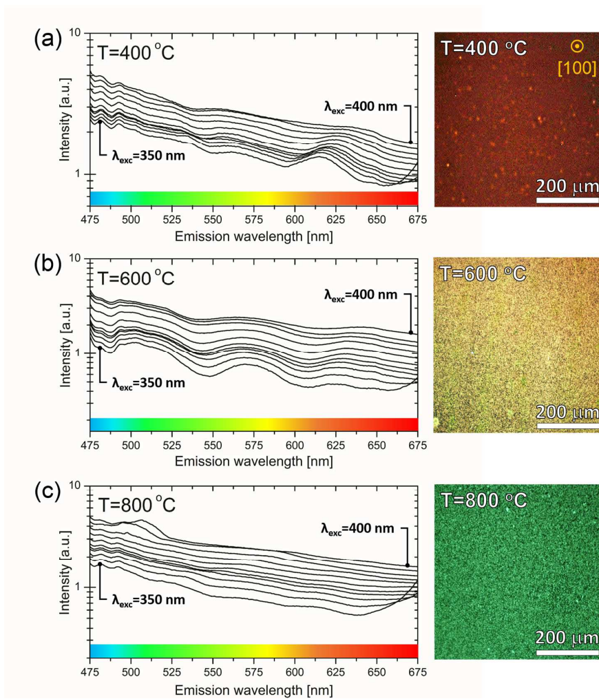
Figure 6: PL measurements and fluorescence microscopy images taken from the samples annealed at temperatures between 400 °C and 800 °C. Note that the features observed at 481 nm and 492 nm correspond to discrete lamp emission lines.
