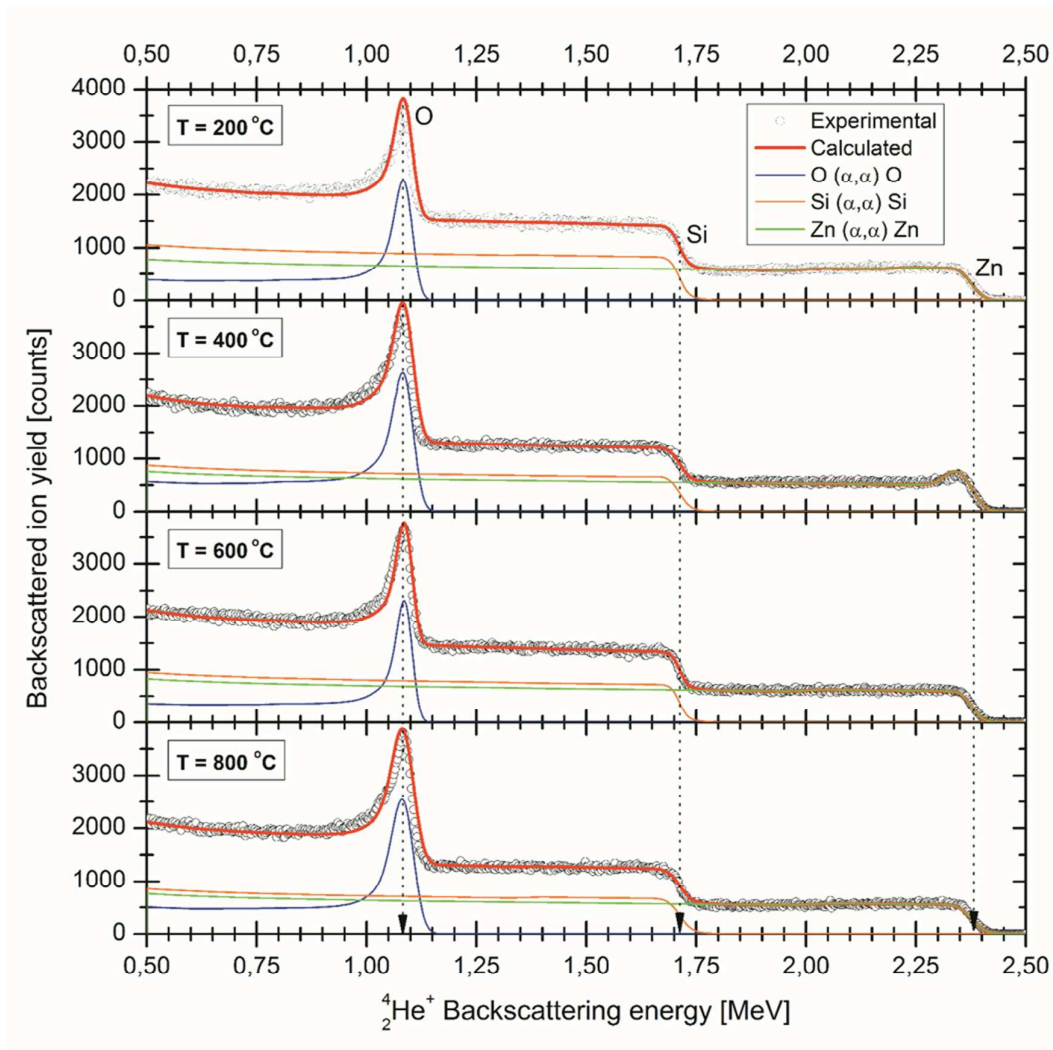
Figure 3: EBS results for the samples annealed between 200 and 800 °C (hollow dots - experimental data, continuous line – fitted spectra) with individual contributions of Zn, O and Si to each fitting.
