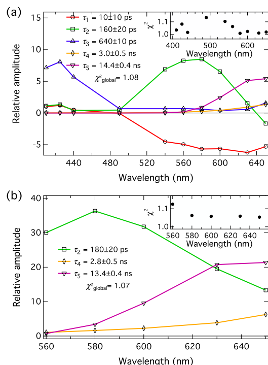
Fig. 8 Decay associated spectra of C 4 -dHONI ( c = 40 \text{ }\mu\text{M} ) in MeCN in the presence of (a) 200 mM of NMI ( \lambda_{\text{exc.}} = 360 \text{ nm} ) and (b) 250 \mu\text{M} of DBU ( \lambda_{\text{exc.}} = 460 \text{ nm} ). The insets show the individual \chi^2 -values at each wavelength. The time constants in (b) are given the same labels as the corresponding ones in (a).
