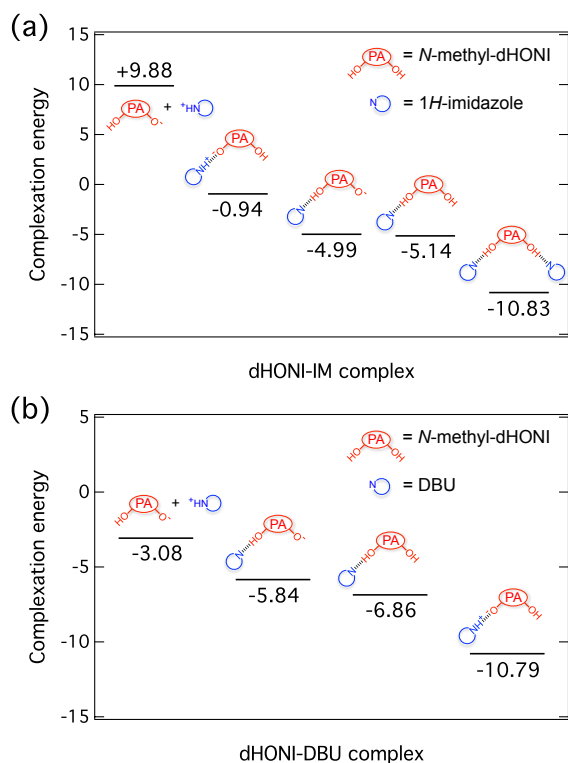
Fig. 2 Calculated complexation energies (kcal/mol) of different (a) dHONI ... IM and (b) dHONI ... DBU ground-state complexes in MeCN.
