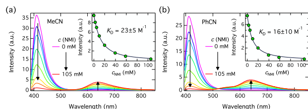
Fig. 5 Steady-state emission spectra of C4-dHONI ( c = 9 \mu\text{M} ) upon addition of NMI in (a) MeCN ( \lambda_{\text{exc.}} = 381.5 \text{ nm} ) and (b) PhCN ( \lambda_{\text{exc.}} = 387 \text{ nm} ). The insets show the integrated emission intensities together with Stern-Volmer fittings for combined quenching, Eq. (1).
