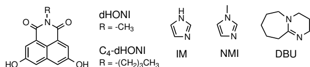
Chart 1 Structures of the studied compounds.
