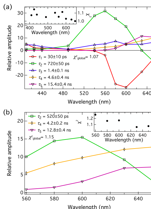
Fig. 9 Decay associated spectra of C 4 -dHONI ( c = 40 \text{ }\mu\text{M} ) in PhCN in the presence of (a) 200 mM of NMI ( \lambda_{\text{exc.}} = 360 \text{ nm} ) and (b) 250 \mu\text{M} of DBU ( \lambda_{\text{exc.}} = 460 \text{ nm} ). The insets show the individual \chi^2 -values at each wavelength. The time constants in (b) are given the same labels as the corresponding ones in (a).
