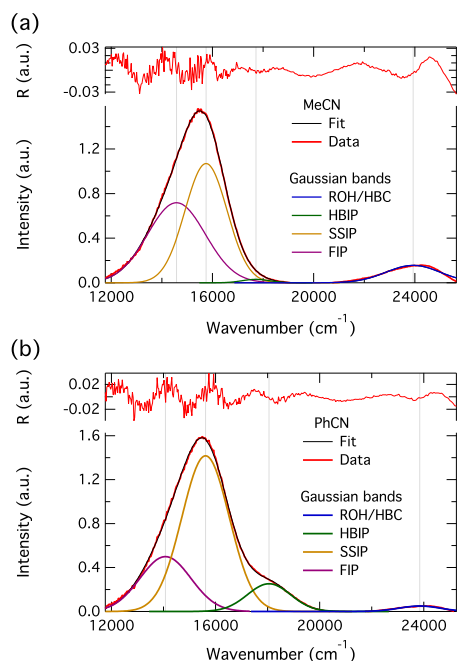
Fig. 10 Decomposed emission spectra of C 4 -dHONI in the presence of NMI in (a) MeCN and (b) PhCN. The residuals are shown on top. The three long-wavelength emission bands are attributed to the three ion pair species as indicated in the legends.
