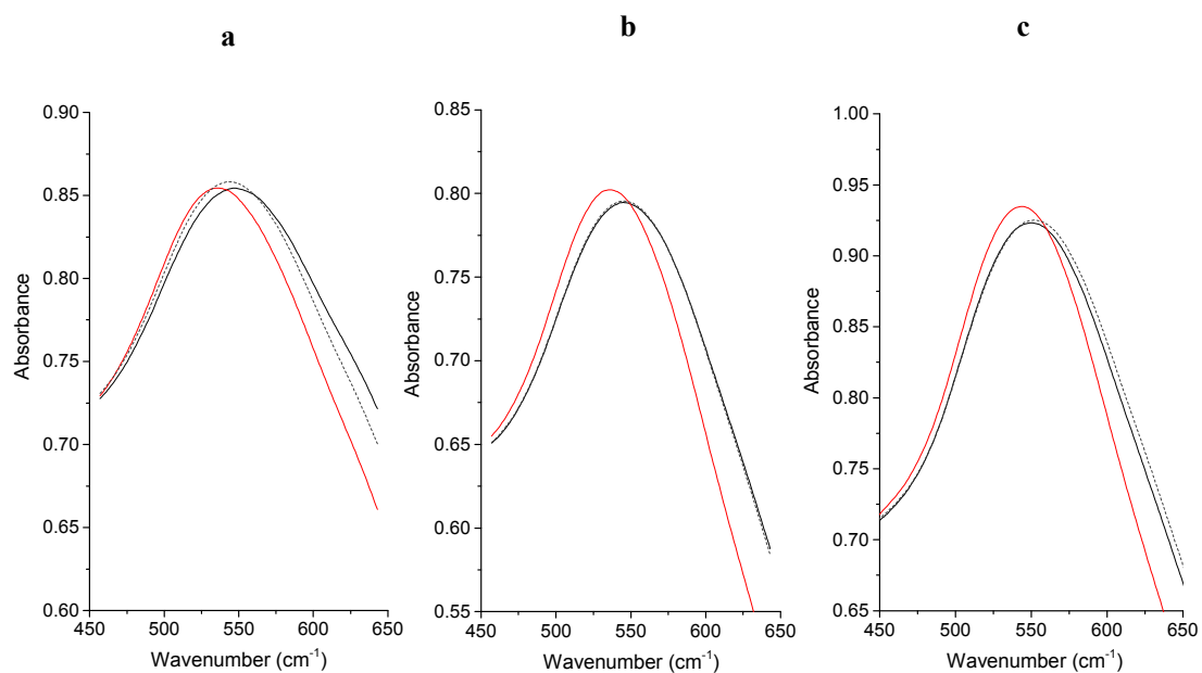
Figure 5: UV-Vis analysis of catalyst under N_2 (black), 0.5% CO/N_2 (red) and returning to a N_2 (black dots) environment : 1 wt.% Au/TiO 2 catalysts before treatment (a), after 1 h reflux (b) and calcination at 500°C (c)
