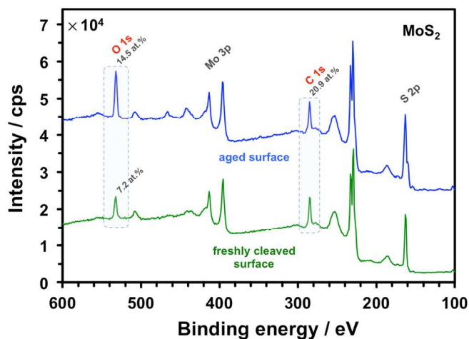
Fig. 5 XPS spectra recorded on the aged (blue) and freshly cleaved (green) MoS 2 surface. Each spectrum is an average combined from 5 different areas. The main element peaks (labelled) were used for the quantification (ESI†, Table S1).
