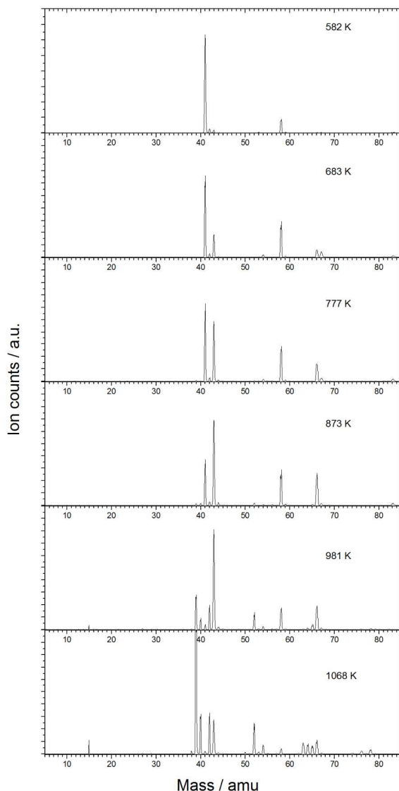
Figure 1: All-electron mass spectra of the pyrolysis of 0.5% allyl iodide in acetylene at temperatures of 582, 683, 777, 873, 981, and 1068 K, recorded at a photon energy of 9.5 eV.
