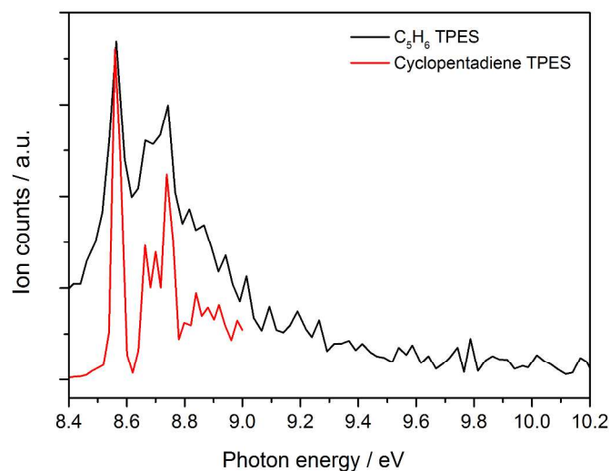
Figure 3: Mass selected threshold photoelectron spectrum of C 5 H 6 formed in the reaction between C 3 H 5 • and C 2 H 2 (in black) plotted together with a measured spectrum of cyclopentadiene (in red).
