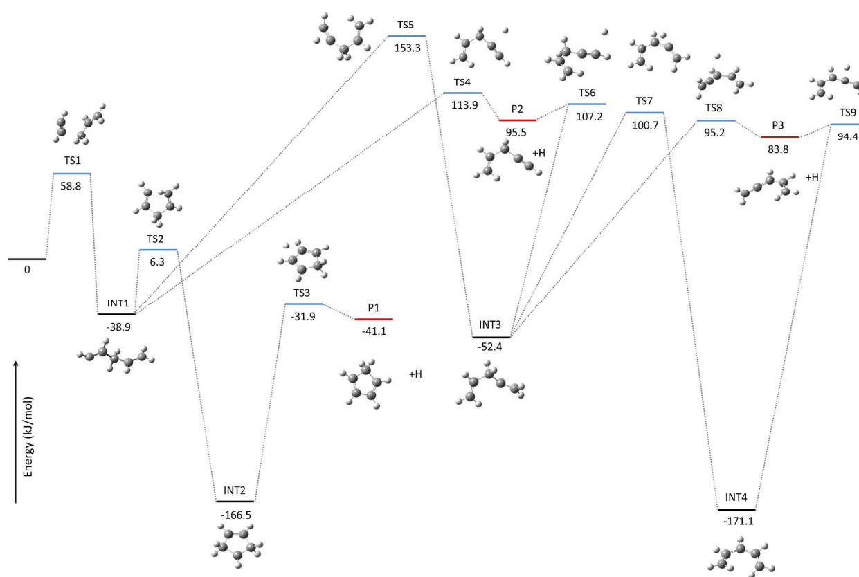
Figure 4: C 5 H 7 potential energy surface obtained at the CBS-QB3 level of theory. All energies are shown in kJ mol -1 relative to the energy of C 3 H 5 + C 2 H 2 . Products (red), intermediate states (black) and transition states (blue) are color coded.
