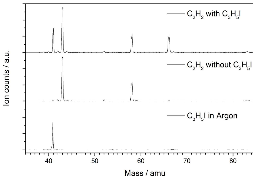
Figure 2: Comparison of mass spectra recorded for the pyrolysis of C_3H_5I in Ar at 823 K (bottom), pyrolysis of C_2H_2 at 873 K (middle) and pyrolysis of C_2H_2 in presence of C_3H_5I at 873 K (top).
