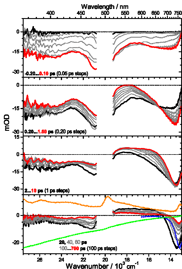
Fig. 3 Transient PSCP absorption spectra of CH 3 NH 3 PbI 3 (1-step deposition on TiO 2 /glass) after excitation at 500 nm: (first panel) -0.20...0.10 ps with 50 fs steps; (second panel) 0.20...1.60 ps with 0.20 ps steps; (third panel) 2...10 ps with 1 ps steps; (fourth panel) 20, 40, 60 ps and 100...700 ps (100 ps steps). Selected transient spectra are shown as thick colored lines for guidance. The green dotted line in the bottom panel corresponds to the inverted and scaled steady-state absorption spectrum; the orange-dotted line is the smoothed and scaled first derivative of the steady-state absorption spectrum; the blue-dotted line corresponds to the scaled steady-state stimulated emission spectrum of CH 3 NH 3 PbI 3 . The OD at the excitation wavelength was 0.57.
