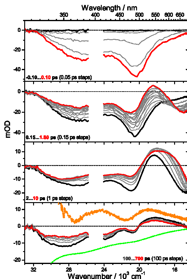
Fig. 5 Transient PSCP absorption spectra of \text{CH}_3\text{NH}_3\text{PbI}_3 on \text{TiO}_2/\text{quartz} (DSSD) for excitation at 400\text{ nm} : (first panel) -0.10\dots0.10\text{ ps} with 50\text{ fs} steps; (second panel) 0.15\dots1.80\text{ ps} with 0.15\text{ ps} steps; (third panel) 2\dots10\text{ ps} with 1\text{ ps} steps; (fourth panel) 100\dots700\text{ ps} ( 100\text{ ps} steps). Selected transient spectra are shown as thick colored lines for guidance. In the bottom panel, the green dotted line corresponds to the inverted and scaled steady-state absorption spectrum. The orange-dotted line represents the smoothed and scaled first derivative of the steady-state absorption spectrum. Data in a range of \pm 800\text{ cm}^{-1} around the center pump wavenumber are not shown due to considerable scattered pump light. The OD at the excitation wavelength was 1.19 .
