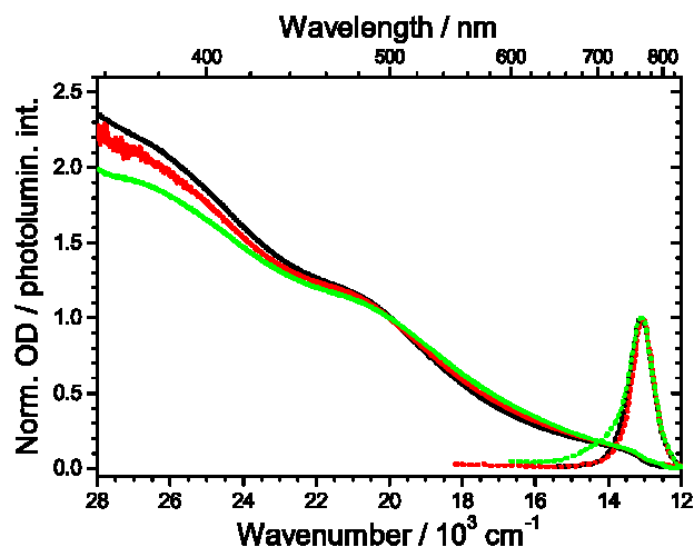
Fig. 2 Steady-state absorption (solid lines) and photoluminescence spectra (dotted lines) of the perovskite CH 3 NH 3 PbI 3 on a ca. 300 nm thick TiO 2 nanoparticle film attached to different substrates. Black: 1-step deposition of the perovskite on TiO 2 /glass. Red and green: 2-step deposition procedure on TiO 2 /glass (DSDS) and TiO 2 /quartz (DSSD), respectively. For an easier comparison, absorption spectra are set to Zero at 12000 cm -1 and normalized at 20000 cm -1 . Photoluminescence spectra are normalized at their maxima.
