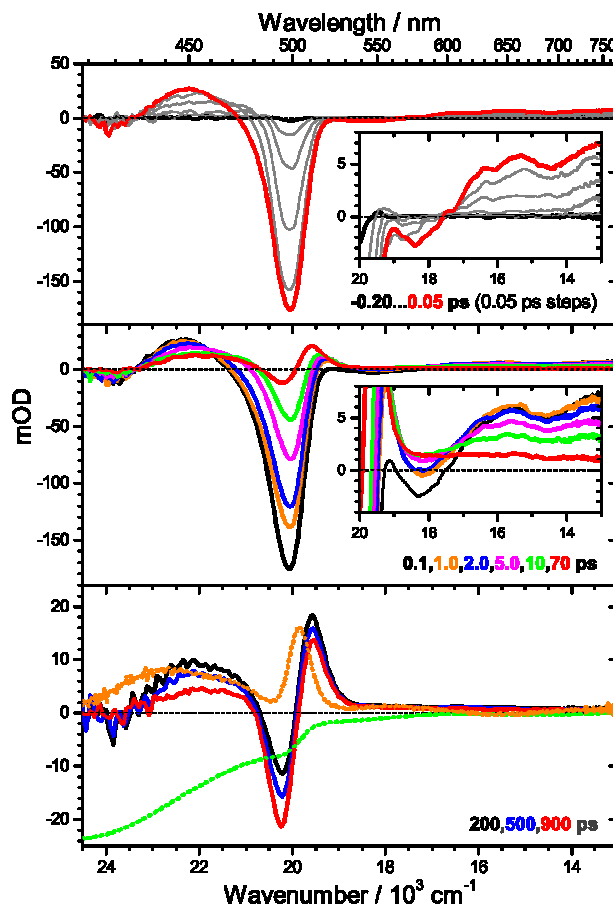
Fig. 8 Transient PSCP absorption spectra of \text{PbI}_2 on \text{TiO}_2/\text{glass} for excitation at 495 nm: (upper panel) -0.20...0.05 ps with 50 fs steps; (middle panel) 0.1, 1.0, 2.0, 5.0, 10, 70 ps; (lower panel) 200, 500, 900 ps. Selected transient spectra are shown as thick colored lines for guidance. In the lower panel, the green dotted line corresponds to the inverted and scaled steady-state absorption spectrum of \text{PbI}_2 . The orange dotted line represents the smoothed first derivative of the steady-state absorption spectrum. The insets in the top and middle panel show magnifications of the weak “absorption tail” below 20000\text{ cm}^{-1} .
