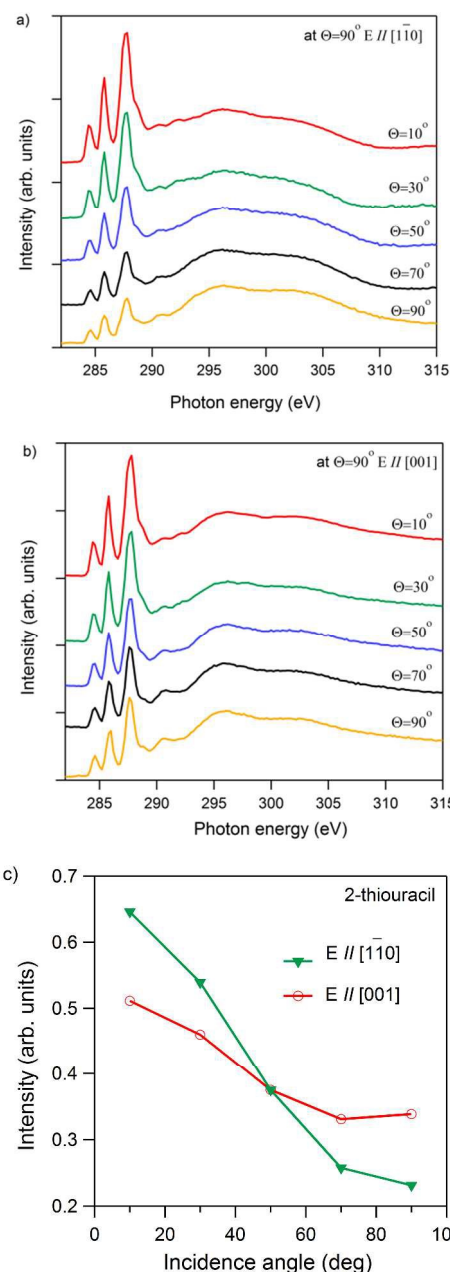
Fig. 8. C K-edge NEXAFS spectra of 2-thiouracil recorded with the photon beam polarized parallel to (a) Au [110] and (b) Au [001]. \theta = the angle between the surface plane (Au(110)) and the propagation vector of the incident photon beam; ranging from GI(10°) to NI(90°) (c) Polarisation dependence of the intensity of the \pi^* resonances in the C 1s NEXAFS spectra of 2-thiouracil.
