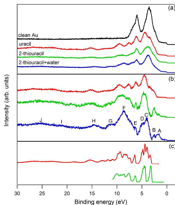
Fig. 2. (a) The valence band spectra measured with a photon energy of 120 eV for clean Au(110) surface (black); saturated coverage of uracil (red); saturated coverage of 2-thiouracil (green); and 2-thiouracil layer after exposure to water (blue); (b) Normalised spectra formed by subtraction of the clean Au(110) surface spectrum from the spectra for each molecular layer; (c) The gas phase valence band spectra for uracil and 2-thiouracil measured at photon energy of 100 eV.
