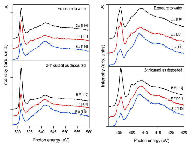
Fig. 7. (a) O K-edge and (b) N K-edge NEXAFS data for 1 ML 2-thiouracil exposed to water and 1 ML 2-thiouracil as deposited. Top scans (black) taken at GI and bottom two scans (red and blue) taken at NI.
