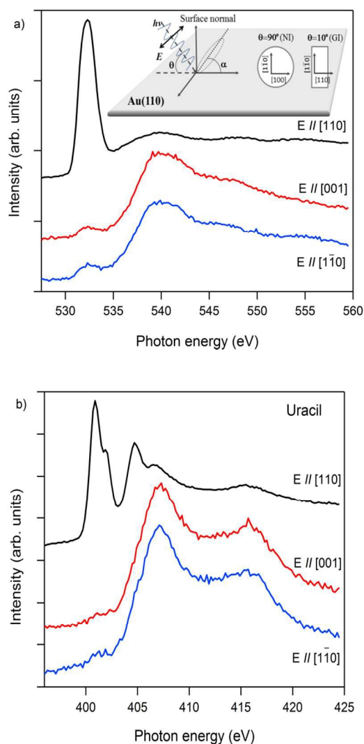
Fig. 5. (a) O K-edge and (b) N K-edge NEXAFS for uracil taken at GI (black) and at NI (red and blue).
