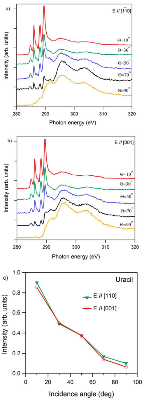
Fig. 6. C K-edge NEXAFS spectra of uracil recorded with the photon beam polarized parallel to (a) Au [1\bar{1}0] and (b) Au [001] . \theta = the angle between the surface plane (Au(110)) and the propagation vector of the incident photon beam; ranging from GI( 10^\circ ) to NI ( 90^\circ ) (c) Polarization dependence of the intensity of the \pi^* resonances in the C 1s NEXAFS spectra of uracil.
