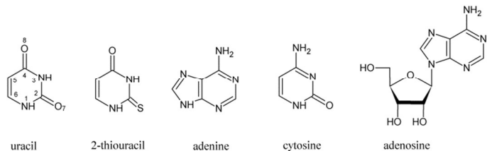
Fig. 1. Schematic structures of studied molecules.
