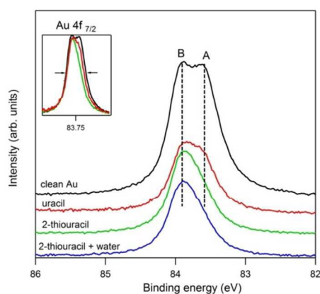
Fig. 3. Au 4f_{7/2} core-level spectra measured with a photon energy of 120 eV. From the top: (black) clean Au (110) surface; (red) uracil deposited in vacuum; (green) 2-thiouracil deposited in vacuum; (blue) vacuum deposited 2-thiouracil after exposure to water. Inset: Intensities of the clean surface spectra have been renormalised arbitrarily to allow comparison with other spectra in order to visualize the shift of the surface state A .
