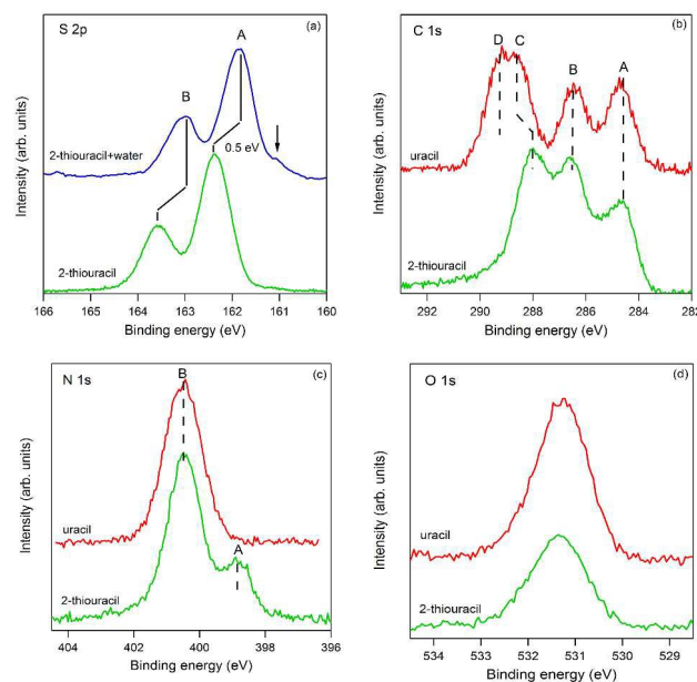
Fig. 4. (a) S 2p spectra from 2-thiouracil (green) and 2-thiouracil after exposure to water (top, blue). (b) C 1s, (c) N 1s and (d) O 1s spectra from uracil (red) and 2-thiouracil (green) measured at photon energies of 200 eV (S 2p), 500 eV (C 1s and N 1s) and 630 eV (O 1s) at NE geometry.
