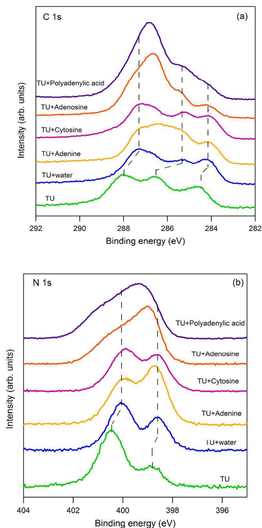
Fig. 9. (a) C 1s and (b) N 1s spectra of a pristine 2-thiouracil layer after adsorption (bottom), and after exposure to (from bottom to top): water, adenine (saturated), cytosine, adenosine, and polyadenylic acid, in solution.
