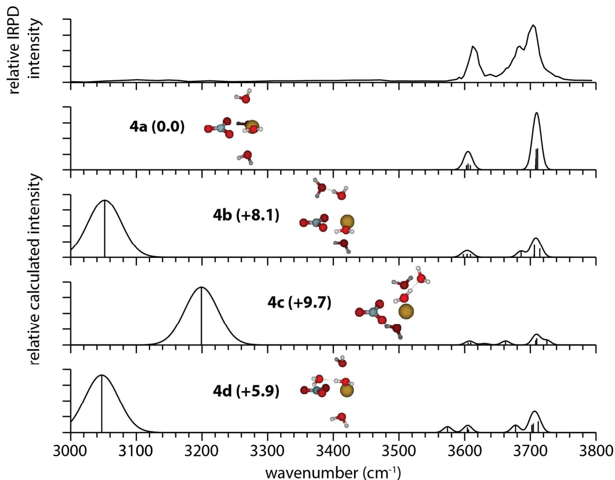
Figure 4. IRPD spectrum of [\text{PbNO}_3]^+(\text{H}_2\text{O})_4 and calculated spectra of low-energy isomers at the B3LYP/aug-cc-pVDZ level of theory, along with their relative Gibbs free energies in kJ/mol at 133 K.
