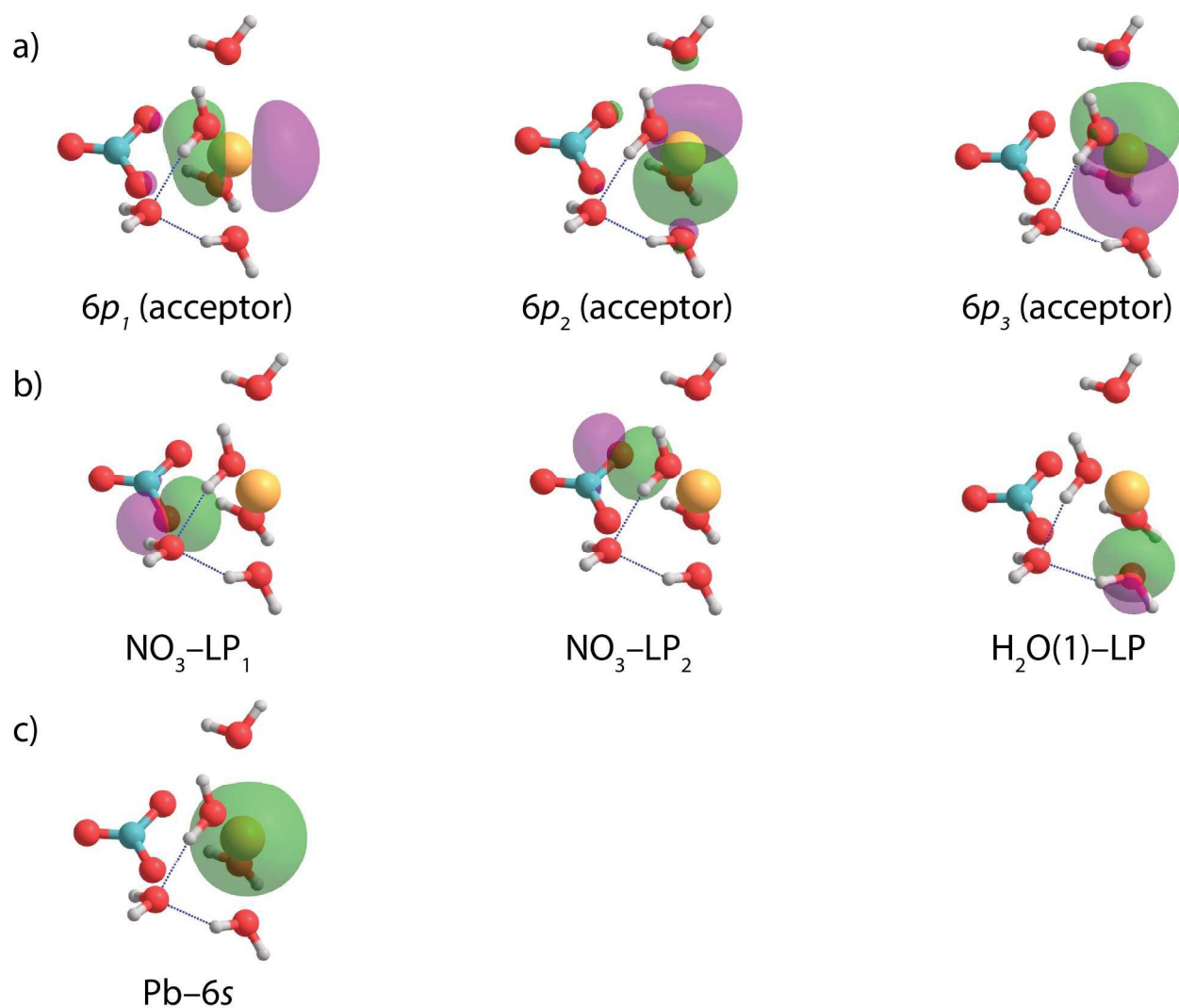
Figure 7. (a) Unfilled NBOs centered on Pb(II) that accept charge. (b) Filled NBOs on the nitrate and water ligands that donate charge. (c) NBO of valence 6s electrons on Pb(II) that has almost pure s character. All orbitals are plotted using an isosurface value of 0.05 \text{ e}/\text{\AA}^3 .
