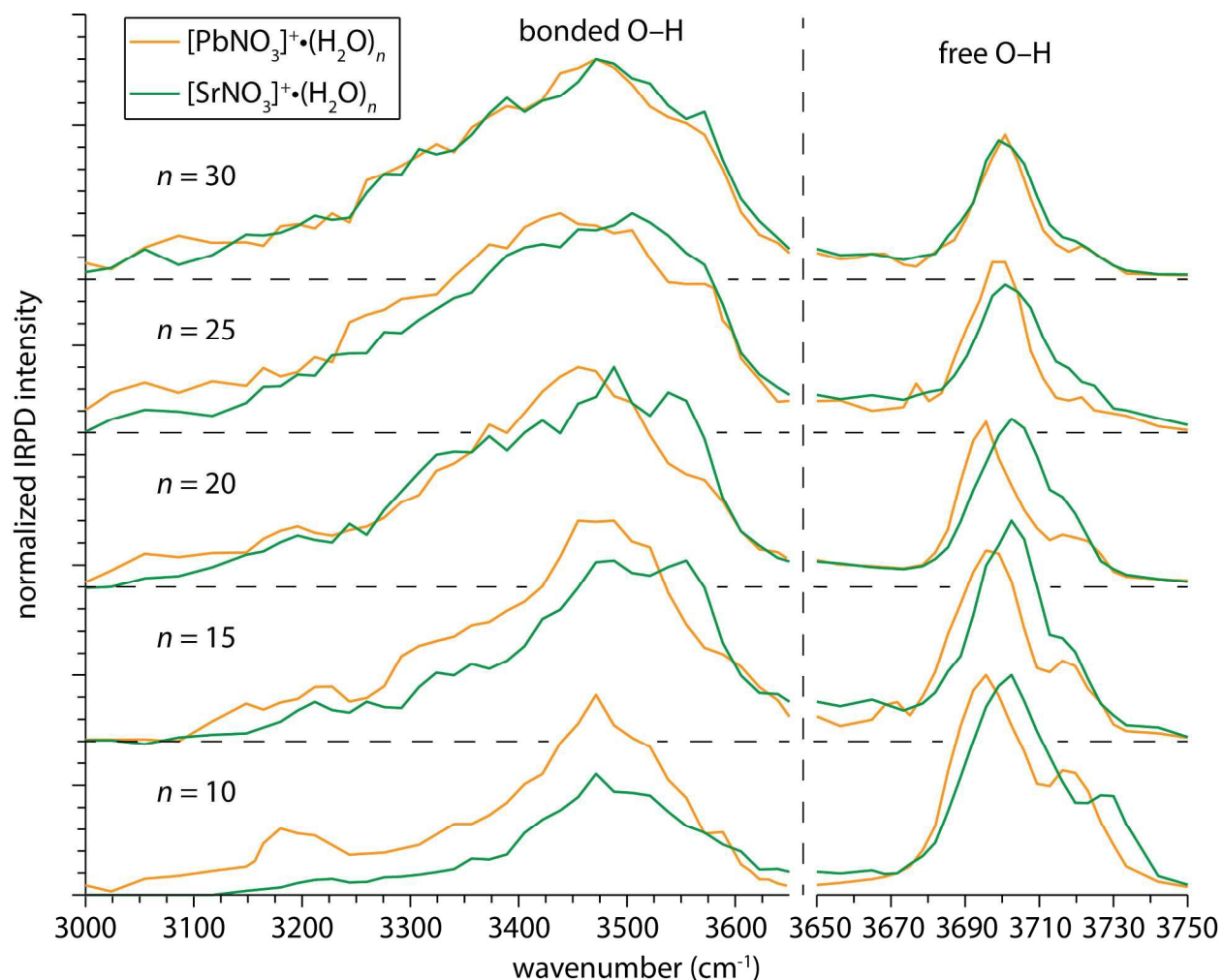
Figure 8. IRPD spectra of [\text{PbNO}_3]^+(\text{H}_2\text{O})_n and [\text{SrNO}_3]^+(\text{H}_2\text{O})_n for n = 10, 15, 20, 25, 30 in the free O—H ( \sim 3650\text{--}3750\text{ cm}^{-1} ) and bonded O—H ( \sim 3000\text{--}3650\text{ cm}^{-1} ) regions. The abscissa in the free O—H region is expanded to make the differences between these bands more clear.
