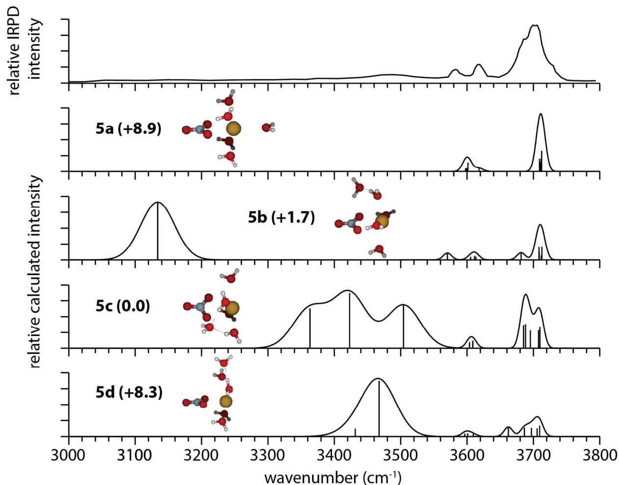
Figure 6. IRPD spectrum of [\text{PbNO}_3]^+(\text{H}_2\text{O})_5 and calculated spectra of low-energy isomers at the B3LYP/aug-cc-pVDZ level of theory, along with their relative Gibbs free energies in \text{kJ/mol} at 133 K.
