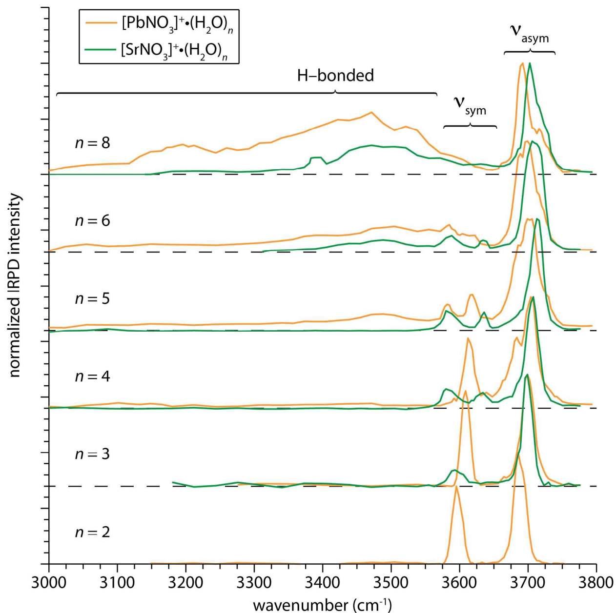
Figure 1. IRPD spectra of [\text{PbNO}_3]^+(\text{H}_2\text{O})_{2-6,8} and [\text{SrNO}_3]^+(\text{H}_2\text{O})_{3-6,8} measured at 133 K.
