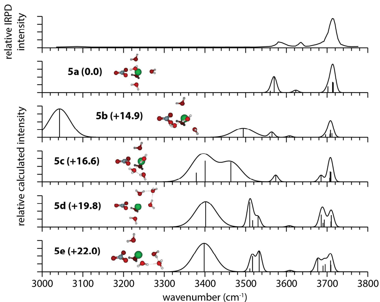
Figure 5. IRPD spectrum of [\text{SrNO}_3]^+(\text{H}_2\text{O})_5 and calculated spectra of low-energy isomers at the B3LYP/aug-cc-pVDZ level of theory, along with their relative Gibbs free energies in kJ/mol at 133 K.
