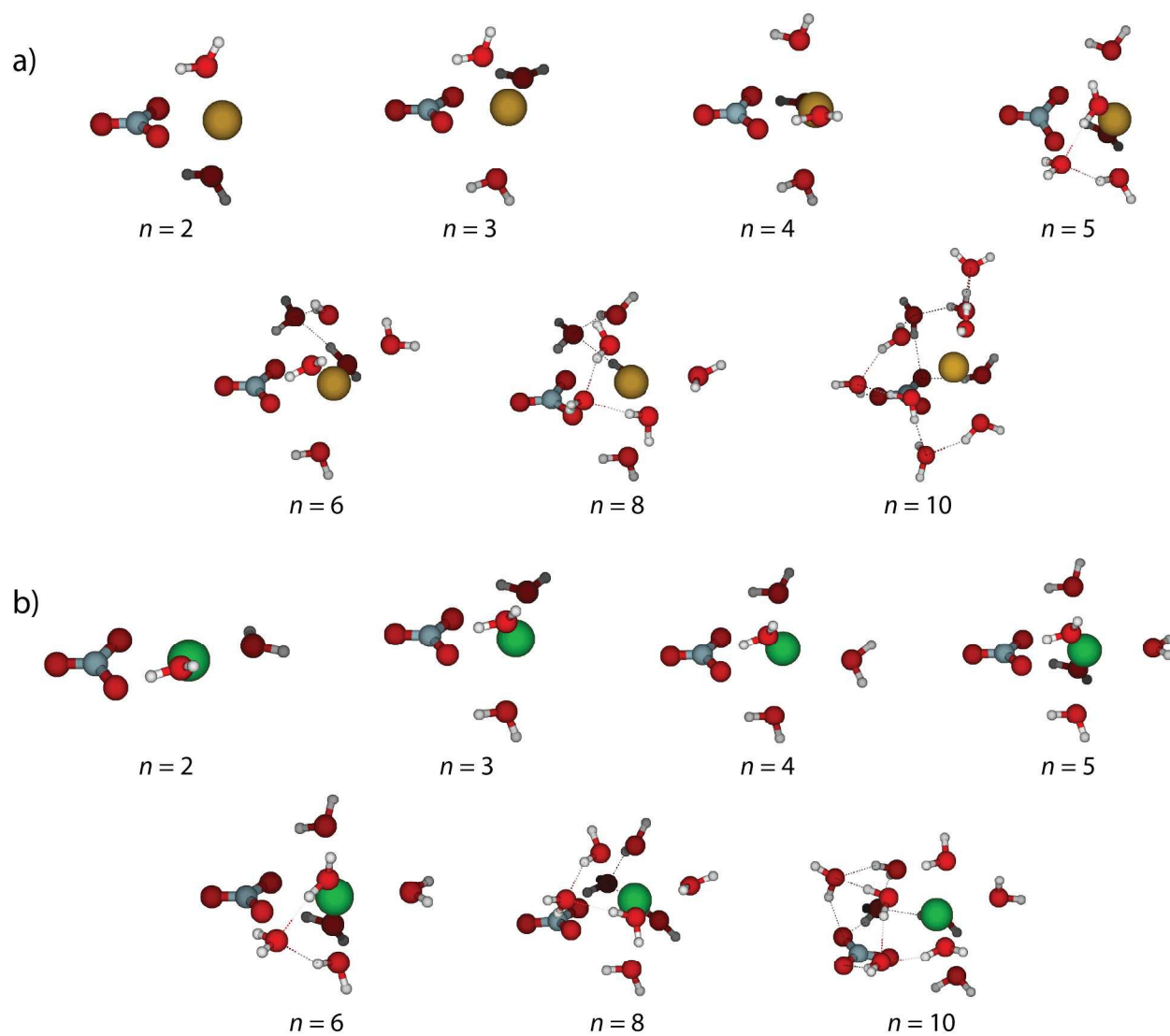
Figure 2. (a) Calculated lowest-energy structures at 133K of (a) [\text{PbNO}_3]^+(\text{H}_2\text{O})_{2-6,8,10} and (b) [\text{SrNO}_3]^+(\text{H}_2\text{O})_{2-6,8,10} at the B3LYP/aug-cc-pVDZ level of theory.
