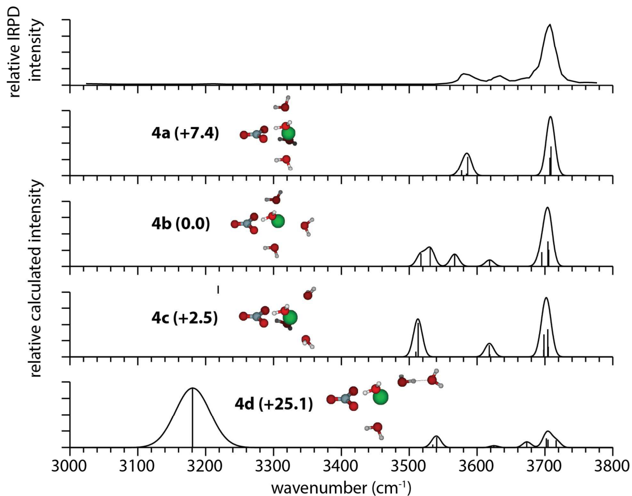
Figure 3. IRPD spectrum of [\text{SrNO}_3]^+(\text{H}_2\text{O})_4 and calculated spectra of low-energy isomers at the B3LYP/aug-cc-pVDZ level of theory, along with their relative Gibbs free energies in \text{kJ/mol} at 133 K.
