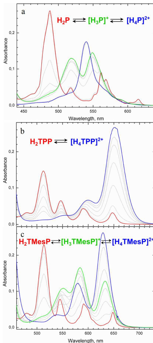
Figure 1: Ground-state absorption spectra of the free base, mono- and diprotonated species (red, green and blue colors, respectively). Panels from top to bottom: porphine ( H_2P , [H_3P]^+ , [H_4P]^{2+} ), tetra- meso -phenylporphyrin ( H_2TPP , [H_4TPP]^{2+} ), and tetra- meso -mesitylporphyrin ( H_2TMesP , [H_3TMesP]^+ , [H_4TMesP]^{2+} ).
