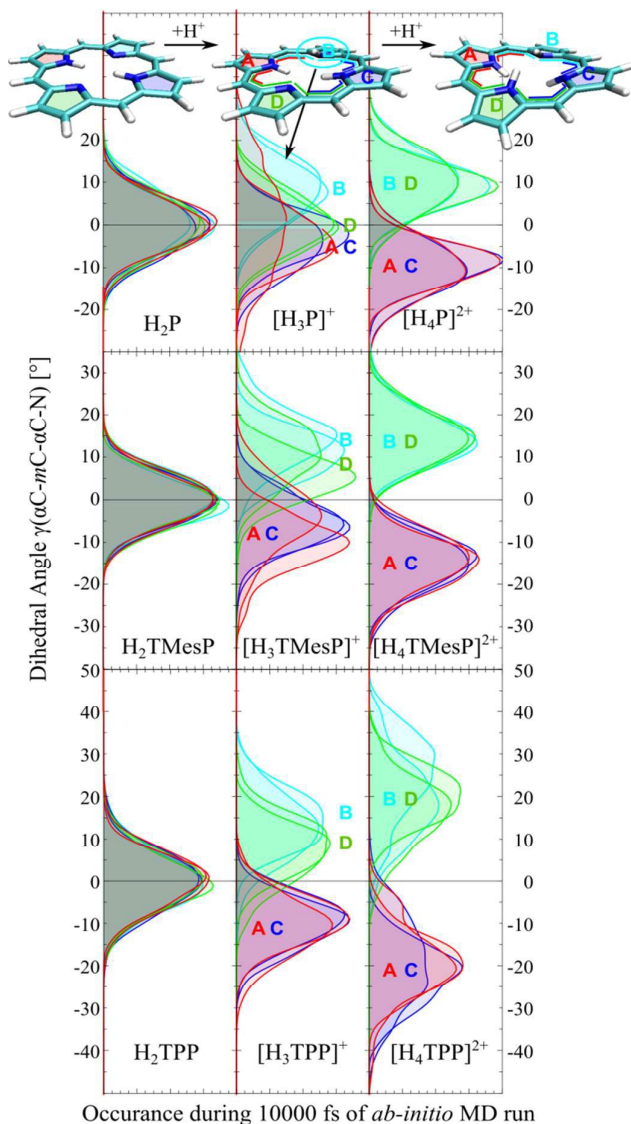
Figure 2: Histograms of dihedral angles \theta^N , which quantify the oop -distortion and are determined by the flexibility of the macrocycle. For each pyrrole two dihedral angles involving the same nitrogen, but \alpha -, meso -, and next \alpha -carbons in opposing directions can be defined, as indicated in the protonated structures at the top of the figure. Thus, two identically colored lines represent the smoothed histograms these two dihedral angles.
