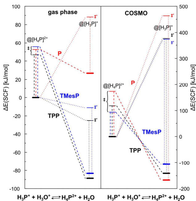
Figure 3: Energies of geometry-optimized mono- and diprotonated species as well as states with geometries matching those of the neighboring protonation state. † labels: Mono-protonated species that are distorted to match the geometries of their diprotonated forms (via removing one proton from the diprotonated forms). ‡ labels: Diprotonated species that are distorted to match the geometries of their mono-protonated forms (via constraint geometry optimization after adding a proton to the mono-protonated forms).
