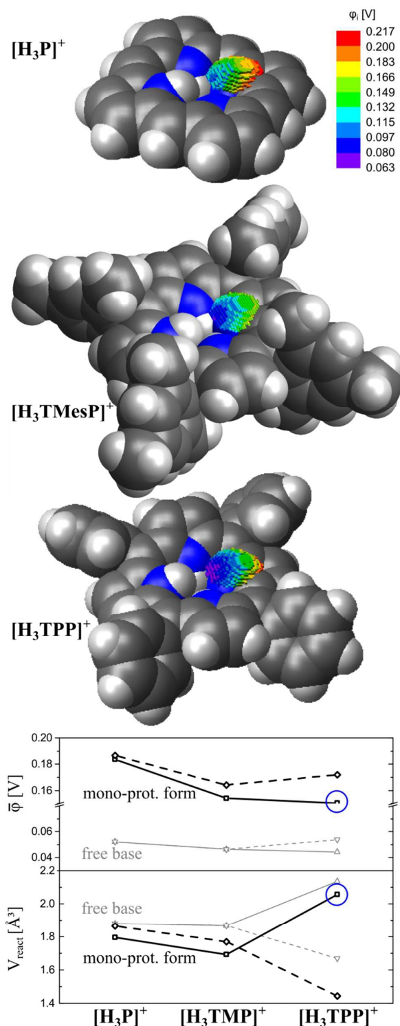
Figure 5: Van der Waals surface representations of the mono-protonated species [\text{H}_3\text{P}]^+ , [\text{H}_3\text{TMesP}]^+ , [\text{H}_3\text{TPP}]^+ together with voxels that represent the reactivity volumes V_{\text{react}} . The color coding of the voxels corresponds to the electrostatic potential in the center of each voxel. Color coding of atoms: White, Gray, Blue – H, C, N. Reactivity volumes V_{\text{react}} with their associated mean
