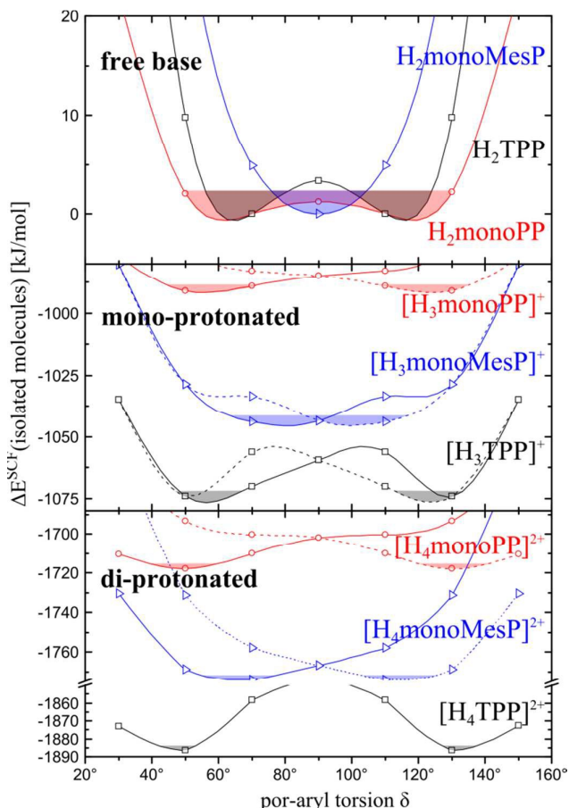
Figure 4: Torsional profiles of mono- meso -substituted porphyrins. The influence of the different meso -substituents (phenyl, P, and mesityl, Mes) on the SCF energy upon torsion against the porphyrin in the model compounds \text{H}_2\text{monoPP} and \text{H}_2\text{monoMesP} and their mono- and diprotonated forms is compared. The torsional profiles of the mono-protonated species refer to protonation of the pyrrole that is closest to the meso -substituent. The dashed graphs are mirrored representatives of the continuous line graphs. Both are asymmetric for the protonated species since the pyrrole oop -twist is different for the two pyrroles
