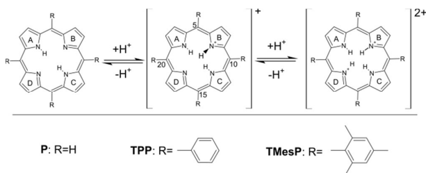
Scheme 1: Acid-base-equilibria of different porphyrin derivatives. Carbon atoms 5, 10, 15, 20 are the meso -carbons.
