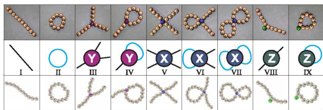
Fig. 1 An overview of all the basic units we consider in three different representations. Top row: photographs of commercially available magnetic beads; middle row: topological classification used in the proposed theoretical approach, here in lack we indicate chain segments and in blue – rings; bottom row: structures extracted from Monte Carlo computer simulations analysed in this manuscript. From left to right: (I) a linear chain of regular particles; (II) a ring of regular particles; (III) three linear chains of regular particles connected by one Y defect; (IV) one linear chain and one ring of regular particles connected by a Y defect; (V) four linear chains of regular particles connected by one X defect; (VI) one X defect connecting one ring and two chains of regular particles; (VII) one X defect joining two rings of regular particles; (VIII) a linear chain with an internal Z defect; (IX) a ring with an internal Z defect.
