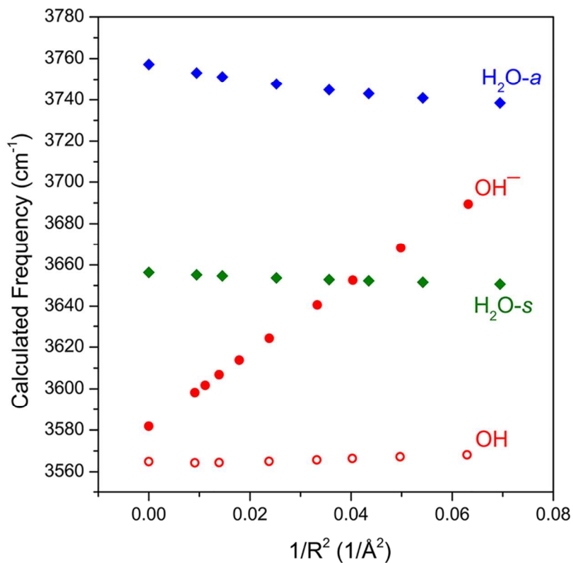
Figure 5. The calculated (CCSD/aug-cc-pVTZ) vibrational frequencies of \text{OH}^- , \text{OH} , and symmetric/antisymmetric \text{H}_2\text{O} at various distances from a point charge ( +1e ). The harmonic frequencies are scaled by 0.949.
