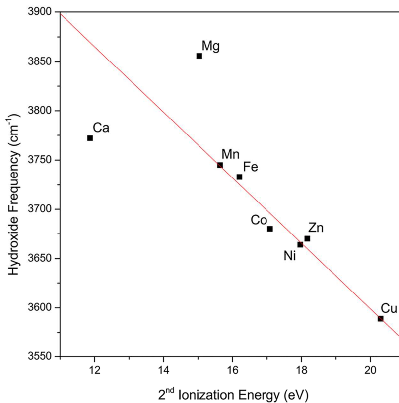
Figure 3. Experimental hydroxide vibrational frequency in the \text{MOH}(\text{H}_2\text{O})^+\cdot\text{D}_2 complexes as a function of the 2 nd ionization energy of the bare metal. The experimental values for the hydroxide frequency of the Mg and Ca complexes are obtained from ref. 17. The red line is a linear fit of the data points excluding the Mg and Ca values.
