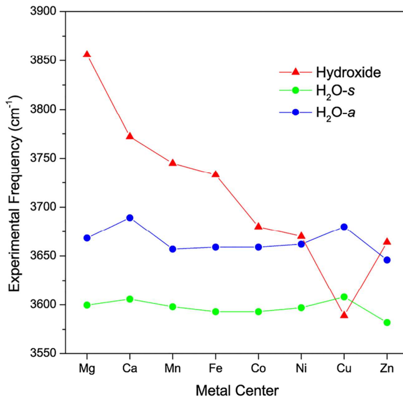
Figure 2. Experimental vibrational frequencies of the \text{MOH}(\text{H}_2\text{O})^+\cdot\text{D}_2 complexes as a function of the metal species. The values for the Mg and Ca complexes are obtained from ref. 17.
