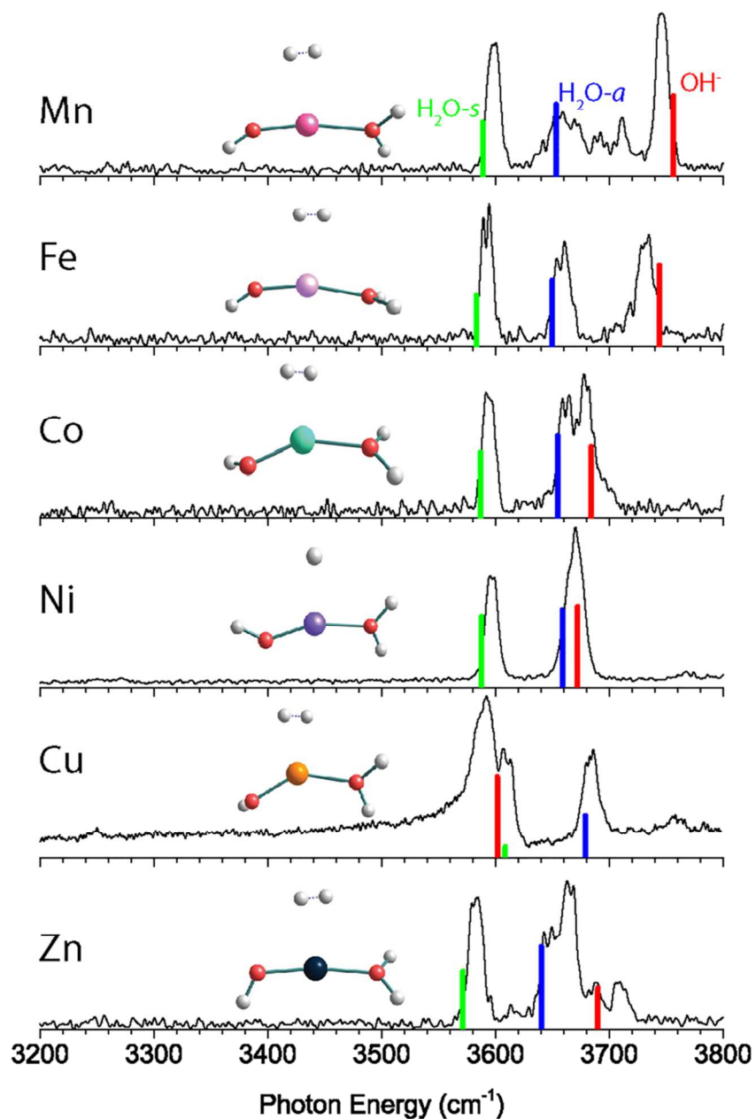
Figure 1. Experimental vibrational predissociation spectra and calculated (cam-B3LYP/def2TZVP) harmonic infrared spectra of the MOH(H 2 O) + ·D 2 (M=Mn, Fe, Co, Ni, Cu, Zn) complexes. H 2 O-s: H 2 O symmetric stretch; H 2 O-a: H 2 O antisymmetric stretch; OH - : hydroxide stretch.
