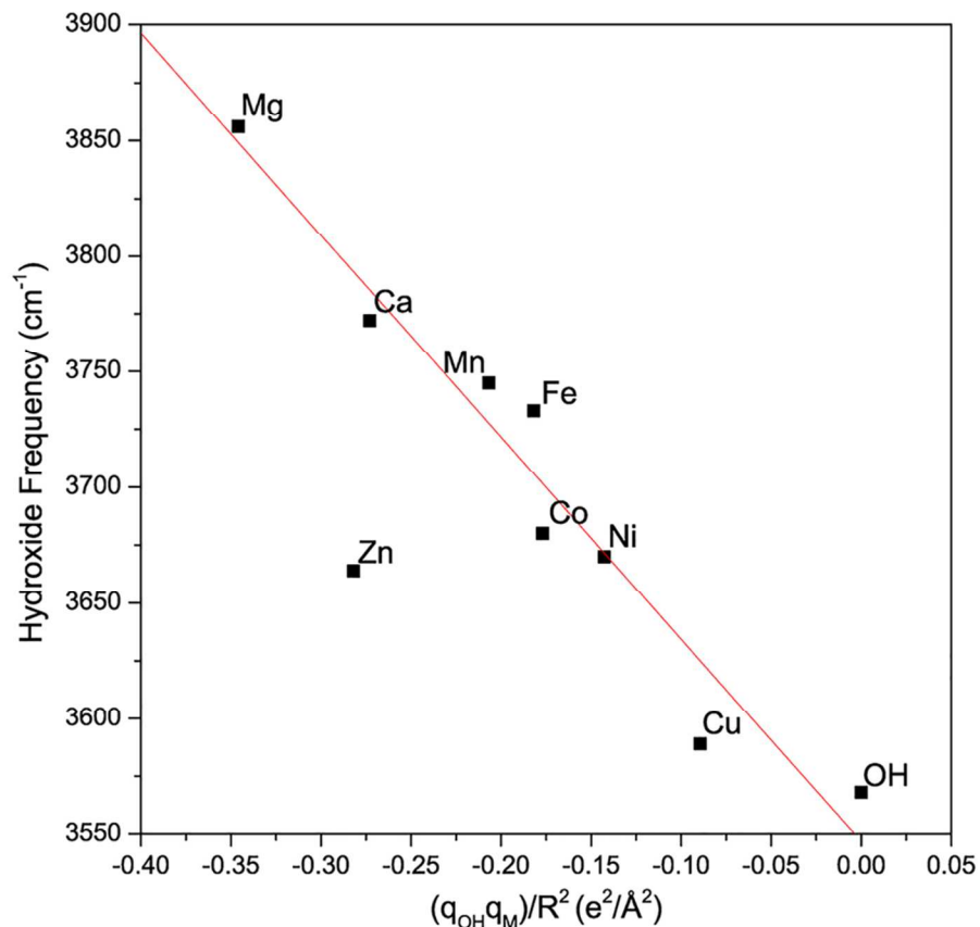
Figure 6. The experimental hydroxide frequency as a function of the field induced by the metal center ( q_M/R^2 ) multiplied by the charge present on the hydroxide ( q_{OH} ). The gas phase vibrational frequency of the hydroxyl radical is also included. The experimental values for the hydroxide frequency of the Mg and Ca complexes are obtained from ref. 17. The red line is a linear fit of the data points excluding the Zn complex.
