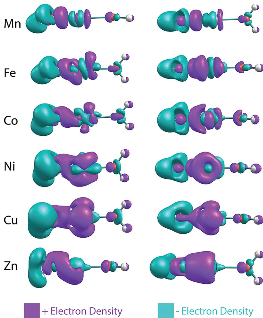
Figure 4. SCF electron density difference map of the MOH(H 2 O) + complexes. The contour isovalue is 0.007. The difference map is obtained by subtracting the SCF densities of the individual OH - and [M-OH 2 ] 2+ fragments from the entire MOH(H 2 O) + complex.
