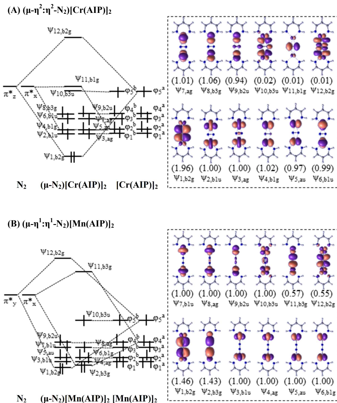
Figure 4. Schematic orbital interaction diagrams of (A) (\mu\text{-}\eta^2:\eta^2\text{-N}_2)[\text{Cr}(\text{AIP})]_2 and (B) (\mu\text{-}\eta^1:\eta^1\text{-N}_2)[\text{Mn}(\text{AIP})]_2 . In dashed line are natural orbitals with occupation numbers.
