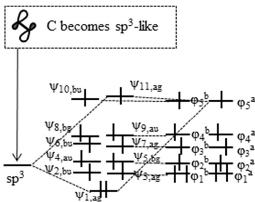
\text{C}_2\text{H}_4 (\mu\text{-C}_2\text{H}_4)[\text{Mn}(\text{AIP})]_2 [\text{Mn}(\text{AIP})]_2
