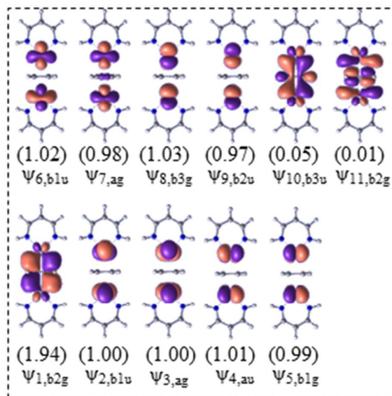
\text{C}_2\text{H}_4 (\mu\text{-C}_2\text{H}_4)[\text{Cr}(\text{AIP})]_2 [\text{Cr}(\text{AIP})]_2
