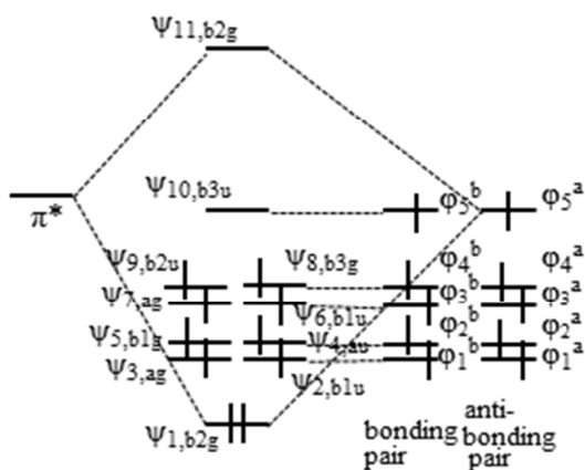
\text{C}_2\text{H}_4 (\mu\text{-C}_2\text{H}_4)[\text{Cr}(\text{AIP})]_2 [\text{Cr}(\text{AIP})]_2
