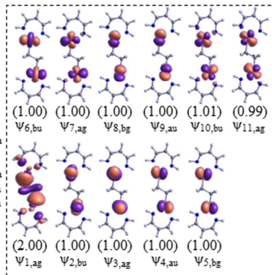
Figure 3. Schematic orbital interaction diagrams of (A) (\mu\text{-}\eta^2:\eta^2\text{-C}_2\text{H}_4)[\text{Cr}(\text{AIP})]_2 and (B) (\mu\text{-}\eta^1:\eta^1\text{-C}_2\text{H}_4)[\text{Mn}(\text{AIP})]_2 . In dashed line are natural orbitals with occupation numbers.
