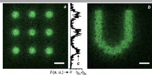
Fig. 6 Confocal laser-scanning fluorescence images ( a and b , \lambda_{\text{Ex}} = 405 nm, \lambda_{\text{Em}} = 430 – 650 nm, scale bar = 30 \mu\text{m} ) of PBMA films, doped with 1 (3% w/w) and deposited on glass slides with silver nanoparticles on their surface, recorded after illumination ( \lambda_{\text{Ac}} = 405 nm, 0.1 mW, 300 s) of defined areas within the imaging field. Profile of the emission intensity ( c ) measured across some of the activated areas in a .
