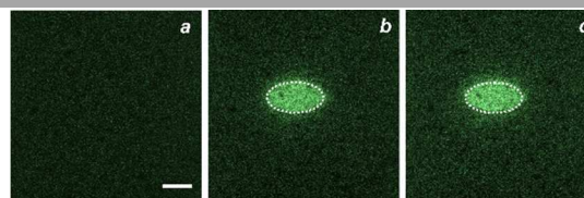
Fig. 4 Confocal laser-scanning fluorescence images ( \lambda_{\text{Ex}} = 405 nm, \lambda_{\text{Em}} = 430 – 650 nm, scale bar = 30 \mu\text{m} ) of a PBMA film, doped with 1 (3% w/w) and deposited on a glass slide with silver nanoparticles on its surface, recorded before ( a ), immediately ( b ) and 10 min ( c ) after illumination ( \lambda_{\text{Ac}} = 405 nm, 0.1 mW, 90 s) of an ellipsoidal area within the imaging field.
