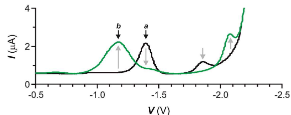
Fig. 3 Square wave voltammograms [ 50 \text{ mV s}^{-1} , V vs. \text{Ag}/\text{Ag}^+ (1 mM in \text{AgNO}_3 ), \text{Bu}_4\text{NPF}_6 (50 mM)] of a MeCN solution of 1 (100 \mu\text{M} , 20 ^{\circ}\text{C} ) before ( a ) and after ( b ) illumination ( \lambda_{\text{AC}} = 350 nm, 4.88 \text{mW cm}^{-2} , 10 min).
