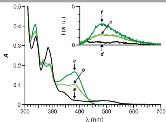
Fig. 2 Absorption ( a–c ) and emission ( d–f , \lambda_{\text{EX}} = 380 nm) spectra of MeCN solutions (10 \mu\text{M} , 20 ^{\circ}\text{C} ) of 1 , before ( a and d ) and after ( b and e ) irradiation ( \lambda_{\text{AC}} = 350 nm, 4.88 \text{mW cm}^{-2} , 10 min), and of 2 ( c and f ).
