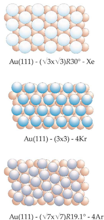
Figure 2: Adsorption geometry for xenon, krypton and argon on a Au(111) surface. Due to the lack of experimental data we assume the argon and krypton adsorption geometry on Au(111) to be similar to the adsorption geometry on similar close-packed transition metal surfaces.
