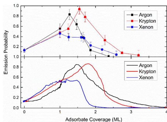
Figure 4: The upper panel shows the electron emission probability versus adsorbate coverage for argon, krypton, and xenon. Lines are added to guide the eye. Error bars are applied reflecting the uncertainty associated with multiple measurements of monolayer enhancement as presented in
