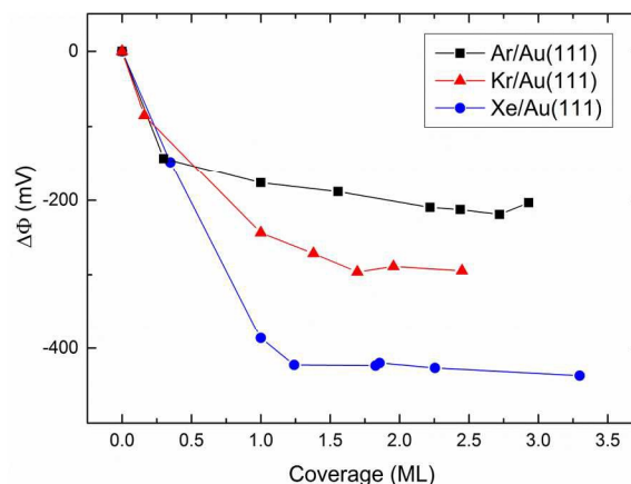
Figure 5: Work function change of the Au(111) surface due to the adsorption of rare gas. The work function drops strongly with the adsorption of one monolayer. The effect of any further adsorbed gas is minor. Lines are added to guide the eye.
