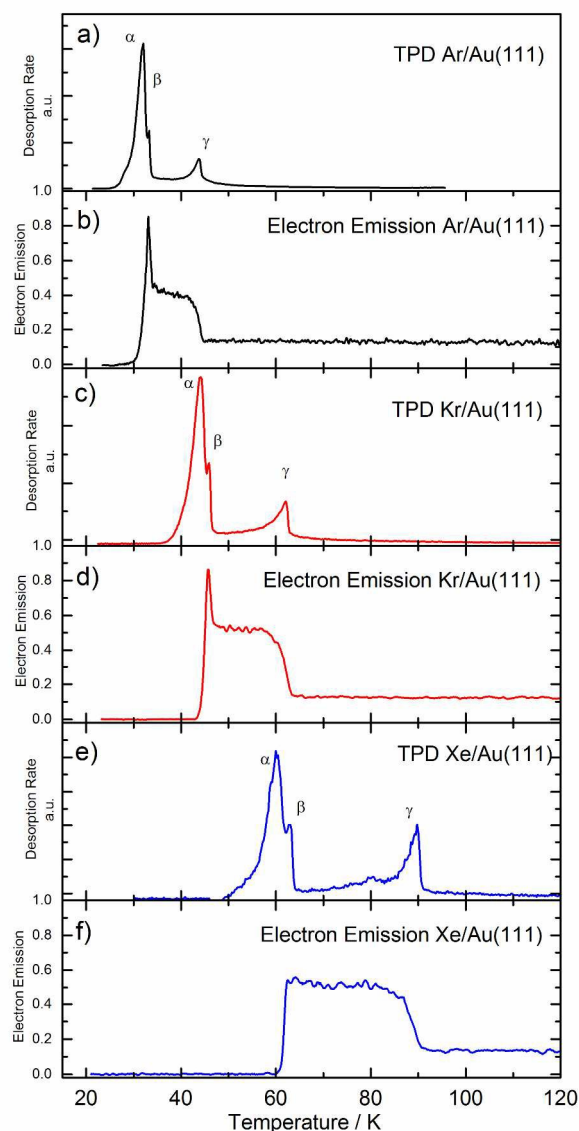
Figure 3: TPDs (a, c, e) and electron emission curves (b, d, f) for Ar, Kr and Xe adsorbed on a Au(111) surface. During all scans the heating rate was 10 K/min and the initial coverages > 5 ML for Ar/Au(111), Kr/Au(111) and Xe/Au(111), respectively. For all TPDs, \alpha indicates the overlayer peak, \beta the bilayer peak and \gamma the
