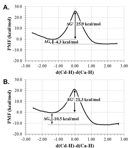
Figure 1. Free energy profiles for the hydride transfer step of the TSase catalyzed reaction, obtained as mono-dimensional AM1/MM potential of mean force (1D- PMF) using two different initial X-ray structure 2TSC (top) and 1TLS (bottom), at 303 K. The distinguished reaction coordinate (in Å)
