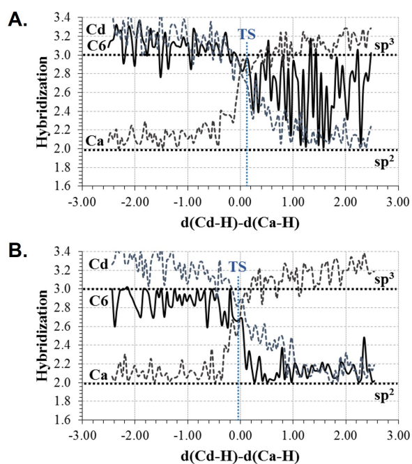
Figure 6. Evolution of the hybridization states of the hydride donor carbon (Cd) and hydride acceptor carbon (Ca), in dashed lines, and the carbon atom involved in the C6(dUMP)-S(Cys146) breaking bond (solid lines) along the reaction coordinate (in Å). Results from stepwise (A) and concerted (B) mechanisms derived from the corresponding 1D PMFs performed at 303 K. Hybridization value of 2 on the carbon atom corresponds to a sp^2 molecule, while a value of 3 represents a sp^3 hybridization. Position of the TSs are indicated as a dotted vertical blue lines.
