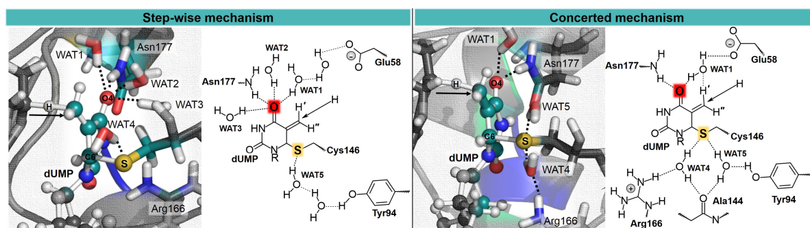
Figure 3. Representative snapshots of the averaged structures of reactants state obtained from the 1D PMFs generated from the A) step-wise mechanisms (1D PMFs generated from 2TSC) and B) concerted mechanisms (1D PMFs generated from 1TLS).
