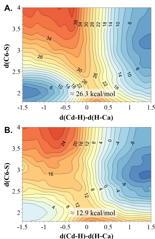
Figure 5. M06-2X/MM 2D PMF performed at 303 K using two different initial X-ray structure 2TSC (A) and 1TLS (B). The distinguished reaction coordinates (in Å) are the C6(dUMP)-S(Cys146) distance and the antisymmetric combination of the breaking and forming bonds of the transferred hydrogen atom, d(\text{Cd-H}) - d(\text{Ca-H}) . Values on isoenergetic lines are reported in \text{kcal} \cdot \text{mol}^{-1} .
