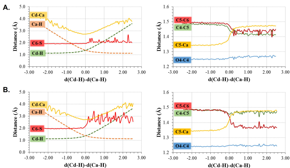
Figure 2. Evolution of key distances along the distinguished reaction coordinate (in Å) computed as averages over the different windows generated along the A) step-wise mechanisms (1D PMFs generated from 2TSC) and B) concerted mechanisms (1D PMFs generated from 1TLS).
