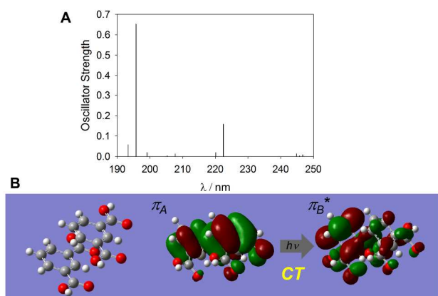
Fig. 9 (A) The absorption spectrum calculated for an IPA dimer indicating a CT-like photoexcitation of isophthalic acid, \pi_A - \pi_B^* transition at 222 nm with an oscillator strength of 0.158, by TD-DFT calculation on CAM-B3LYP at the 631Gd level with Gaussian 09. (B) The dimer structure (left) taken from the BENZDC10 file provided in Cambridge Structural DS 2013 and the molecular orbitals for the RIP dimers, \pi_A (middle) and \pi_B^* (right).
