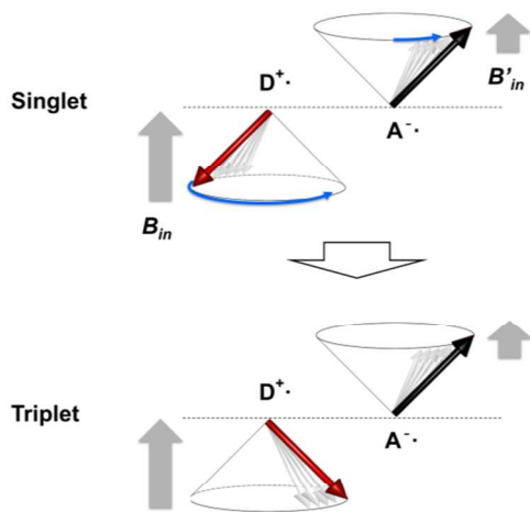
Fig. 4 A spin exchange mechanism by electron spin precessions in an RIP consisted of an electron-donating radical cation ( D^{\cdot+} ) and an electron-accepting radical anion ( A^{\cdot-} ). The two spins are under different internal magnetic fields ( B_{in} and B'_{in} ), which causes different precession rates. The faster spin ( D^{\cdot+} ) in the singlet state catches up the slower spin ( A^{\cdot-} ) in due course to produce a triplet state.
