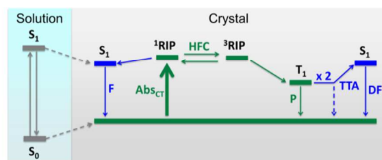
Fig. 10 A state energy diagram for IPA phosphorescence. Green color shows a route to phosphorescence emission and blue color shows a route to fluorescence and delayed fluorescence. Abs CT : CT absorption, P: Phosphorescence, TTA: Triplet-triplet annihilation, DF: Delayed fluorescence, HFC: Hyperfine coupling.
