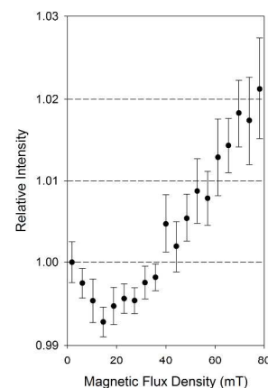
Fig. 5 Magnetic-field effects on the phosphorescence intensity at 500 nm of IPA. IPA was excited at 308 nm under external magnetic field from an electromagnet connected to a constant voltage supply with the voltage variation between 0 and 90 V. The data represent the mean value from nine experiments and the error bars are \pm s.e.m.
