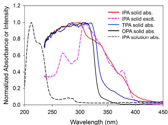
Fig. 8 Absorption spectra of IPA, TPA, and OPA solids and IPA solution in methanol, and phosphorescence excitation spectrum with the emission at 501 nm. CT absorptions are observed for IPA and TPA between 340 and 400 nm.
