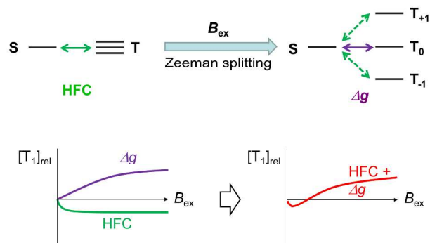
Fig. 6 HFC and \Delta g magnetic field effects on the phosphorescence of IPA. Without external magnetic fields ( B_{\text{ex}}=0 ), S-T spin conversions are mediated by the internal magnetic field ( B_{\text{in}} ) generated from nuclear spins (HFC). An external magnetic field ( B_{\text{ex}} ) suppresses the S- T_{+1} and S- T_{-1} spin exchanges (HFC) due to Zeeman splitting, giving a downward saturation curve. The S- T_0 spin exchange is enhanced with increasing B_{\text{ex}} by \Delta g effect, where the difference of Larmor frequency between two electron spins is amplified by B_{\text{ex}} , giving a rising curve overriding the downward curve of HFC. [T_1]_{\text{rel}} denotes the relative concentration of T_1 . Here, S, T_0 , and T_{\pm 1} denote RIPs as precursors of triplet exciton T.
