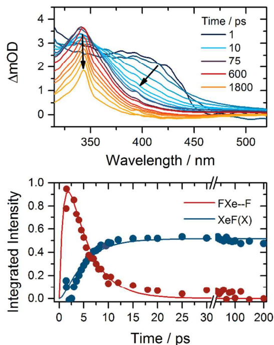
Figure 1. Top: time-resolved electronic absorption spectra of \text{XeF}_2 / \text{CH}_3\text{CN} solutions
