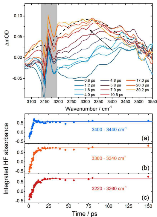
Figure 3. Top: time-resolved IR spectra of HF from the reaction of F atoms with CH_3CN . The dashed black line is a steady-state FTIR spectrum of HF in acetonitrile, and the feature masked by the grey shading is a solvent interference. The inset key shows the time delays at which spectra were obtained. Bottom: time-dependence of HF absorbance summed over three wavenumber intervals, (a) 3400 – 3440 cm^{-1} , (b) 3300 – 3340 cm^{-1} and (c) 3220 – 3260 cm^{-1} . Solid lines are single exponential fits.
