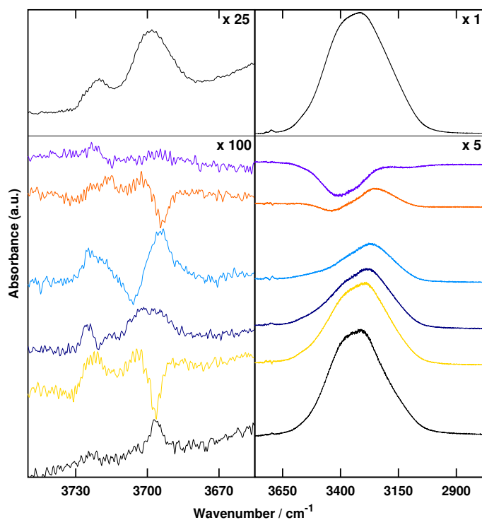
Fig. 3 Selective irradiations at irregular frequency “jumps” within the dH bands. Upper panels: dH bands (on the left), and bulk component (on the right) of an unirradiated ASW sample. Lower panels: dH bands (left), and bulk component (right) difference spectra after irradiation at the frequency indicated by an arrow (for irradiation n - (n-1) ). Irradiation duration at each frequency: 30 min. From top to bottom: irradiation at i. 3715 \text{cm}^{-1} (indigo, P_{\text{laser}}=37 mW); ii. 3690 \text{cm}^{-1} (orange, P_{\text{laser}}=42 mW); iii. 3705 \text{cm}^{-1} (light blue, P_{\text{laser}}=35 mW); iv. 3720 \text{cm}^{-1} (violet, P_{\text{laser}}=22 mW); v. 3695 \text{cm}^{-1} (yellow, P_{\text{laser}}=47 mW); vi. 3725 \text{cm}^{-1} (black, P_{\text{laser}}=22 mW). Spectra are multiplied by the factor in the top right-hand corner of each panel.
