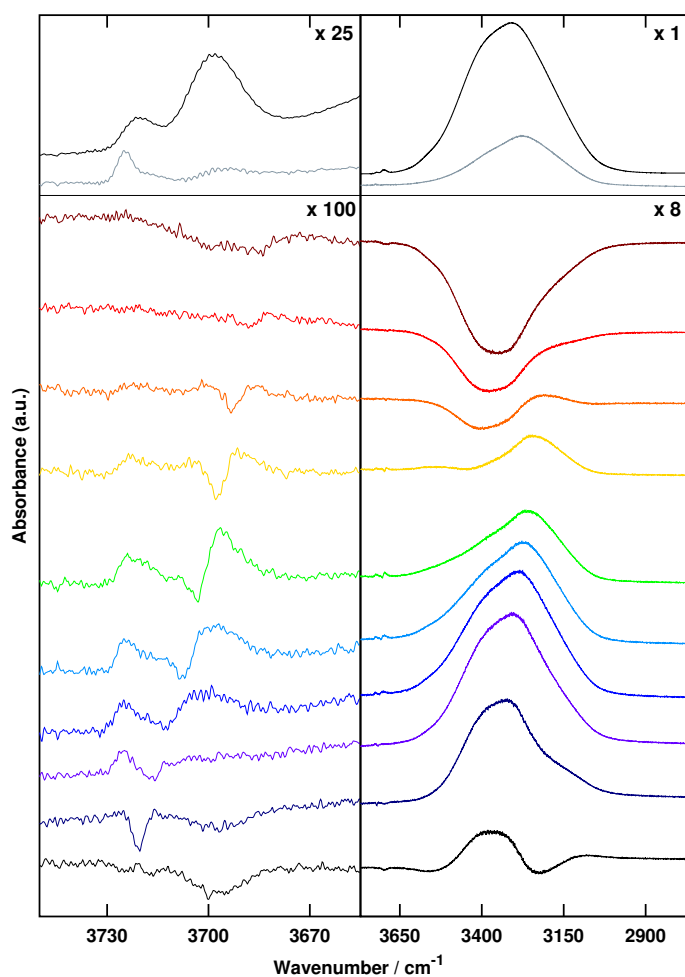
Fig. 2 Series of selective irradiations of the dH bands, from “red to blue”. Upper panels: dH bands (on the left), and bulk component (on the right) of an unirradiated ASW sample (black) and the overall difference spectrum after 10 irradiations (grey). Lower panels: dH bands (left), and bulk component (right) difference spectra after irradiation at the frequency indicated by an arrow (for irradiation n - (n-1) ). Irradiation duration at each frequency: 30 min. From top to bottom: irradiations at i. 3680\text{ cm}^{-1} (brown, P_{\text{laser}}=33\text{ mW} ); ii. 3685\text{ cm}^{-1} (red, P_{\text{laser}}=29\text{ mW} ); iii. 3690\text{ cm}^{-1} (orange, P_{\text{laser}}=34\text{ mW} ); iv. 3695\text{ cm}^{-1} (yellow, P_{\text{laser}}=36\text{ mW} ); v. 3700\text{ cm}^{-1} (green, P_{\text{laser}}=36\text{ mW} ); vi. 3705\text{ cm}^{-1} (light blue, P_{\text{laser}}=36\text{ mW} ); vii. 3710\text{ cm}^{-1} (dark blue, P_{\text{laser}}=29\text{ mW} ); viii. 3715\text{ cm}^{-1} (indigo, P_{\text{laser}}=47\text{ mW} ); ix. 3720\text{ cm}^{-1} (violet, P_{\text{laser}}=36\text{ mW} ); x. 3725\text{ cm}^{-1} (black, P_{\text{laser}}=32\text{ mW} ). Spectra are multiplied by the factor in the top right-hand corner of each panel.
