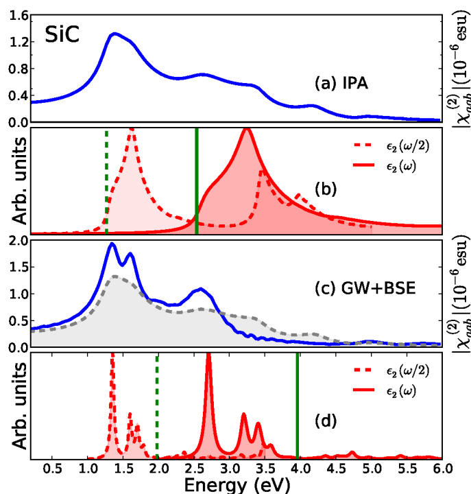
Fig. 2 [Color online] Optical absorption and SHG in SiC. Panels (a) and (c): |\chi_{aab}^{(2)}(\omega)| respectively at the IP (Eq. (6)) and GW +BSE level (Eq. (7)). For a direct comparison the IP spectrum is also shown in panel (c) in gray dashed line. Panels (b) and (d) shows the optical absorption calculated at \omega/2 for both the IP and GW +BSE level of approximation. The green continuous vertical line represents the calculated minimum direct gaps within KS [(b)] and G_0W_0 [(d)] approaches. The dashed green vertical line corresponds to half the minimum gap.
