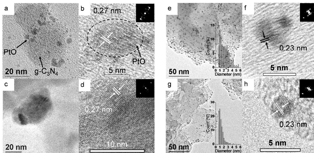
Fig. 3 TEM (a, c, e, g) and HRTEM (b, d, f, h) images of different Pt-g-C 3 N 4 samples before (a-d) and after (e-h) photocatalytic process. Images of platinum a, b) impregnated on g-C 3 N 4 and c, d) after calcination treatment. Images of e, f) impregnated and g, h) photodeposited Pt-g-C 3 N 4 after 20 hours of visible irradiation. Insets e and g: statistical nanoparticle size distribution.
