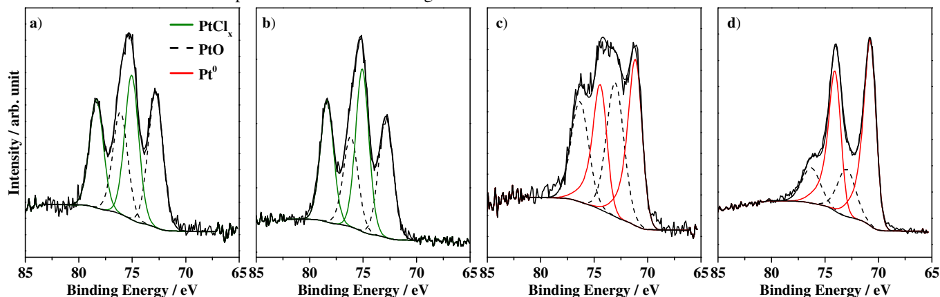
Fig. 2 XP spectra of the Pt 4f region for Pt-g-C 3 N 4 a) impregnated and b) calcined before photocatalysis; c) impregnated and d) photodeposited after photocatalysis.
