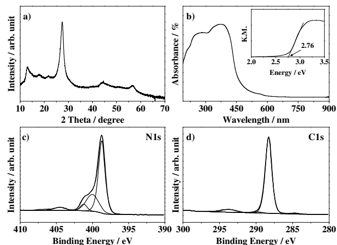
Fig. 1 a) XRD pattern, b) UV-Vis absorbance spectrum (inset: Kubelka-Munk), c) XPS N1s and d) C1s spectra of \text{g-C}_3\text{N}_4 .
