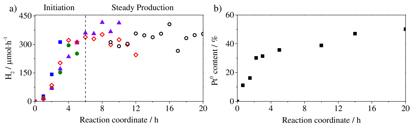
Fig. 4 (a) H 2 evolution rate (μmol·h -1 ) of five different experiments: ■) 3 hours, ●) 5 hours, ▲) 10 hours, ◇) 12 hours, ○) final 10 hours. Test conditions: 0.2 g of catalyst in 0.2 L of 0.025 M aqueous solution of oxalic acid, visible light ( \lambda \geq 420 nm). (b) Pt 0 % of total platinum content on Pt-g-C 3 N 4 as obtained from XPS analysis (for XP spectra see Fig. S3).
