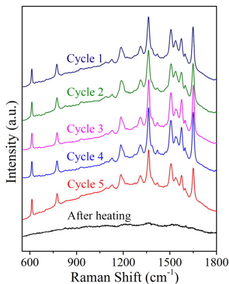
Figure 5. Raman spectra of R6G ( 10^{-6} M) on a SERS substrate of Au decorated 1L BN after five cycles of reusability test. A typical Raman spectrum after heating at 400 °C to remove the adsorbed R6G is also shown for comparison. All the spectra were acquired under the same conditions.
