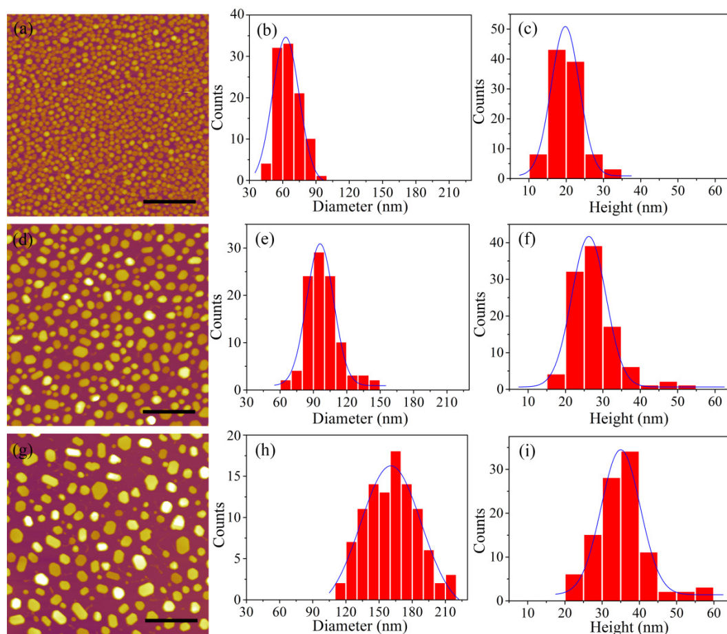
Figure 2. (a), (d) and (g) AFM images showing the size and distribution of Au particles on BN using different sputtering time (20, 30 and 40 s, respectively); (b), (e) and (h) statistic of the AFM-derived particle diameter and corresponding Gaussian fits on the distribution; (c), (f) and (i) statistic of particle height and corresponding fits. All scale bars are 500 nm.
