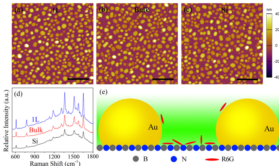
Figure 4. AFM images of Au particles on (a) monolayer BN, (b) bulk BN and (c) SiO 2 /Si substrate, respectively. The scale bars are 500 nm. (d) Raman spectra of R6G on the three SERS substrates; (e) a diagram illustrating that R6G molecules are adsorbed on a monolayer BN, which can improve the SERS enhancement.
