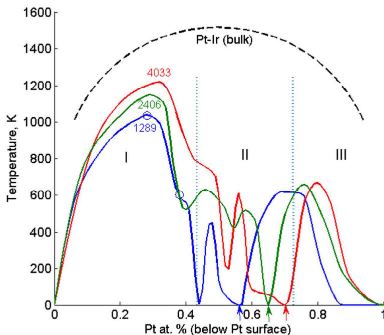
Fig.7. Nanophase diagram of symmetry-breaking transitions in Pt-Ir TO NPs (with marked sizes) computed by the CGLM-FCEM. The left (I) and right (III) domes correspond to inner-core quasi-Janus and subsurface quasi ball-and-cup transitions to multi-shell configurations, respectively. The intermediate region (II) involves ideal multi-shell (no transitions) at “magic compositions” indicated by arrows (Pt-surface@Ir-subsurface@Pt-inner-core). The transitions presented in Figs. 4 and 5 are marked by small circles on the separation-coexistence dome of the 1289-atom TO. FCEM-computed bulk diagram miscibility gap is shown for comparison.
