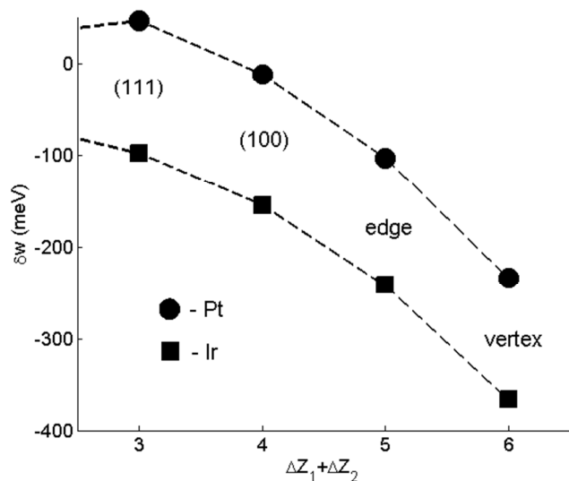
Fig.2. The dependence of surface-subsurface bond-energy variations, \delta w , on the number of pair broken bonds, \Delta Z_1 + \Delta Z_2 , as extracted from DFT-computed surface energies (bulk bond energies are: w_b^{Pt} = -1.160 eV, w_b^{Ir} = -1.635 eV).
