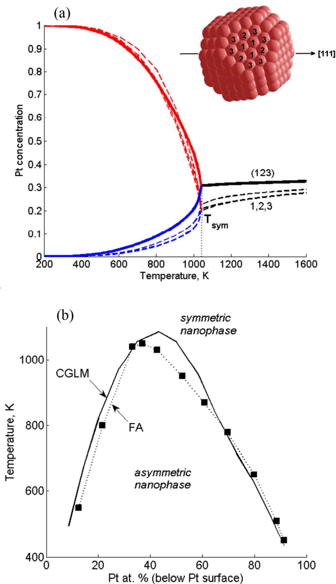
Fig.3. Verification of the coarse-grained layer model (CGLM): Asymmetric-symmetric transitions along the [111] axis in Pt 376 Ir 210 TOs computed with the CGLM-FCEM vs. the fully-atomistic (FA)-FCEM. (a) Three distinct subsurface site concentrations (thin dashed lines) vs. one subsurface layer concentration computed using the CGLM (thick solid lines). Below the transition at T_{sym} , Pt-side - red, Ir-side - blue. The site positions are marked in the subsurface schematics (inset); (b) Nanophase diagram computed in the CGLM (thick solid line), compared to the diagram obtained by the FA computation 11 (■ - magic-number compositions).
