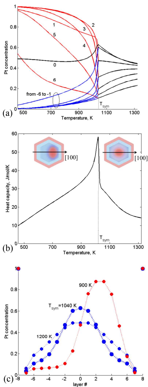
Fig.4. CGLM-FCEM computation results for 1289-atom TO with 28 at. % Pt core: (a) Thermally-induced variations of the Pt-side (red) and Ir-side (blue) inner core layer concentrations, which coincide (black) at the transition temperature T_{sym} . Inset: schematics of asymmetric (quasi-Janus) and symmetric (multi-shell) configurations below and above T_{sym} . (b) The corresponding configurational heat-capacity \lambda -peak. (c) Layer concentration profiles for T < T_{sym} , T = T_{sym} and T > T_{sym} . Layer numbering corresponds to Fig.1.
