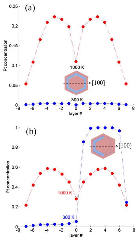
Fig.6. Subsurface layer concentration profiles computed for 1289-atom TO. (a) Magic composition ( \sim 57 at. % Pt core): multi-shell structure without a transition; (b) \sim 75 at. % Pt core: asymmetric quasi ball-and-(subsurface)-cup at 300 K and symmetric profile at 1000 K. Layer numbering corresponds to Fig.1.
