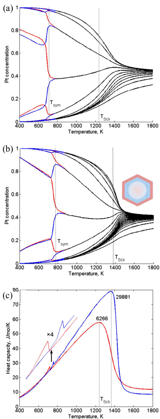
Fig.8. Variations with temperature of the inner core layer concentrations in 6266-atom (a) and 29881-atom (b) TOs (37 at. % Pt core); (c) Heat-capacity Schottky humps corresponding to the indicated TO sizes. The weak features around 700 K correspond to symmetry-breaking transitions accompanied by nanophase boundary small shifts.
