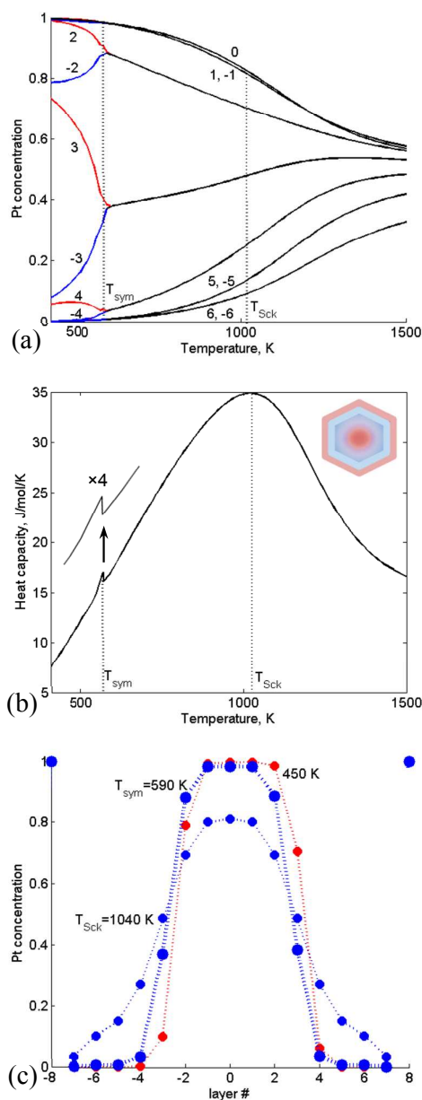
Fig.5. CGLM-FCEM results for 1289-atom TO with 38 at. % Pt core (along the [100] axis): (a) Thermally-induced variations of the Pt-side (red) and Ir-side (blue) inner core layer concentrations, which coincide (black) at the transition temperature T_{sym} . (b) The corresponding configurational heat-capacity Schottky hump with maximum at T_{Sck} \gg T_{sym} and a weak sharp feature related to the symmetry-breaking minor transition. Inset: schematics of a symmetric (multi-shell) configuration above T_{sym} . (c) Layer concentration profiles for T < T_{sym} , T = T_{sym} and T > T_{sym} . Layer numbering corresponds to Fig.1.
