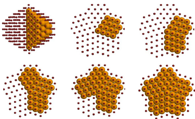
Fig. 6 The shape of the nickel core for clusters of the decahedral structure for five magic numbers corresponding to the filling of the five “slices”. Ni atoms are shown as large gold spheres, copper as small red spheres.
