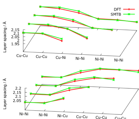
Fig. 1 Surface relaxation in the z -direction for: a) 1-to-4 nickel layers over bulk copper, b) 1-to-4 copper layers over bulk nickel.
