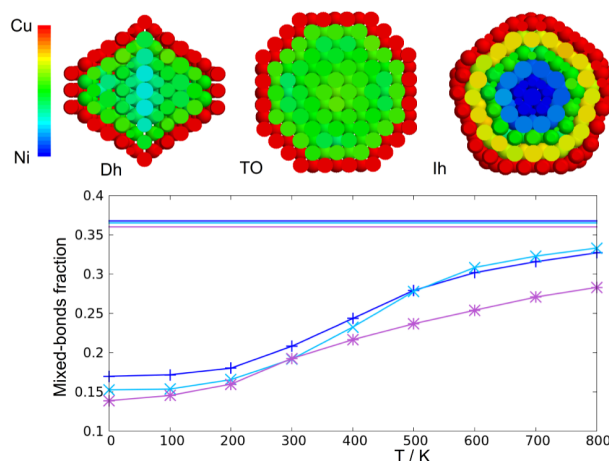
Fig. 7 a) Average local nickel occupations for Dh, Ih and TO clusters at 25% Ni composition at 600 K. b) Percentage of heterogeneous bonds for the same clusters as a function of temperature: Dh (+), TO (×) and Ih (*) clusters.
