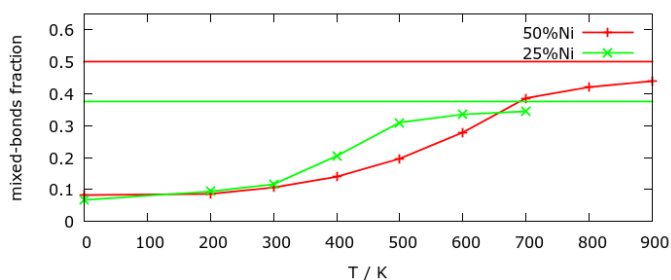
Fig. 3 Percentage of mixed-bonds in bulk at 25% and 50% Ni concentration as a function of the temperature. For each concentration the value for complete random mixing is shown.
