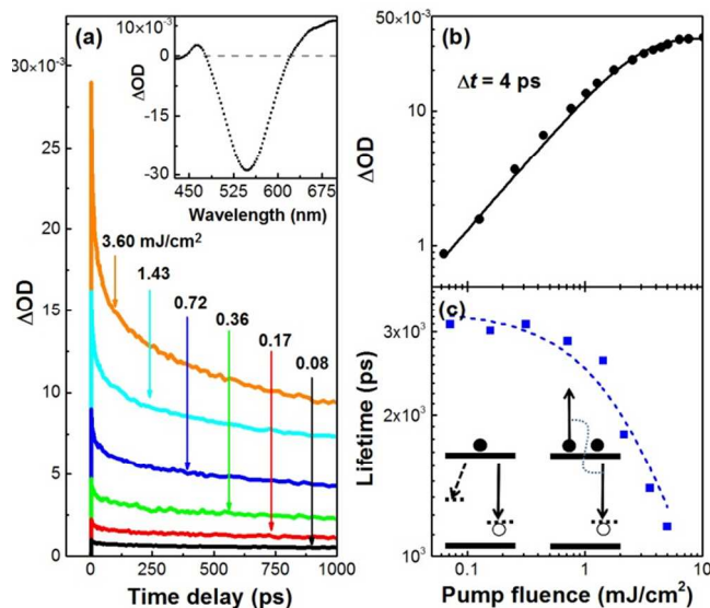
Fig. 3 (a) TA kinetics of 2.5 nm CIS QDs under different excitation densities and the inset shows the TA spectrum under the pump fluency of 3.6 mJ/cm 2 . Excitation power density dependence of (b) bleach amplitudes and (c) average life times probed at 1S transitions. The left scheme in figure (c) depicts the surface trapping and free-to-bound recombination under low pump fluency. The right scheme in figure (c) depicts the trap-assisted Auger recombination under high pump fluency. The dashed line in (c) is the fit by Eq. (1).
