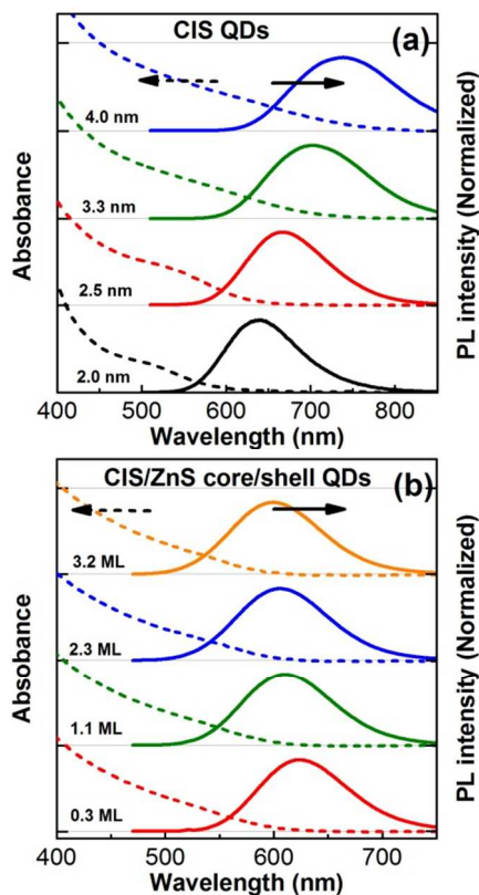
Fig. 1 Steady-state absorption (dashed lines) and PL spectra (solid lines) of (a) CIS QDs with four different sizes and (b) CIS/ZnS core/shell QDs with core diameter of 2.5 nm and four differently-thick ZnS shells.
