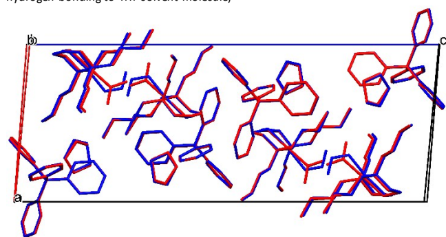
Figure 5. Overlay of unit cell packing diagrams for the GS (red) and MS (blue) of ( 1 ), showing subtle changes in the unit cell as a result of excitation at \lambda = 400 nm
