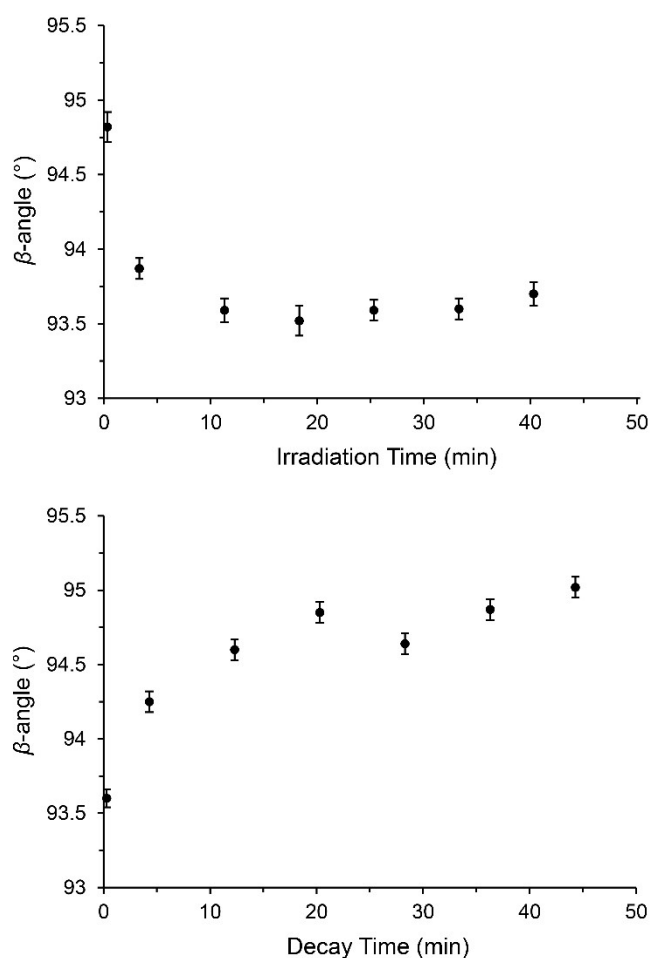
Figure 7. SC-XRD kinetics experiments at 240 K, following the change in \beta -angle as a result of nitrite linkage isomerism. Top: plot of \beta -angle vs. irradiation time under continuous illumination ( \lambda = 400 nm). Bottom: plot of \beta -angle vs. decay time in the dark
