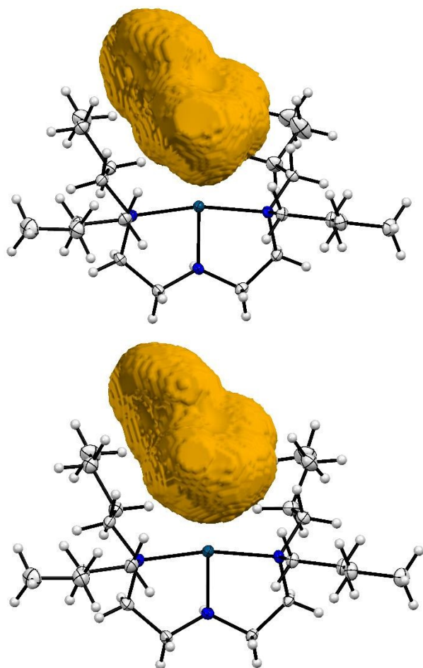
Figure 6. Reaction cavity volumes: top = GS cavity, bottom = MS cavity. Reaction cavity volumes are determined by removing the atoms of the nitrite ligand before conducting a contact surface void calculation in Mercury 35 (probe radius 1.2 Å, grid spacing 0.1 Å)
