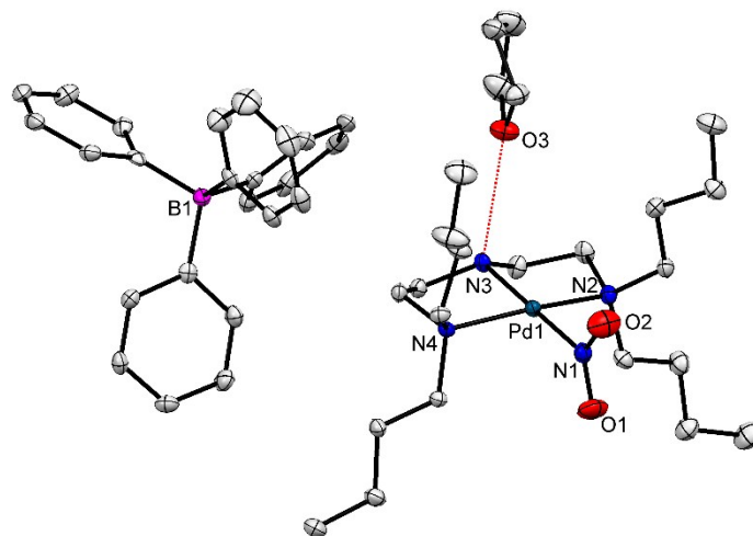
Figure 1. Single-crystal X-ray structure for the asymmetric unit of ( 1 ) showing the atomic arrangement in the ground state (GS), before any irradiation. Ellipsoids are set at 50% probability and hydrogen atoms are omitted for clarity (red dashed line = hydrogen bonding to THF solvent molecule)
