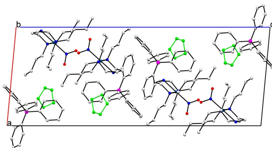
Figure 2. Crystal packing diagram (one unit cell) for the GS structure of (1) , before any irradiation. The packing diagram is viewed along the crystallographic b -axis, c -axis horizontal (hydrogen atoms omitted and THF solvent molecules highlighted in green for clarity)
