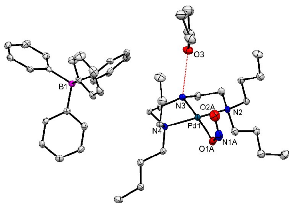
Figure 4. Single-crystal X-ray structure for the asymmetric unit of ( 1 ) showing the atomic arrangement in the metastable state (MS) after 1 h irradiation at \lambda = 400 nm. Ellipsoids set at 50% probability and hydrogen atoms omitted for clarity (red dashed line = hydrogen bonding to THF solvent molecule)
