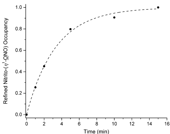
Figure 3. Plot of crystallographically-refined nitrito-( \eta^1 -QNO) occupancy vs. irradiation time (excitation at \lambda = 400 \text{ nm} ) for steady-state photocrystallographic experiments with (1) between 0 and 15 min illumination. JMAK kinetic analysis: k = 0.30(2) \text{ min}^{-1} , ( 0.0049(3) \text{ s}^{-1} ), n = 0.98(7) , R^2 = 0.99 .
