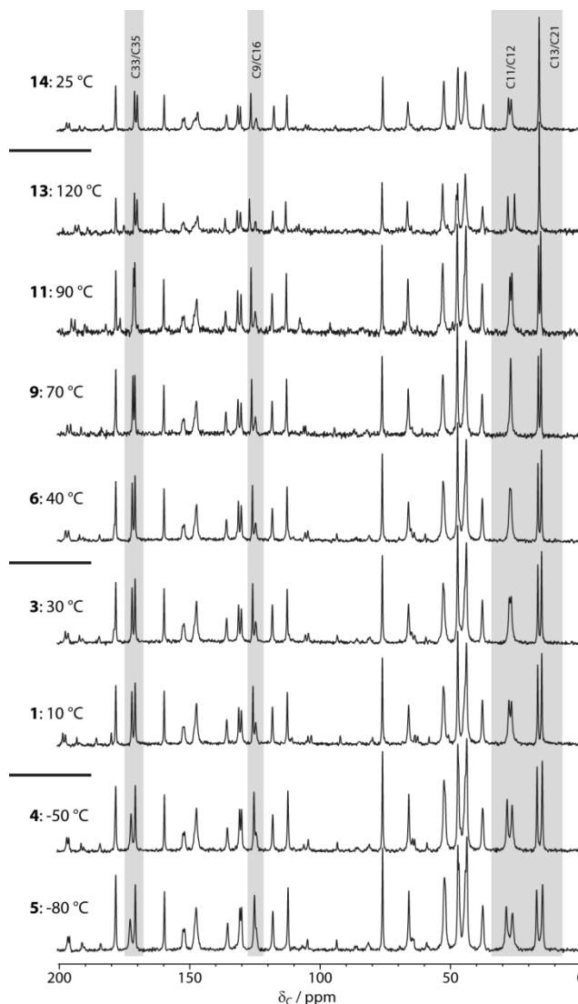
Figure 1. ^{13}\text{C} CPMAS spectra of initially hydrated sildenafil citrate as a function of temperature. Bold numbers indicate acquisition order, starting at 10 °C. Acquisition points 2 (20 °C), 7 (50 °C), 8 (60 °C), 10 (80 °C) and 12 (110 °C) are omitted for clarity. Shaded areas highlight spectral regions exhibiting the largest temperature dependence.
