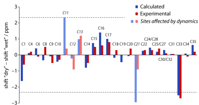
Figure 5. Calculated (blue) vs. experimentally observed (red) differences in ^{13}\text{C} chemical shift between dehydrated and hydrated sildenafil citrate. The shifts of overlapped peaks, where the assignment is ambiguous, have been averaged as indicated. Sites affected by dynamics are marked by paler colours and italic labels. Dotted lines indicated expected one-standard deviation variance expected if individual "errors" are uncorrelated.
