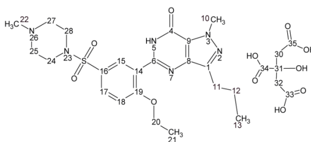
Scheme 1. Molecular schematic of sildenafil citrate, indicating the numbering of carbon and nitrogen atoms used in Ref. 4 and this work. Note that both molecules are shown, as conventionally represented, in their neutral forms, while XRD and NMR are consistent with a transfer of \text{H}^+ from the C34 carboxylic acid group to N26 in the solid state.
