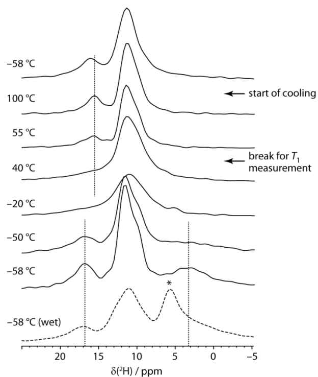
Figure 2. Centreband region of the direct-excitation ^2\text{H} MAS spectra of deuterated sildenafil citrate acquired as a function of temperature, starting at -58\text{ }^\circ\text{C} , heating to 100\text{ }^\circ\text{C} before cooling to the starting temperature. Several intermediate spectra (particularly on the cooling phase) are omitted as no significant changes were observed. Dotted lines mark characteristic signals as guides to the eye. The dashed line shows the spectrum of a new “wet” sample that shows additional intensity \sim 5 ppm (marked with *) assigned to adventitious water (see text).
