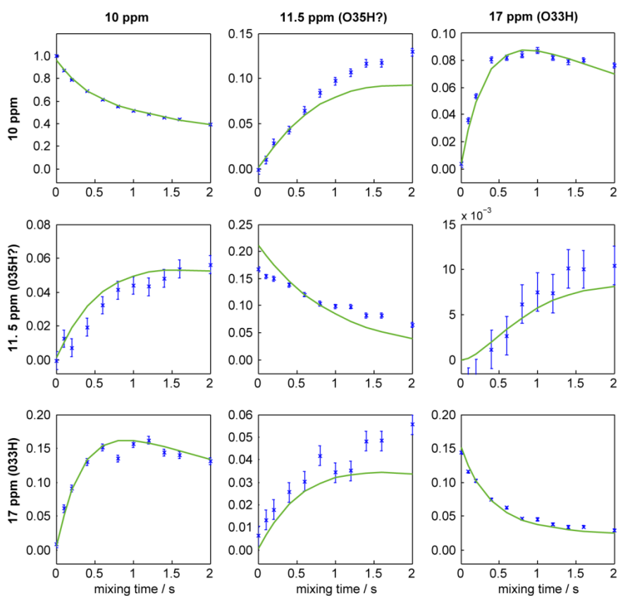
Figure 4. Intensities of cross-peaks in ^2\text{H} DQ/SQ EXSY spectrum and corresponding fits obtained on hydrated sildenafil citrate at -50\text{ }^\circ\text{C} . Columns correspond to frequencies in the direct (single-quantum) dimension, and rows to indirect dimension (double-quantum) frequencies. Error bars indicate one-standard deviation uncertainties on the intensity values. The corresponding figure for data acquired at -30\text{ }^\circ\text{C} can be found as Figure S3 of the Supporting Information.
