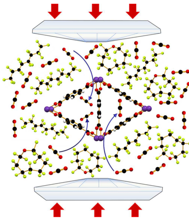
Figure 3. Cartoon schematic of pressure-induced \text{CO}_2 loading of porous \text{Sc}_2\text{BDC}_3 from liquid FC-77. Colour scheme as in Figure 1, with green spheres denoting F atoms. As pressure is applied to the \text{Sc}_2\text{BDC}_3 crystal in the sample chamber between two diamond culets, dissolved \text{CO}_2 in the liquid is squeezed into the previously empty framework. The molecules of the FC-77 are too large to penetrate the framework.
