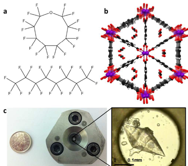
Figure 1. Materials used to perform high-pressure, single-crystal X-ray diffraction experiments. a , structure of Fluorinert™ FC-77; a mixed liquid consisting of perfluorooctane ( C_8F_{18} ) and perfluorooxacyclononane ( C_8F_{16}O ). b , six-channel portion of the previously-determined monoclinic Sc_2BDC_3 crystal structure 12 , shown with partially-occupied adsorbed CO_2 molecules in the framework pores. Purple, black, red and white spheres denote Sc, C, O and H atoms respectively. c , photograph of a modified Merrill-Bassett diamond anvil cell (DAC) (depicted beside a five-pence coin for scale), with an expanded photomicrograph of the sample chamber containing a single crystal of Sc_2BDC_3 surrounded by CO_2 -loaded FC-77 liquid.
