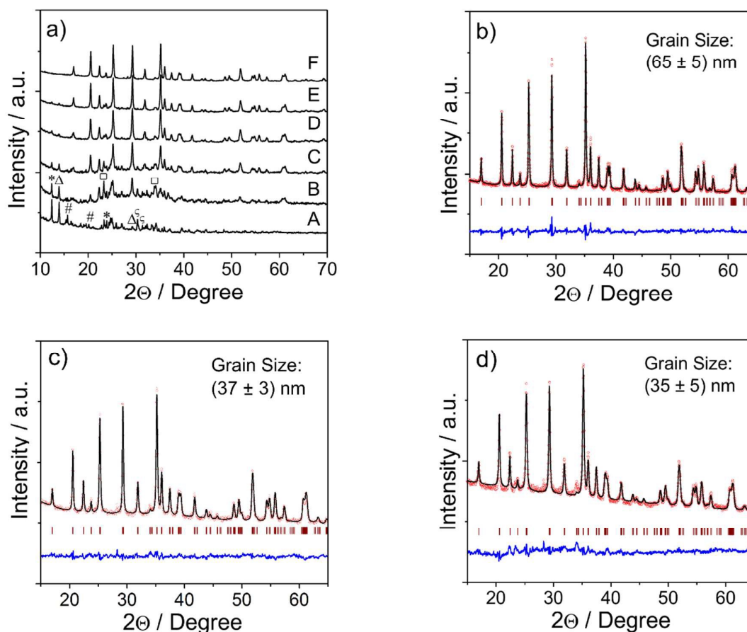
Fig. 1 (a) XRD patterns (undiluted approach with 60 mmol L -1 precursor concentration) recorded after reaction times of 0 min (A), 3 min (B), 5 min (C), 7 min (D), 9 min (E) and 11 min (F), respectively. (b) Refined diffraction pattern of (F). (c) Refined diffraction pattern of LiMnPO 4 after a reaction time of 15 min and two-fold dilution of the LiMnPO 4 precursors (30 mmol L -1 precursor concentration) (d) Refined diffraction pattern of LiMnPO 4 after a reaction time of 21 min and three-fold dilution of the LiMnPO 4 precursors (20 mmol L -1 precursor concentration). Observed intermediate phases are indicated by different symbols: # (MnCl 2 ·2H 2 O; ICSD code 15596), □ (Li 3 PO 4 ; ICSD code 77095), * (Mn(P 4 O 11 ); ICSD code 400840), Δ (Mn 2 (P 4 O 12 ); ICSD code 412558), ζ Mn 6 (PO 4 ) 4 ·1H 2 O; ICSD code 412152).
