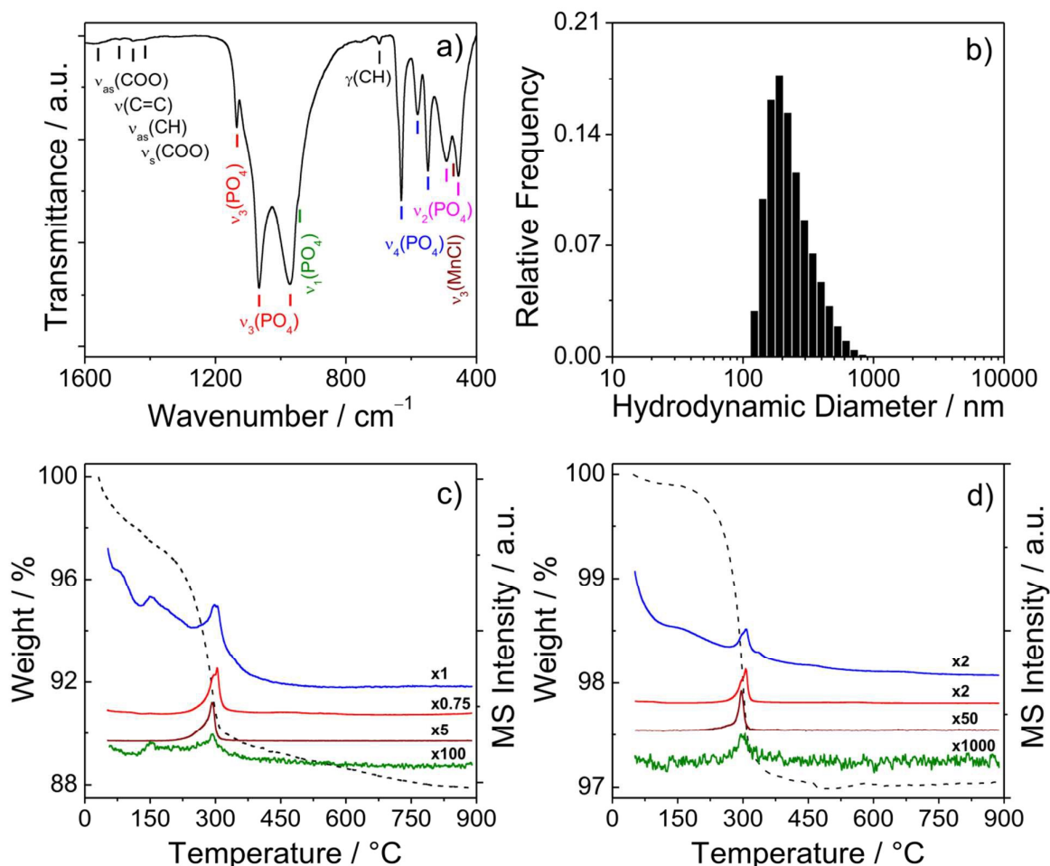
Fig. 4 Results of different analytical investigations of LiMnPO 4 samples with grain sizes of approx. 37 nm (batch size 30 mmol L -1 ; 15 min synthesis time). (a) Representative ATR-FTIR absorption spectrum. (b) Particle size distribution obtained by dynamic light scattering experiments of LiMnPO 4 after redispersion in pure ethanol. The average hydrodynamic diameter is 200 nm. (c) TGA-MS data measured in synthetic air employing a heating rate of 5 °C. The dashed line represents the TG curve. The MS analysis shows H 2 O ( m/e = 18) in blue, CO 2 ( m/e = 44) in red, acetyl ( m/e = 43) in brown and Cl ( m/e = 37) in green. (d) TGA-MS results for the undiluted approach (batch size 60 mmol L -1 ) are also shown for purposes of comparison.
