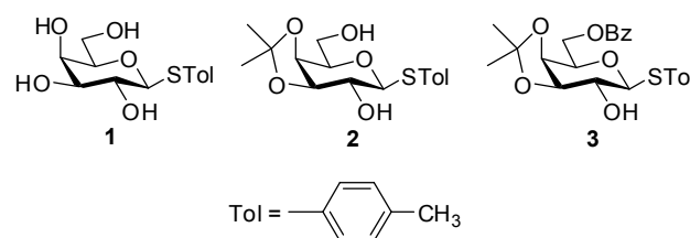
Figure 1: Structures of the derivatives in this study
