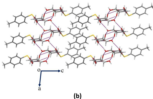
Figure 6 (a) ORTEP representation of the crystal of compound 1 with thermal ellipsoids drawn at the 50% probability level (b) Molecular packing showing 2D HBN in the crystal structure. Notice the formation of double sided comb-like sheets via strong intermolecular O–H...O hydrogen bonds and interlocked by p -thiotolyl groups
