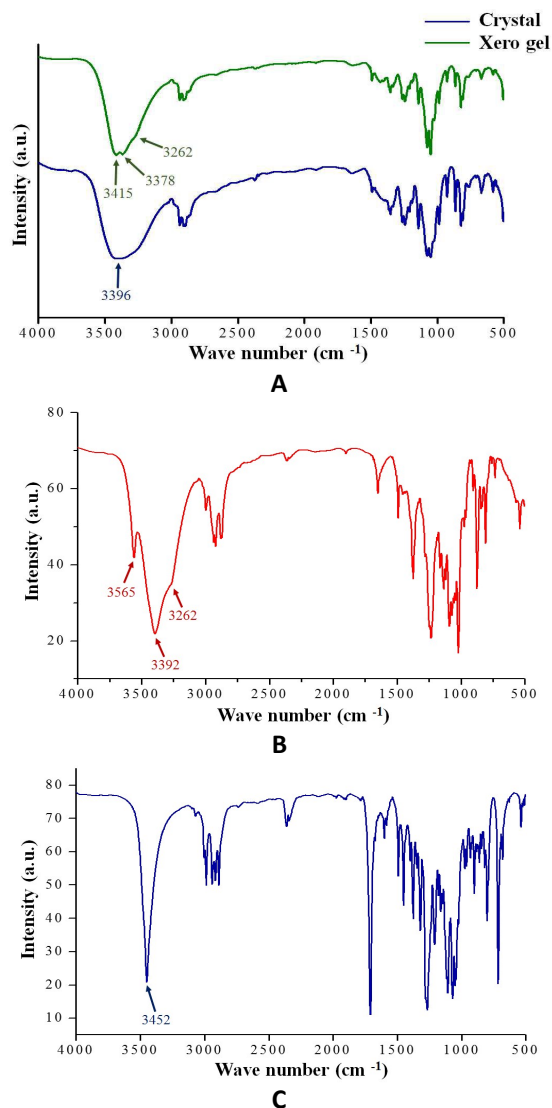
Figure 3 (A) FT-IR spectra of compound 1 in crystalline and xerogel state (0.25% w/v in 1,3-dichlorobenzene); (B) compound 2 in crystalline state and (C) compound 3 in crystalline state
