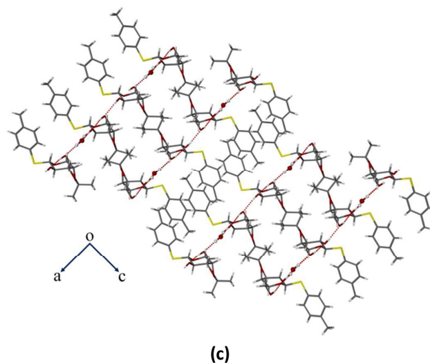
Figure 7 (a) ORTEP representation of the crystal of compound 2 with thermal ellipsoids drawn at the 50% probability level (b) Molecular packing showing 2D HBN involving sugar-sugar and sugar-water interactions in the crystal structure (except the hydroxyl H, all other H have been omitted for clarity). (c) The ladder motif along the b -axis. Notice the formation of double sided comb-like sheets via strong intermolecular O–H...O hydrogen bonds and interlocked by p -thiotolyl groups
