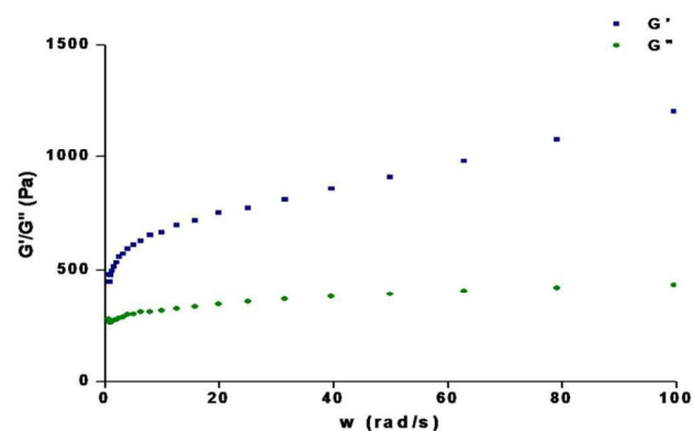
Figure 5 Dynamic rheology of the organogel containing 1.2% w/v compound 1 in 1,3-dichlorobenzene as a function of angular frequency ( \text{rad s}^{-1} ) at 15 °C.
