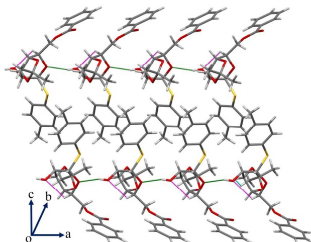
Figure 9 In addition to the strong O-H...O interaction significant intramolecular C-H...O HBN shown in the packing of compound 3 along the given axis
