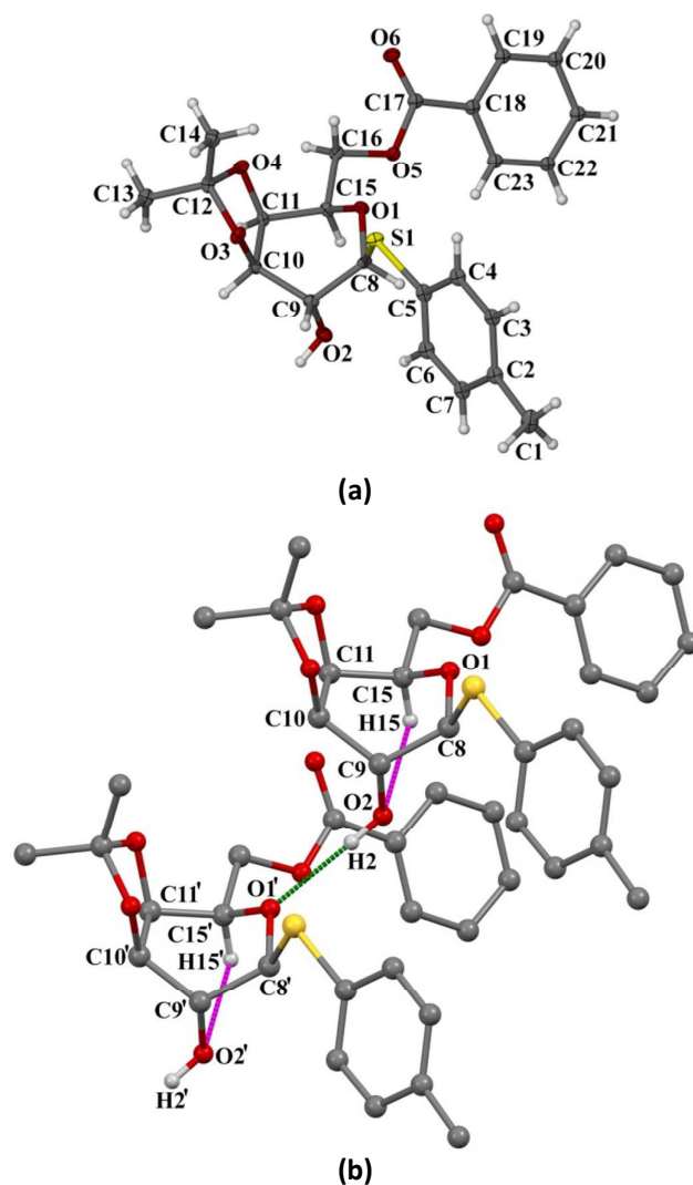
Figure 8 (a) ORTEP representation of the crystal of compound 3 with thermal ellipsoids drawn at the 50% probability level (b) HBN involved for the change of conformation in the pyranose ring (except the hydroxyl H, all other H have been omitted for clarity). Two discrete molecules are shown in ball and stick model to illustrate the HBN responsible for conformational change.
