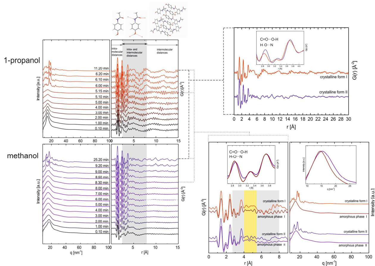
Figure 3. Time-resolved crystallization process of monoclinic form I (top left) from 1-propanol and orthorhombic form II (bottom left) from methanol are analyzed by high energy synchrotron X-ray to gain high q -range data. The PDFs of crystalline products are compared and structural characteristics are highlighted in the enlargement (top right). The graphic below left displays the PDFs of amorphous phases shortly before crystallization starts compared with the PDFs of the corresponding crystalline forms. The inset shows a characteristic range from 2.65 to 4.0 Å. To the right, there are the corresponding X-ray patterns of the amorphous and crystalline phases. The inset highlights the scattering shift of the two different amorphous phases.
