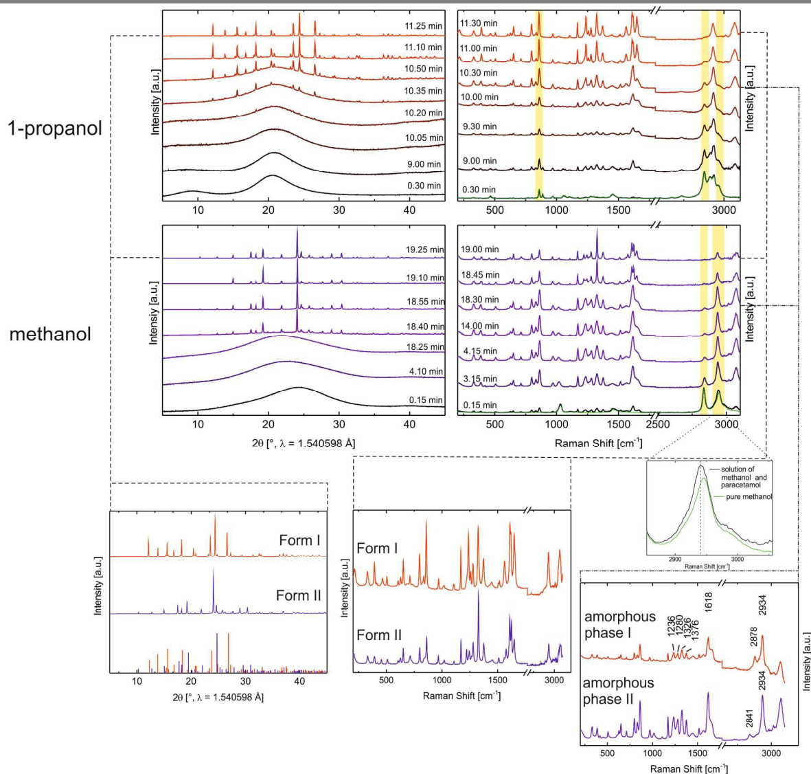
Figure 2. The Crystallization process of form I (top) and form II (middle) detected by combined in situ synchrotron XRD (top and middle left) and Raman spectroscopy (top and middle right). The X-ray patterns of the crystallized polymorphs are compared with the data entries HXACAN27 (form I) and HXACAN31 (form II) of the CSD (bottom left). The Raman spectra of the amorphous phases (bottom right) and final products (bottom middle) during the crystallization to form I and form II are presented. The enlargement of the vibration signal of the methyl group in methanol solution is shown in the range of 2850–3060 \text{cm}^{-1} (bottom right).
