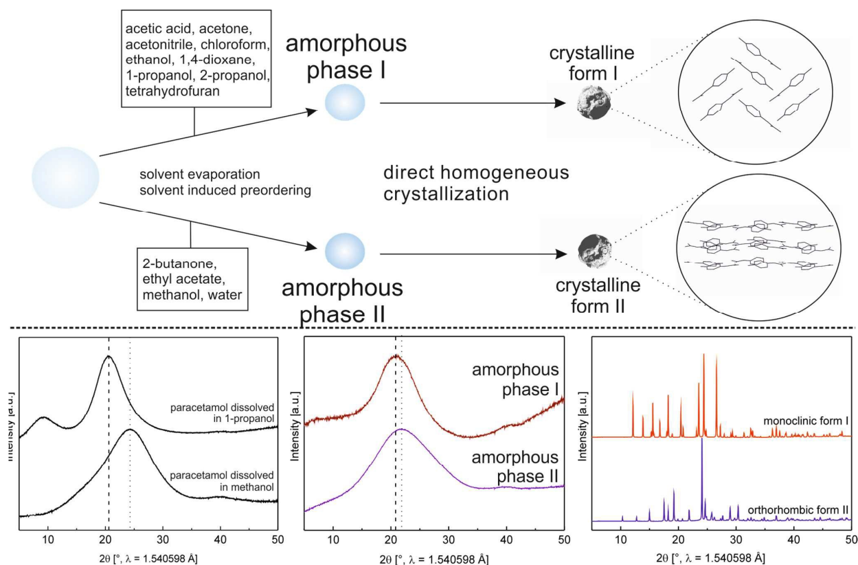
Figure 4. Top: Overview of the crystallization of paracetamol from solution in different solvents and amorphous precursors during the crystallization of form I and form II. Bottom: Corresponding X-ray patterns of the different stages.
