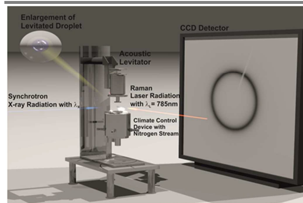
Figure 1. Experimental setup with the acoustic levitator and climatic chamber for the control of crystallization conditions. A) Setup for the crystallization investigation with simultaneously recorded synchrotron X-ray pattern ( \lambda_x=1 \text{ \AA}=0.1 \text{ nm} ) and Raman spectra ( \lambda_l=785 \text{ nm} ). B) Similar setup for the pair distribution function analysis with synchrotron X-ray radiation ( \lambda_x=0.158 \text{ \AA}=0.0158 \text{ nm} ). Raman spectra were not measured.
