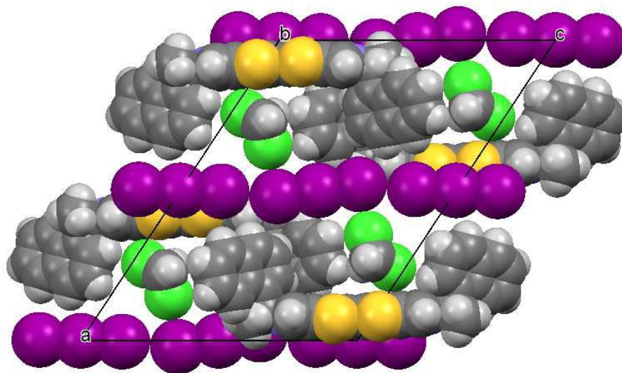
Figure 8. Crystal packing of 12 \cdot I_3 \cdot CH_2Cl_2 viewed down the b axis with one orientation for the triiodide and associated dichloromethane molecule,
