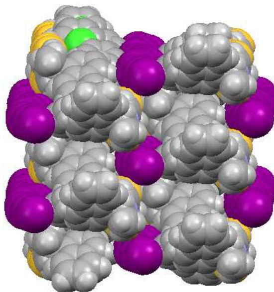
Figure 7. Crystal packing in 12 \cdot \text{I}_3 \cdot \text{chlorobenzene} viewed on the bc plane (above) and viewed along the c axis (below).
