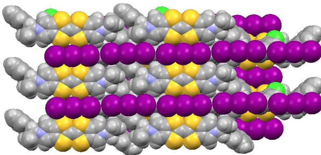
Figure 6. View of the structure of \mathbf{12} \cdot \text{I}_3 \cdot \text{chlorobenzene} , showing how the solvent molecules lie close to the interface between triiodide ions.
