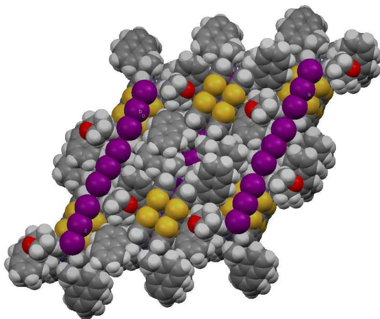
Figure 4: (a) Section of crystal packing in 12 ·I 3 ·THF showing the conformation of the donor and the relative location of the lines of triiodides and the THF molecules, (b) view of crystal packing looking down the b axis.
