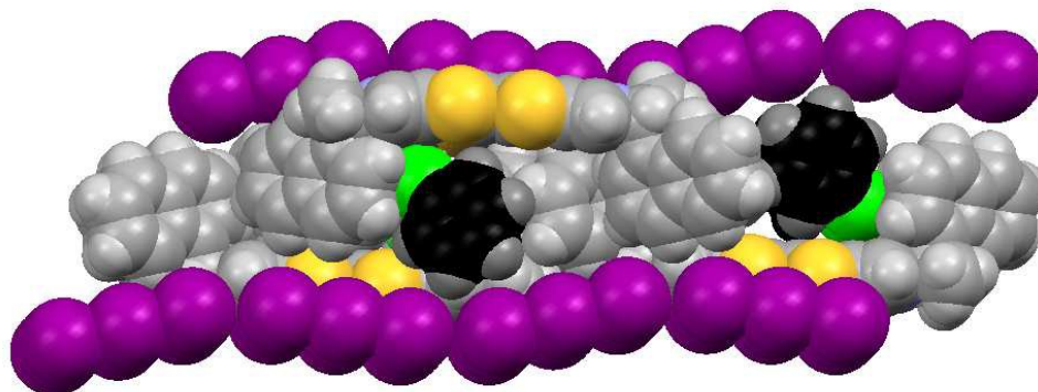
Figure 6. View of the structure of \mathbf{12} \cdot \text{I}_3 \cdot \text{chlorobenzene} , showing how the solvent molecules lie close to the interface between triiodide ions.
