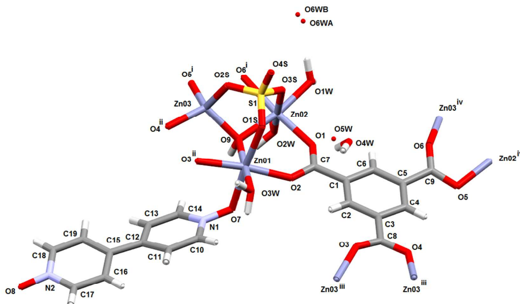
Figure 1. Basic chemical unit of the 104 K structure of 1 showing the coordination environment of the 3 unique Zn(II) ions. i 1+y-x, 1-x, z, ii 1-y, 1+x-y, z, iii y-x, 1-x, z, iv 1-y, x-y, z
