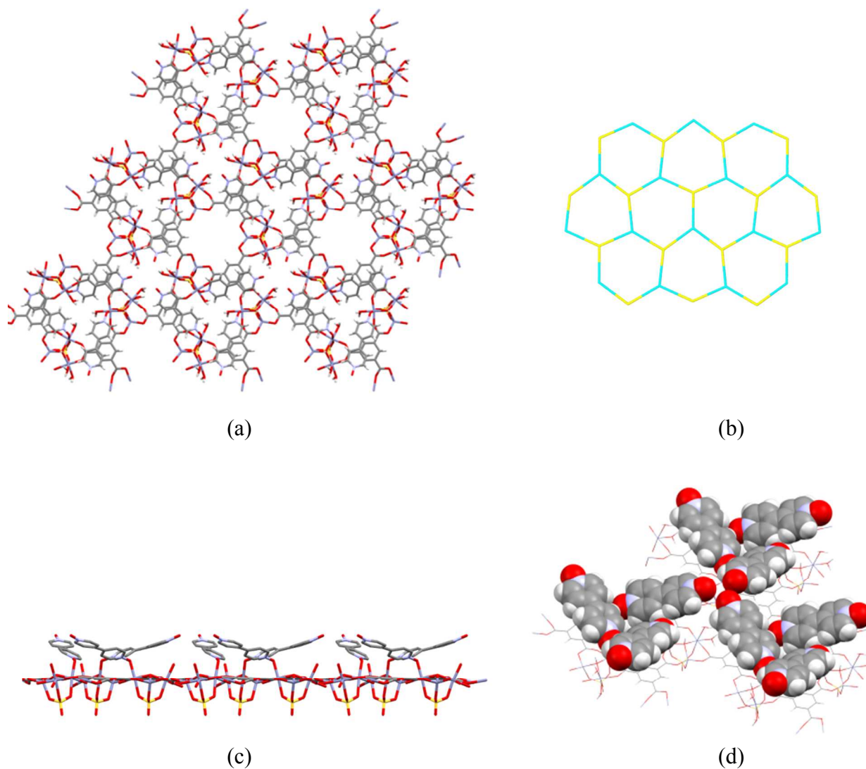
Figure 2. (a) top view of the 2D layer (b) honeycomb motif taking the nodes at the centres of the metal cluster (in blue) and the trimesate ligand (yellow), respectively (c) side view of 2D layer showing the sulfate groups on one side of the layer and the 4,4'-bpdo molecules on the other and (c) oblique view of the 2D layer showing the 'flat' bowl formed by three trigonally arranged 4,4'-bpdo molecules
