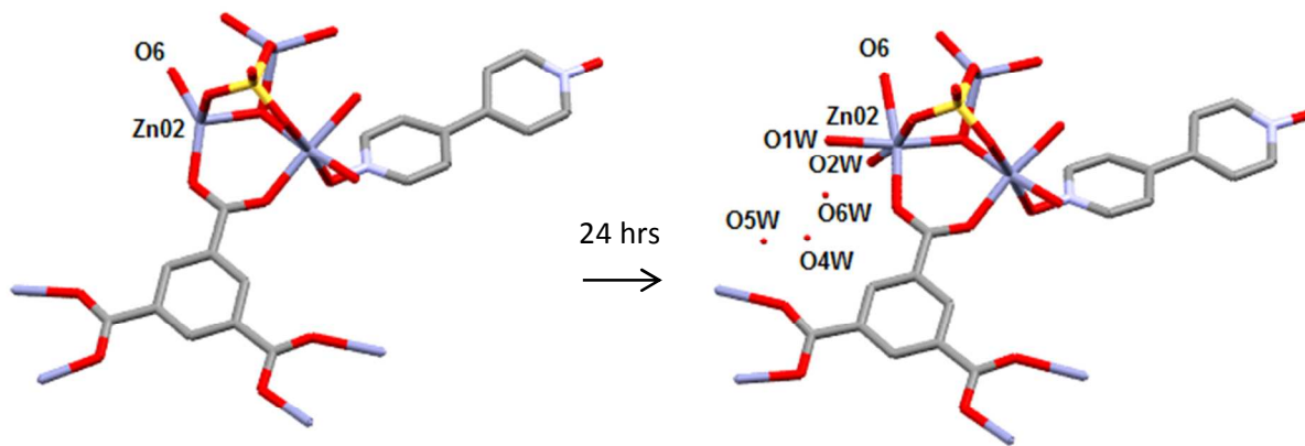
Figure 8. (a) structure of 1 after a single crystal was heated to 373 K and cooled to 298 K (b) subsequent structure of 1 after the single crystal was left on diffractometer for 24 hours without the the flow of dry air over the crystal
