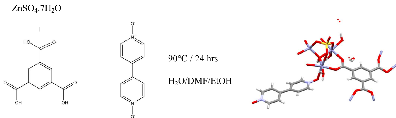
Scheme 1 Preparation of 1
