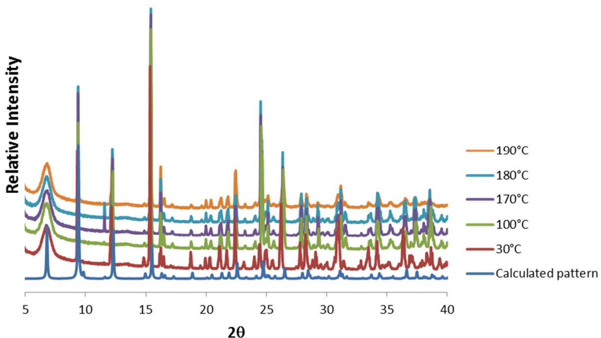
Figure 5 PXRD patterns in the range 30-190°C compared with the calculated pattern of 1 at 298 K.
