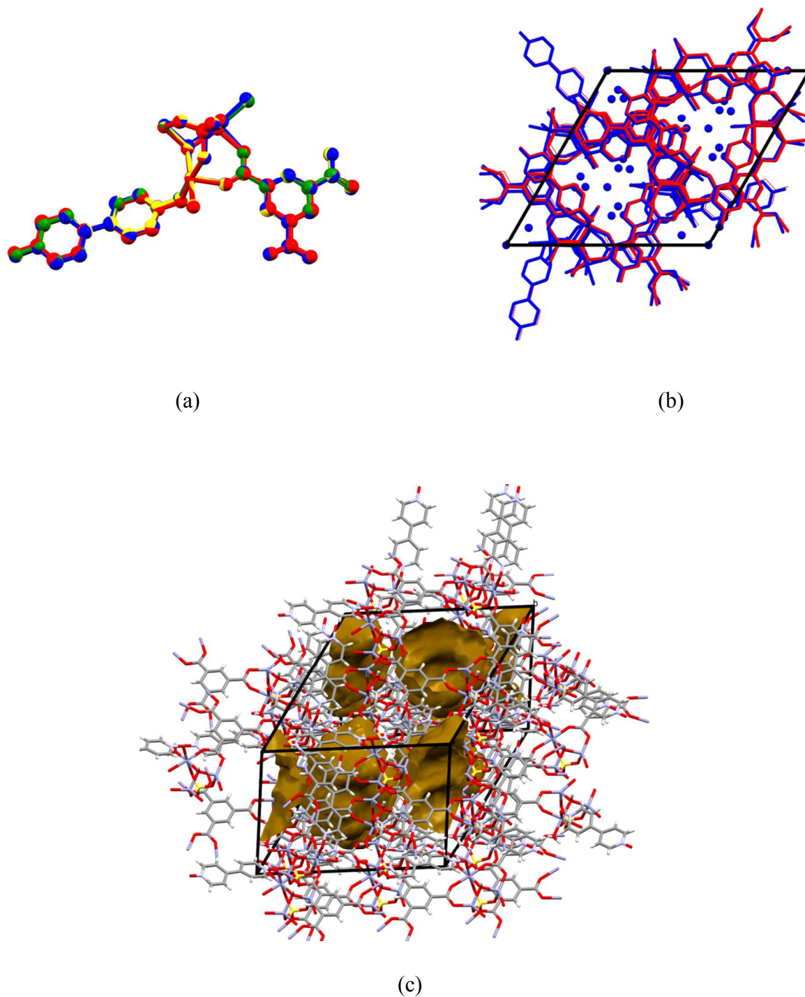
Figure 4. (a) Overlay of the 104 K (blue), 298 K (yellow), 323 K (green) and 373 K (red) chemical units as displayed by Mercury. (b) Overlay of packing of the 104 K structure (blue) and the 373 K structure (red) (water molecules present in the 104 K structure but not present in the 373 K structure are shown as blue spheres) and (c) oblique angle of crystal packing showing isolated voids in the 373 K structure
