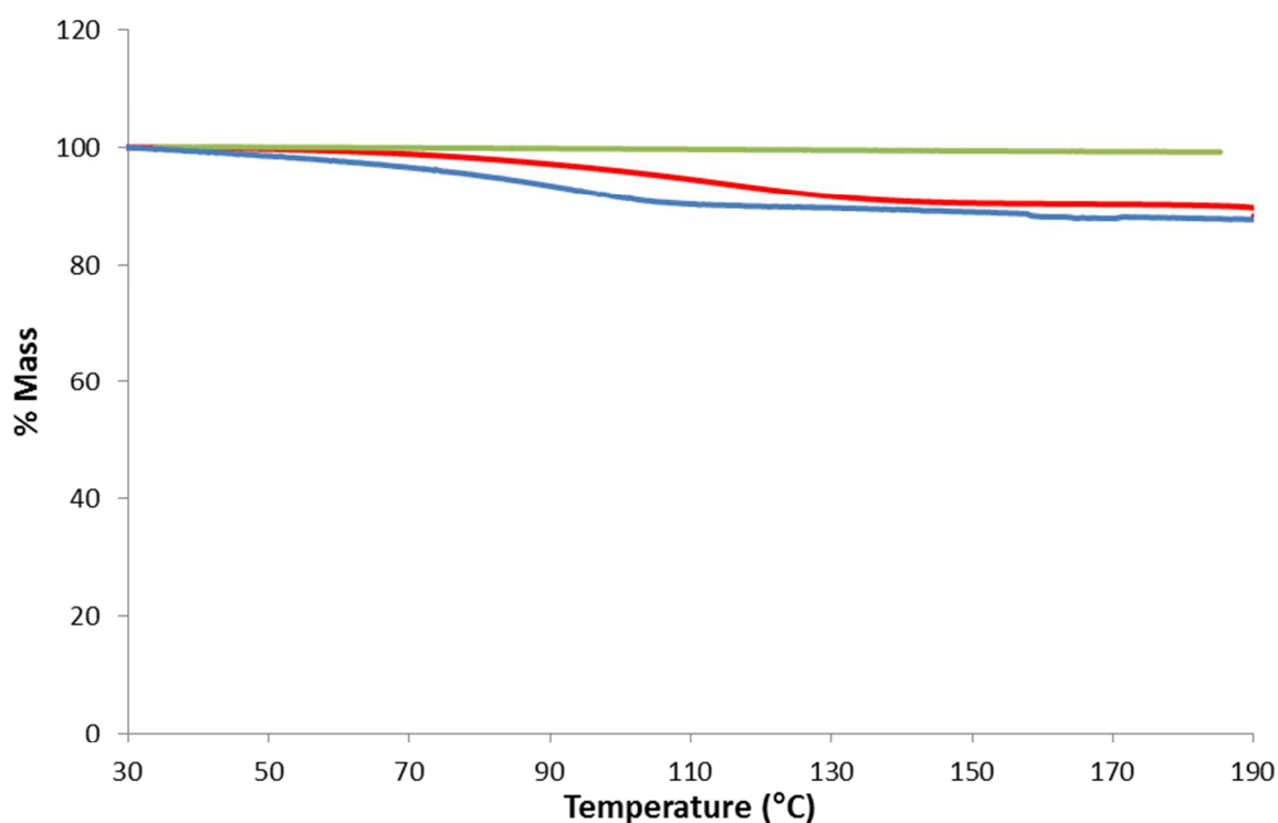
Figure 7. TGA thermograms of 1 for the as-synthesized MOF (red), the immediate reheat (green) and after 24 hours of being exposed to a humid atmosphere (blue)
