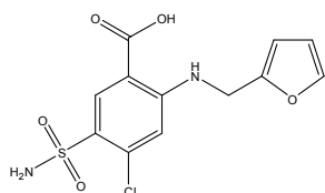
Figure 1 The molecular structure of furosemide
