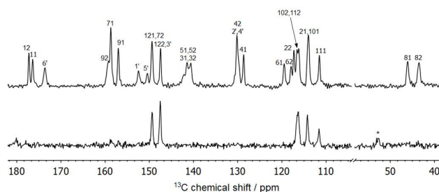
Figure 4 ^{13}\text{C} CPTOSS spectrum (top) and direct-excitation spectrum (bottom) of 2FS-INA at 8 kHz MAS with carbon atoms labelled as in Fig. 3
