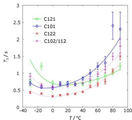
Figure 8 The temperature dependence of the ^{13}\text{C} T_1 relaxation times for the furan rings on FS1 and FS2. Temperatures include a correction of +10 °C for sample heating due to MAS.
