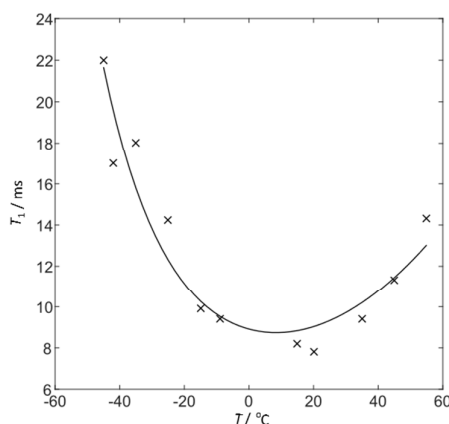
Figure 7 Sulphonamide ^2\text{H} T_1 relaxation time constant as a function of temperature fit to a two-site jump model with an Arrhenius-type temperature dependence of the jump rate. Temperatures include a correction of +15 °C for sample heating due to MAS.
