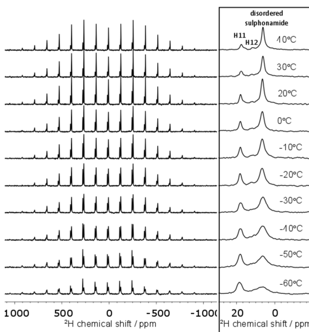
Figure 6 Variable temperature ^2\text{H} spectra at 10 kHz MAS. The centre-band of each spectrum is shown on the right. Baselines were corrected for this figure using the Whittaker Smoother in MestReNova
