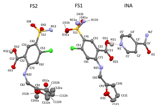
Figure 3 The asymmetric unit of 2FS-INA with the major occupied furan ring and sulphonamide positions drawn as free atoms. The SSHB is shown by the dashed red line and with hydrogen atoms are removed for clarity except for those on the carboxylic acids. Thermal ellipsoids are shown at the 50 % probability level. FS site numbering follows that of Ref. 13 with labels followed by 1 or 2 to distinguish FS1 and FS2. A trailing apostrophe identifies INA sites.
