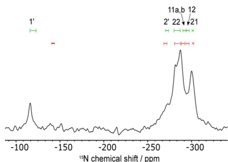
Figure 5 ^{15}\text{N} spectrum of 2FS-INA at 8 kHz MAS. Overlaid are the calculated ^{15}\text{N} shieldings for H11 associated with FS1 (green, top) and transfer of H11 to INA (red, bottom) where the length of the line represents the spread of calculated chemical shifts for the different disorder structures
