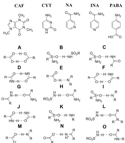
Figure 2 The cofomers in structurally characterised FS cocrystals and the synthons present in FS cocrystals
