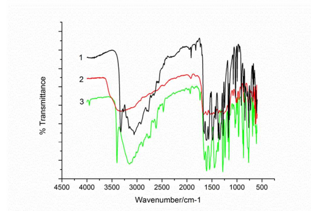
Figure 7: Infra-red spectra showing the initial transformation from Form I (1) to Form II (3), through an intermediate melt stage (2), at which the characteristic N-H stretching mode disappeared. Plots are staggered along the y-axis for clarity.
