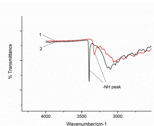
Figure 6: a) IR spectra for Form I (1) and Form II (2); b) Expanded region showing the difference in N-H stretching modes between the two forms.
