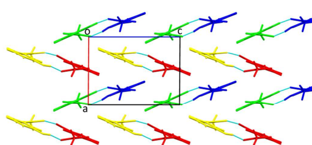
Fig.4. a) Representation of structural motifs in the structure of metacetamol II along a axis, b) along b axis. Hydrogen bonds are shown by dashed lines.
