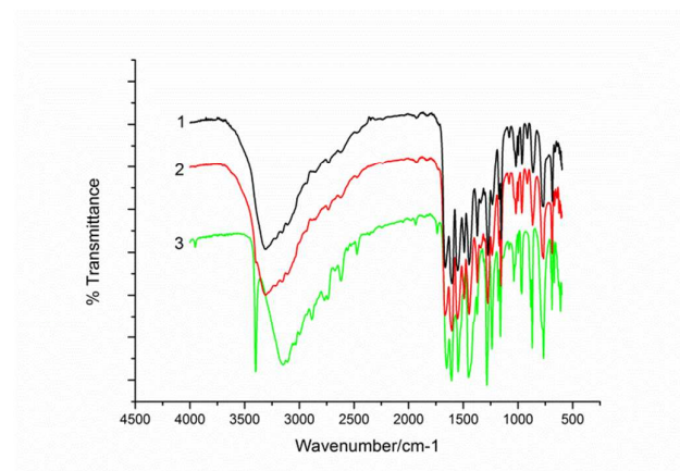
Figure 8: IR-spectra, giving evidence of a slow transformation from an amorphous phase (1, 2) to Form II (3), seen over several hours, identified by the -NH peak which begins to form at \sim 3400\text{cm}^{-1} . Plots are staggered along the y-axis for clarity.
