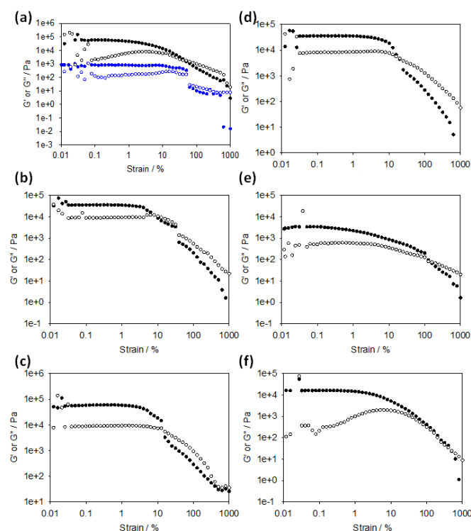
Figure 3. Strain sweeps for gels formed from (a) FmocF; (b) FmocY; (c) FmocW; (d) FmocM; (e) FmocG; (f) FmocI. In all cases, a concentration of Fmoc-amino acid of 10 mg/mL was used and the samples shown are with a GdL concentration of 5 mg/mL. In (a), a gel formed using a GdL concentration of 1 mg/mL is used (blue data). In all cases, the closed symbols represent G' , the open symbols G'' .
