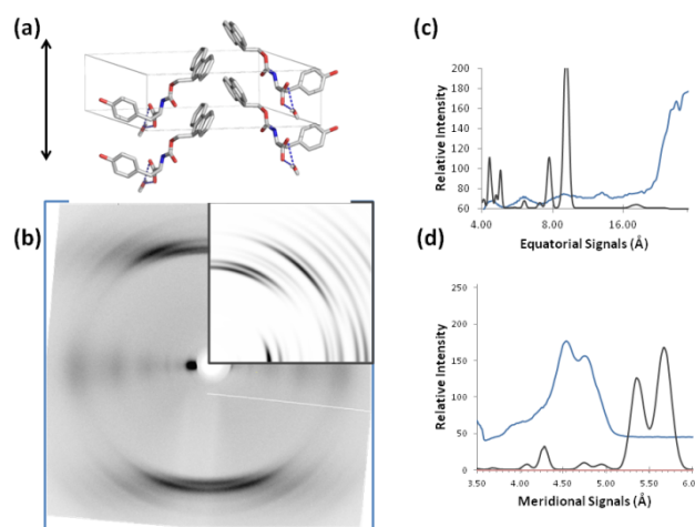
Figure 12. a) The X-ray crystal structure of FmocY oriented to align to a possible fibre axis (denoted by black double head arrow). b) Comparison between calculated (insert) and experimental diffraction data for FmocY. The red arrows denote signals in agreement between experimental and calculated data. c) Graphical trace comparing equatorial signals for calculated (black) and experimental data (blue). d) Graphical trace comparing meridional signals for calculated (black) and experimental data (blue).
