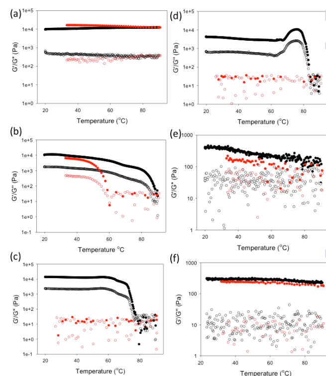
Figure 4. Temperature sweeps for gels formed from (a) FmocF; (b) FmocY; (c) FmocW; (d) FmocM; (e) FmocG; (f) FmocI. In all cases, a concentration of Fmoc-amino acid of 10 mg/mL was used and the samples shown are with a GdL concentration of 5 mg/mL. In all cases, the black data shows the heating cycle (at a rate of 2 °C/min and the red data shows the cooling cycle at a rate of 5 °C/min). The closed symbols represent G' , the open symbols G'' .
