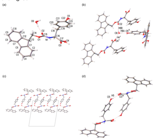
Figure 9. (a) Displacement ellipsoid plot of the asymmetric unit from the single crystal structure FmocY·H 2 O, ellipsoids displayed at 50% probability level. (b) Hydrogen bonded interaction evident between H 2 O and three distinct FmocY molecules. (c) Extension of the hydrogen bonded network of FmocY molecules via H 2 O along crystallographic a axis. (d) Intermolecular hydrogen bonding interactions between two FmocY molecules. Symmetry elements, i: (-1/2+x, 1/2+y, +z), ii: (1/2-x, -1/2+y, -z), iii: (1-x, 1+y, -z).
