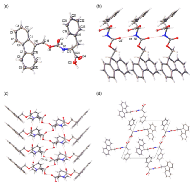
Figure 7. (a) Labeled displacement ellipsoid plot of the asymmetric unit from the single crystal structure of FmocF, ellipsoids displayed at 50% probability level. (b) Intermolecular hydrogen bonding of FmocF molecules via N1-H1\cdots O2 , perspective view [001]. (c) Intermolecular hydrogen bonding of FmocF molecules via carboxylic acid groups, perspective view [101]. (d) Extended crystal packing of FmocF molecules, perspective view [010], unit cell shown. Symmetry element, i: (x, y-1, z) , ii: (-x, -1/2+y, 1-z) .
