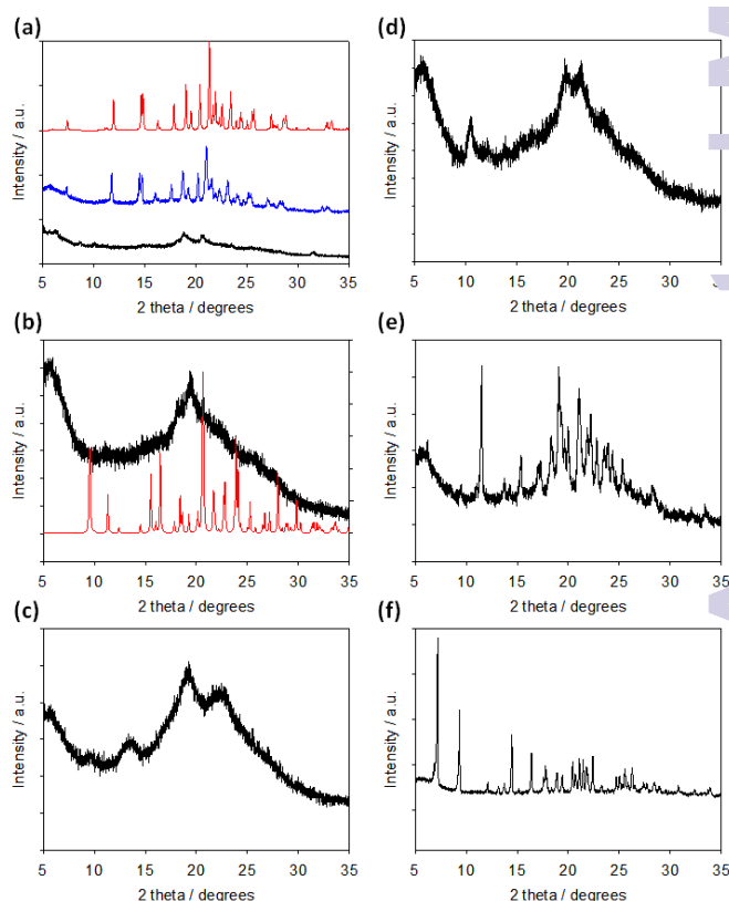
Figure 6. pXRD data for xerogels prepared by air-drying gels formed from (a) FmocF; (b) FmocY; (c) FmocW; (d) FmocM; (e) FmocG; (f) FmocI. In all cases a concentration of Fmoc-amino acid of 10 mg/mL was used and the samples shown are with a GdL concentration (for (b) – (f)) of 5 mg/mL. In (a), data for a gel formed using a GdL concentration of 1 mg/mL (black data) and 5 mg/mL (blue data) are shown. Gels were air-dried 24 hours after addition of GdL. For (a) and (b), the red data is the predicted data calculated from the single crystal structures (see below).
