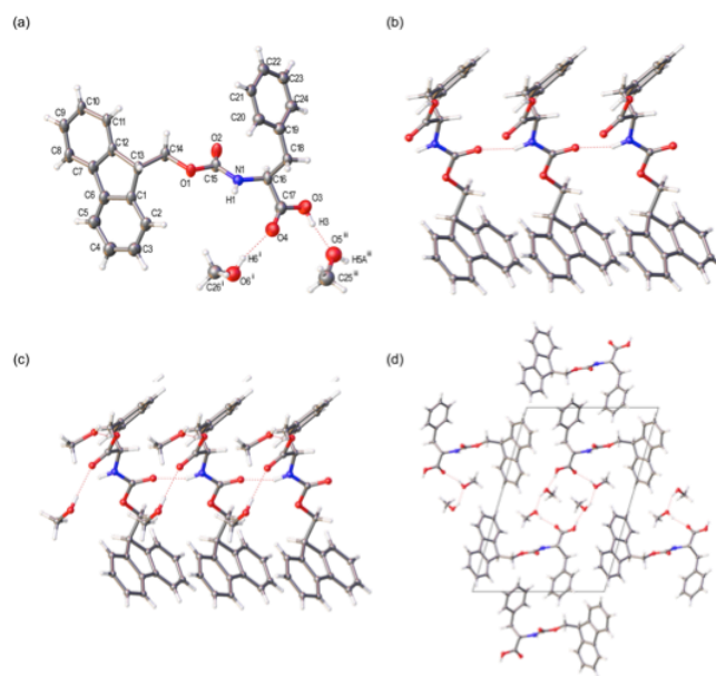
Figure 8. (a) Labeled displacement ellipsoid plot of the asymmetric unit from the single crystal structure of FmocF\cdot(MeOH)_2 , ellipsoids displayed at 50% probability level, hydrogen bonded interactions to MeOH shown. (b) Intermolecular hydrogen bonding of FmocF molecules via N1-H1\cdots O2 . (c) Hydrogen bonding interaction between FmocF carboxylic acid terminus and MeOH. (d) Extended crystal packing of FmocF molecules, perspective view [010], unit cell shown. Symmetry operations, i: (x, -1+y, z) , ii: (1-x, -1/2+y, 1-z) .
