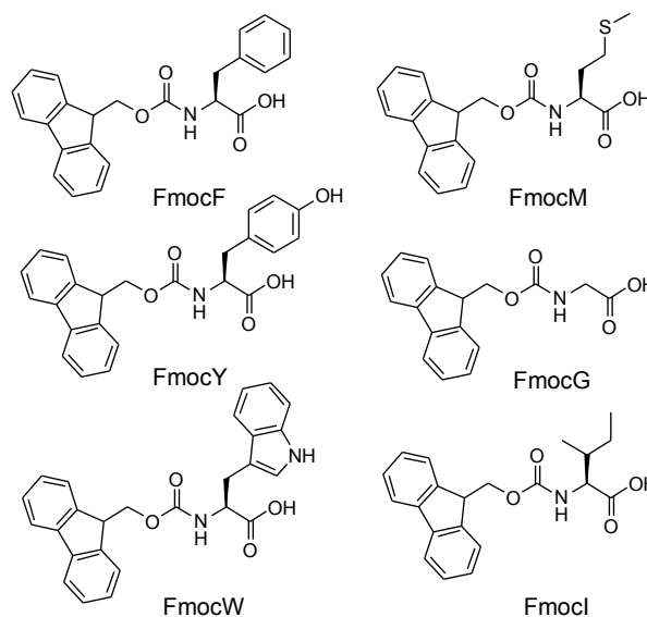
Figure 1. Structures of the Fmoc amino acid LMWG.
