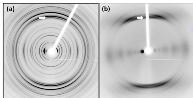
Figure 10. X-ray fibre diffraction patterns from partially aligned hydrogels formed by a) FmocF and b) FmocY. The X-ray fibre axis is vertical and the major meridional reflections are highlighted by the white arrows. Diffraction positions are shown in Table 4.
