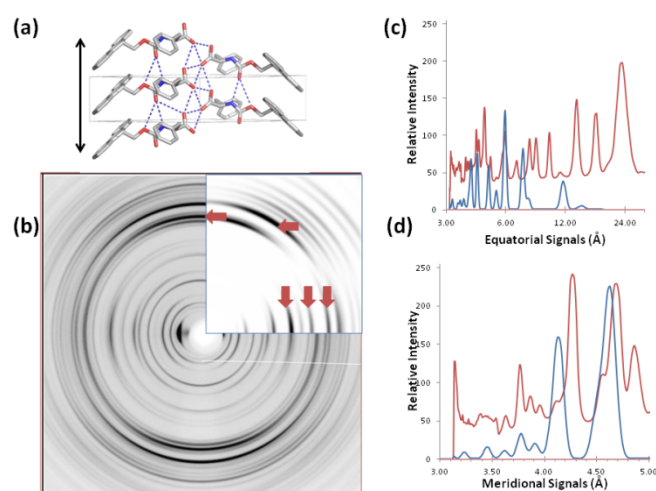
Figure 11. a) The X-ray crystal structure of FmocF oriented to align the hydrogen bonding direction with a possible fibre axis (denoted by black double head arrow). b) Comparison between calculated (insert) and experimental diffraction data for FmocF. The red arrows denote signals in agreement between experimental and calculated data. c) Graphical trace comparing equatorial signals for calculated (blue) and experimental data (red). d) Graphical trace comparing meridional signals for calculated (blue) and experimental data (red).
